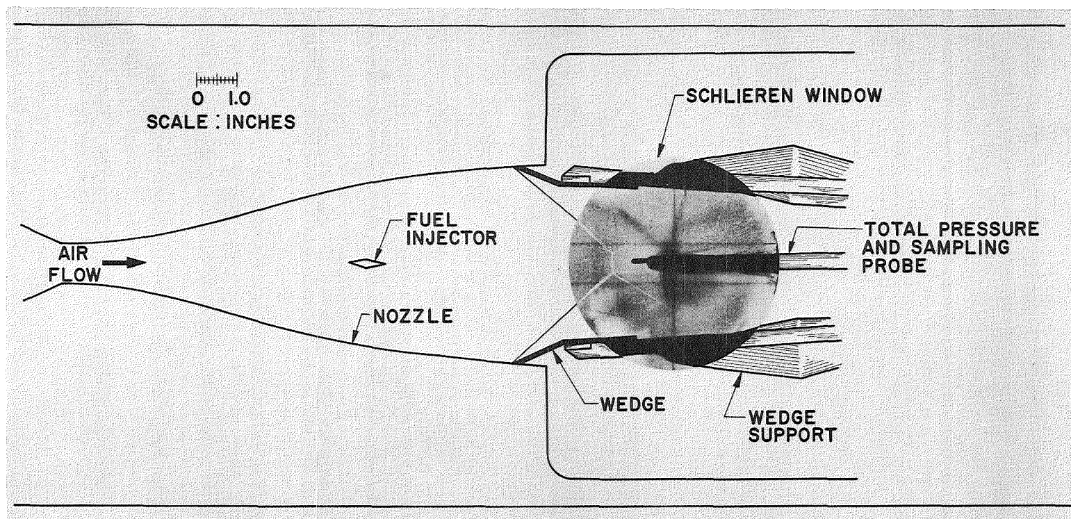
Fig. 2 Schematic of Nozzle and Test Section Showing Normal Shock Configuration with Schlieren Photo of Shock System
