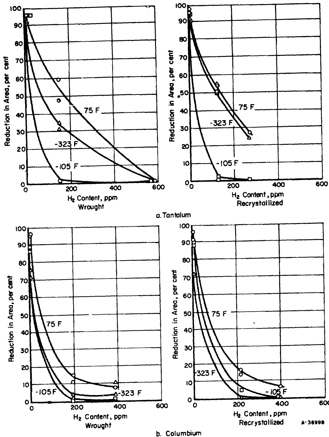
FIGURE 15. EFFECT OF HYDROGEN CONTENT ON THE DUCTILITY OF TANTALUM AND COLUMBIUM
