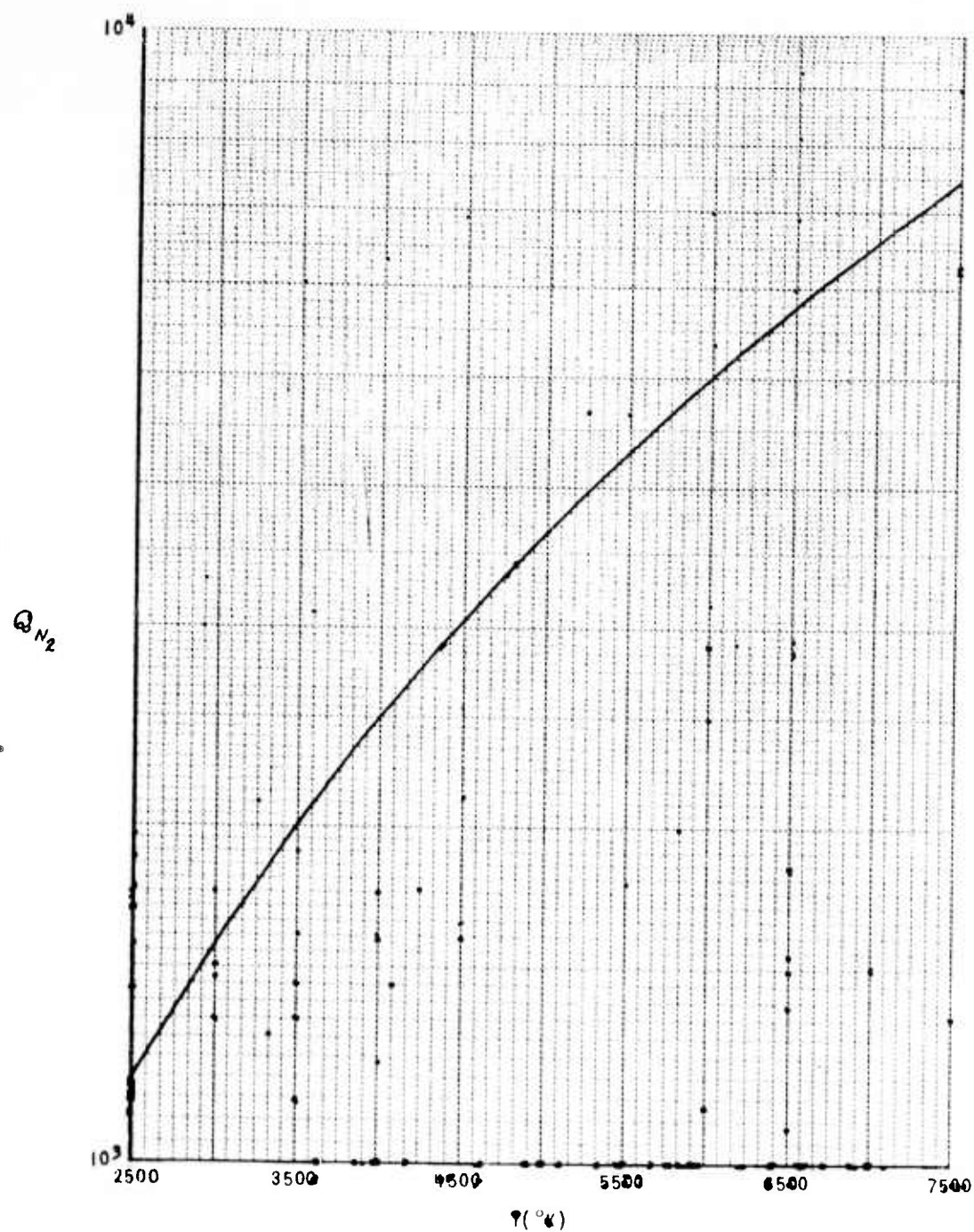
Figure 7 INTERNAL PARTITION FUNCTION FOR NITROGEN (REF. 63)
