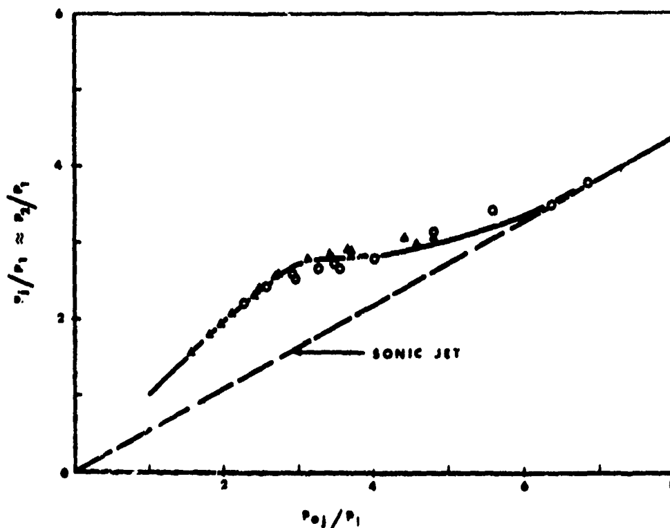
Fig. 6 APPROXIMATE PRESSURE RISE DUE TO INDUCED SHOCK WAVE (SUBSONIC \text{CO}_2 INJECTION DATA)
