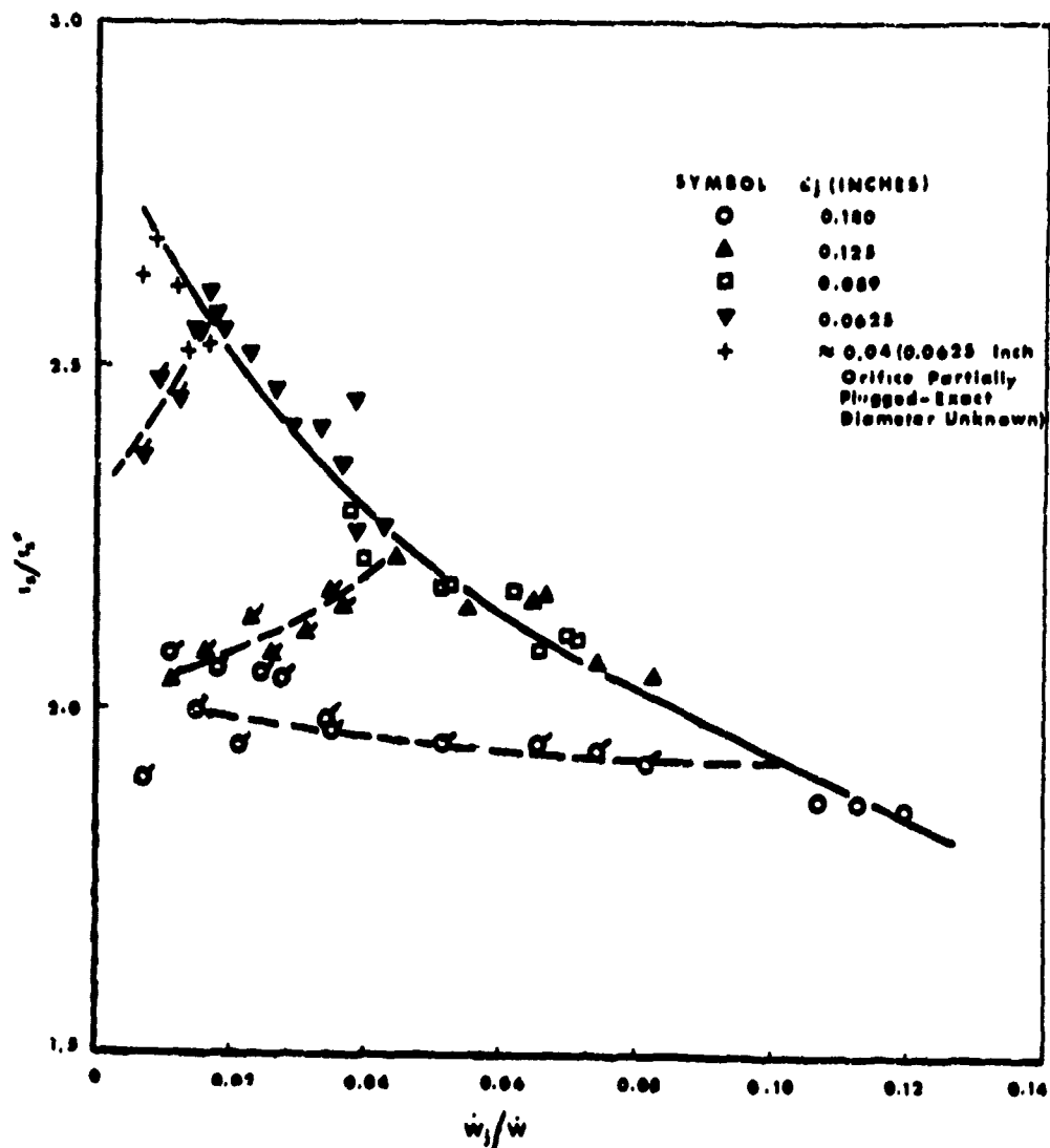
Fig. 7 CORRELATION OF SONIC SECONDARY INJECTION DATA [CO 2 INJECTANT AT 70°F; ALL SUBSONIC INJECTION DATA ( P_{o1}/P_1 4.0) ARE PLUGGED]
