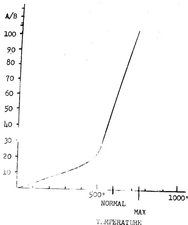
Figure 37. Characterization of EGT Scale
