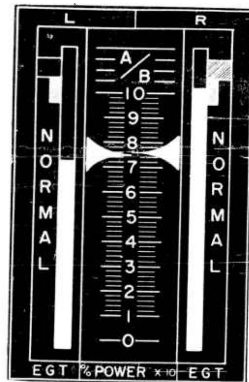
Figure 36. Engine Indicator
