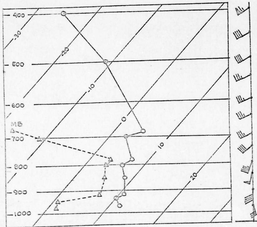
Figure 4-3d. Oklahoma City sounding for 1200Z (0600C) 27 Oct 1961.
