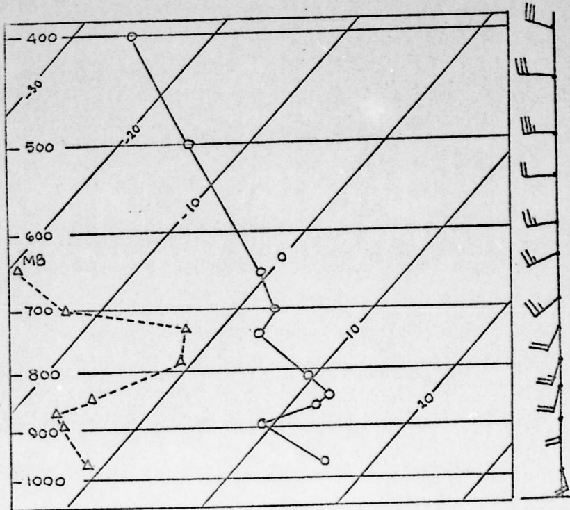
Figure 4-3c. Oklahoma City sounding for 0000Z (1800C) 26 Oct 1961.
