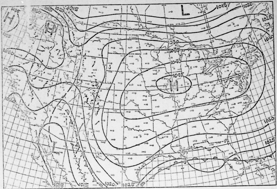
Figure 4-5. Surface Synoptic Map for 1230Z (0630C) 2 February 1959.
