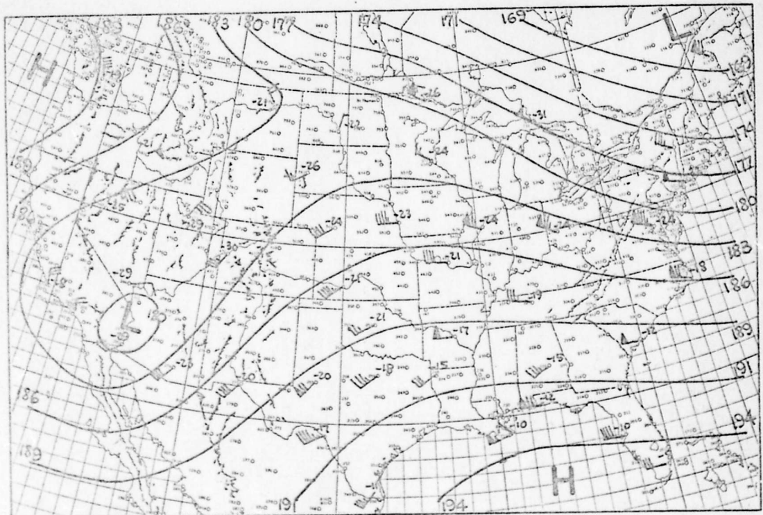
Figure 4-6. 500MB Chart for 1200Z (0600C) 2 February 1959.
