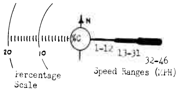
Figure 3-7b. Seasonal Surface Wind Roses. Period of Record: Dec 1942-Jan 1946, and Sep 1946-Sep 1953. Tinker AFB, Oklahoma City, Oklahoma.
