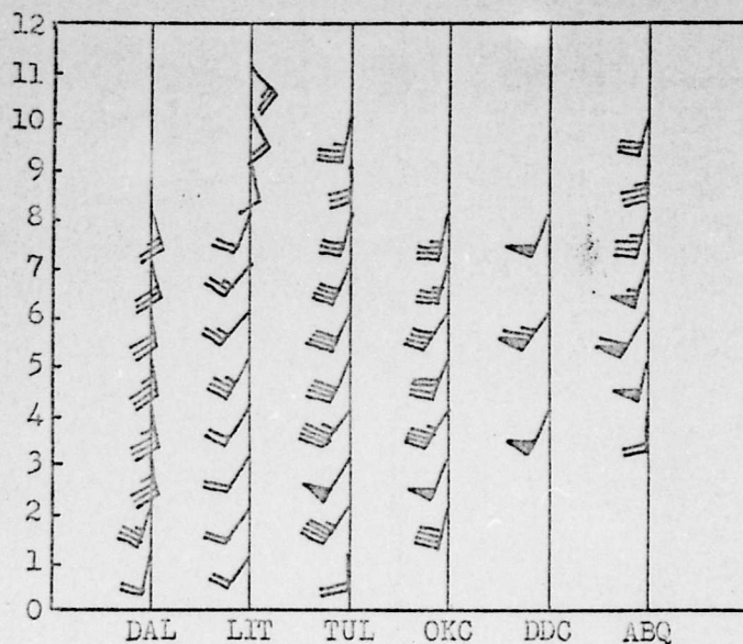
Fig. 4-23. Winds aloft for 1115Z on 17 June 1944.
