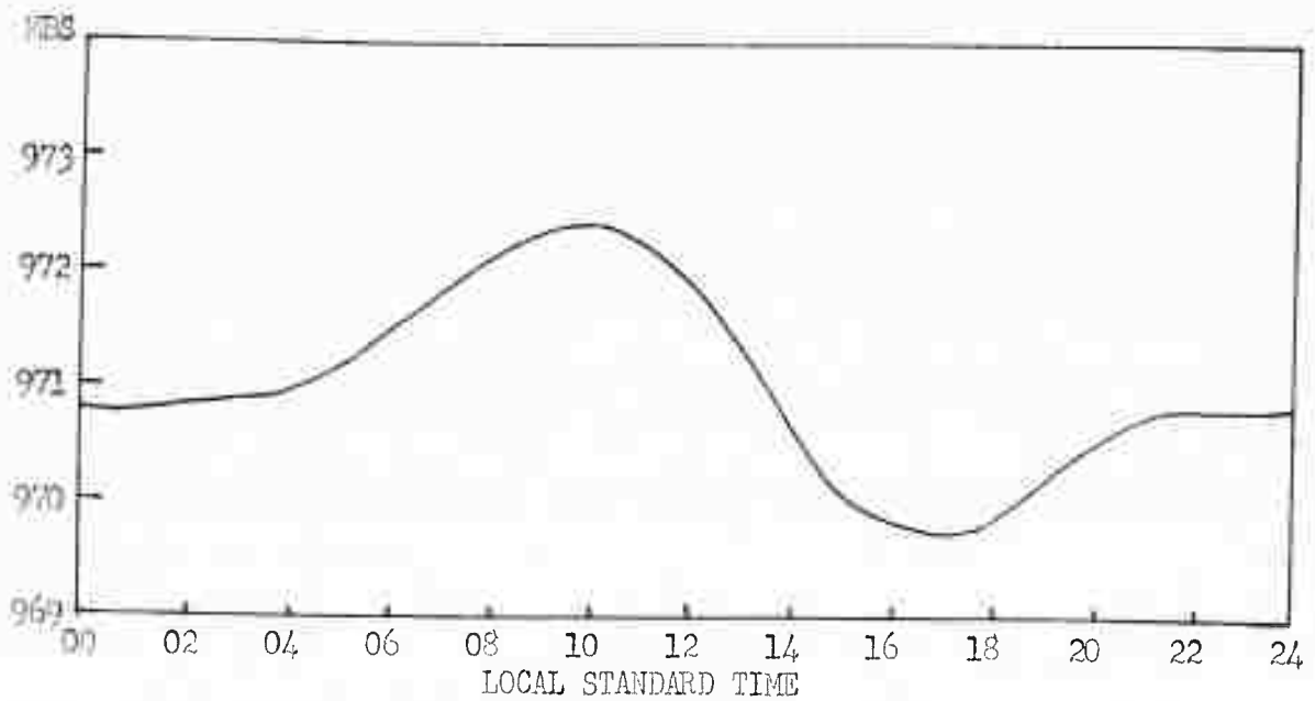
Figure 3-6s. Normal Station Pressure for Oklahoma City, Oklahoma from a Weather Bureau Summary "Normal Station Pressures (1931-1940)."
