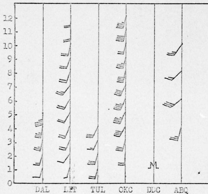
Fig. 4-24. Winds aloft for 1730Z on 17 June 1944.
