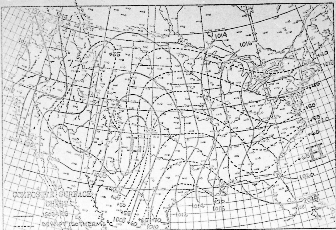
Figure 4-28. Composite maps from 66 tornado situations (449 tornadoces) that occurred in the Oklahoma area from March through June 1945 through 1953.
