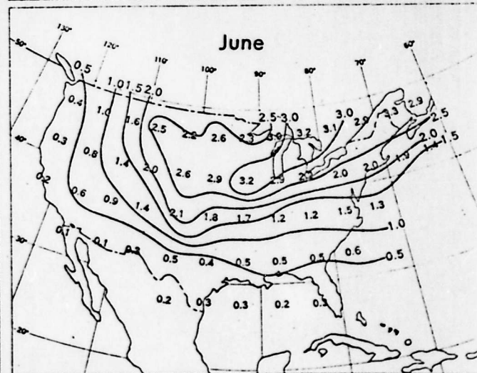
Figure 2-1a. Number of cyclones passing through each 5° latitude-longitude grid in the United States, by months, 1905-1954 (2).
