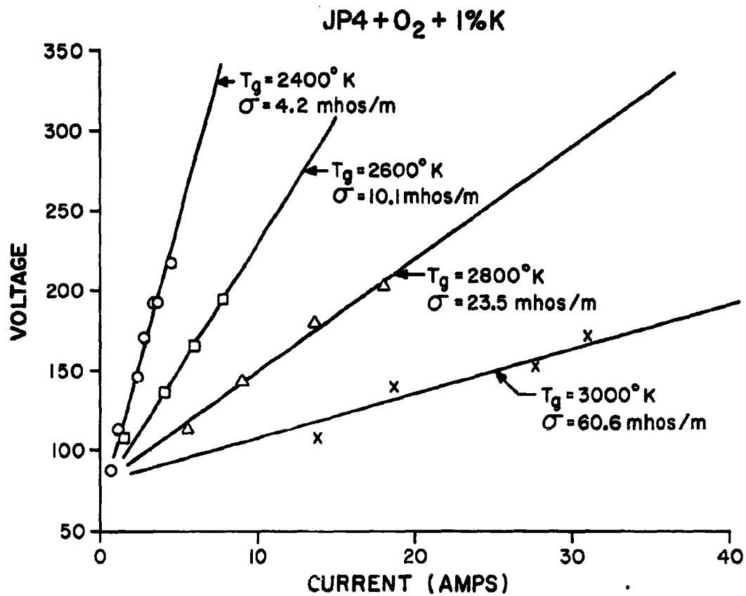
Fig. 3 DC Voltage-Current Characteristics of Seeded JP4-O 2 Combustion Products
