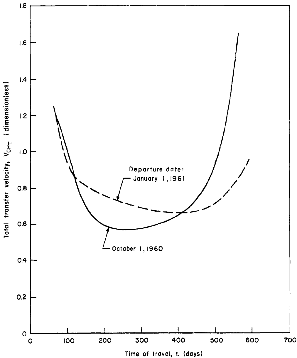
Fig.5 — Coplanar characteristic - velocity variation
