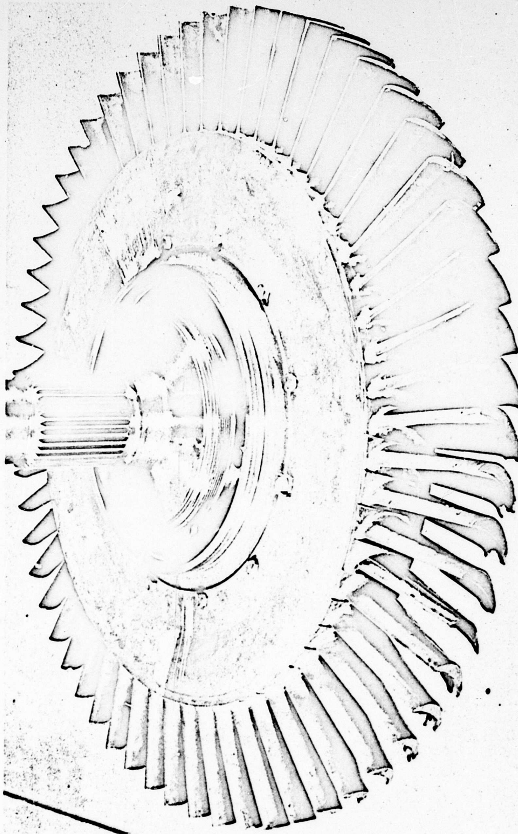
TRANSPARATION COOLED TURBINE ROTOR ASSEMBLY SHOWING BLADE WITH MISSING AIRFOIL AFTER TEST (FRONT)
