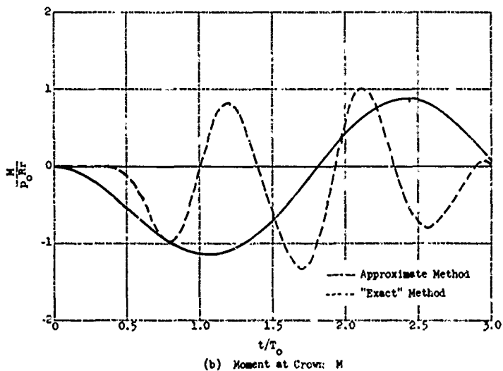
FIG. 4. COMPARISON OF RESPONSE CURVES FOR UNIFORM PRESSURE, p_0/\rho_{gr} = 2.0 Other data same as in Fig. 2
