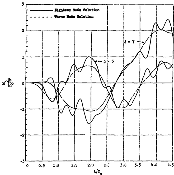
FIG. 12 RESPONSE CURVES FOR AXIAL FORCE AND MOMENTS \varphi = 90^\circ , L_0/\pi = 100 , t_i/T_0 = 1.5 , t_d/T_0 = 3
