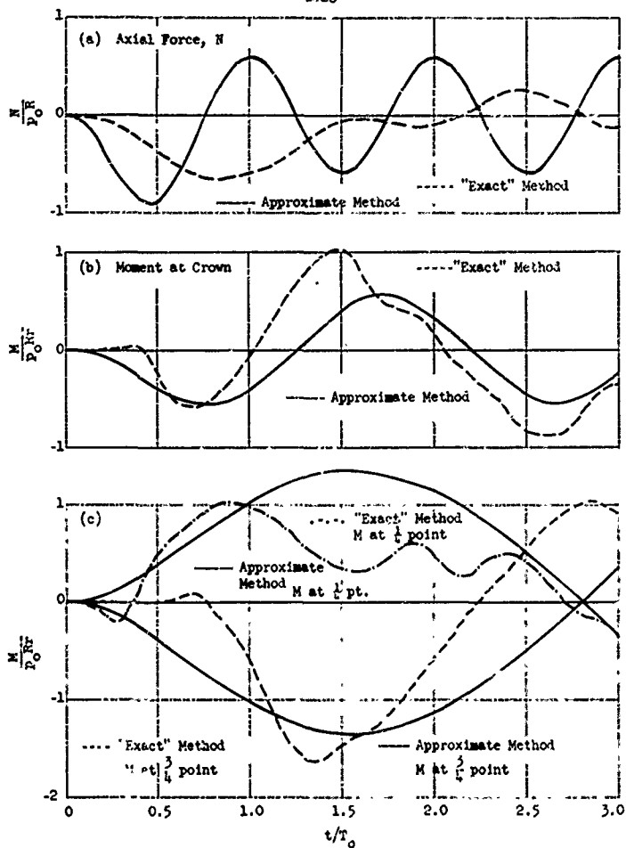
FIG. 14 COMPARISON OF RESPONSE CURVES FOR A MOVING PRESSURE PULSE t/L_0 = 0.2 , L_0/r = 100 , p_0/p_{cr} = 1 , t_i/T_0 = 1 , t_d/t_i = 1
