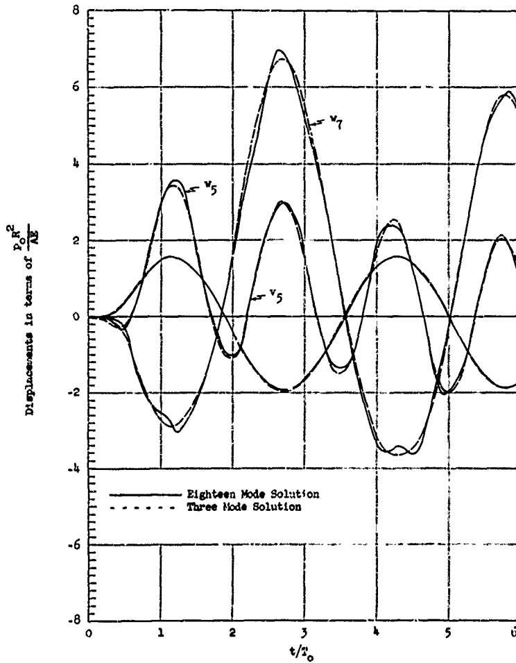
FIG. 7 RESPONSE CURVES FOR DISPLACEMENTS \phi_0 = 60^\circ , L_0/r = 100 , t_0/T_0 = 1 , t_d/T_0 = 5
