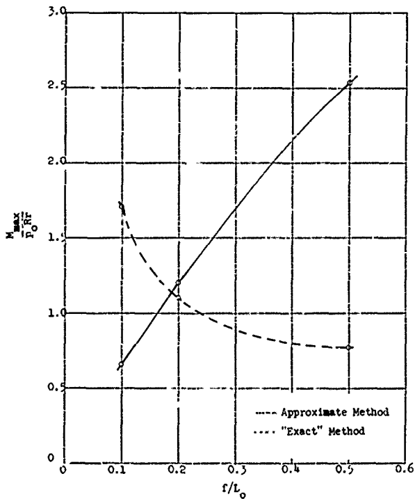
FIG. 13 COMPARISON OF SPECTRUM FOR MAXIMUM CROWN MOMENT-- r/L_0 VARIED
