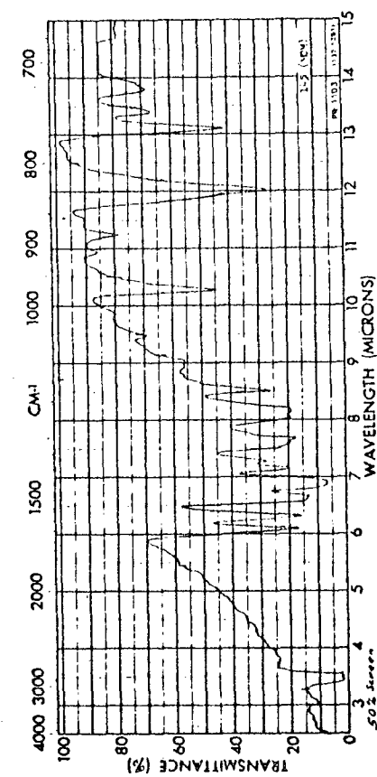
c. Poly-2-(p-phenylene)-6-carboxamido-benzothiazole
