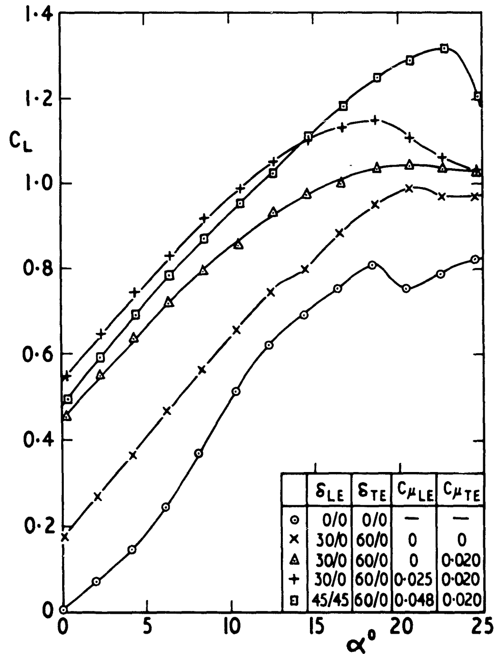
Fig.5 Blowing at knee of leading-edge and trailing-edge flaps; untapered, sharp-edged 55° swept wing
