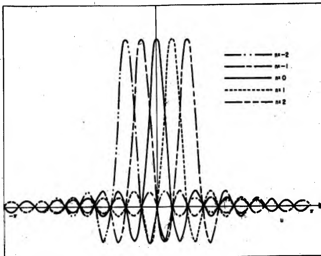
Figure 27. Illustration of coverage of five beams for 20 element simultaneously scanned array.
