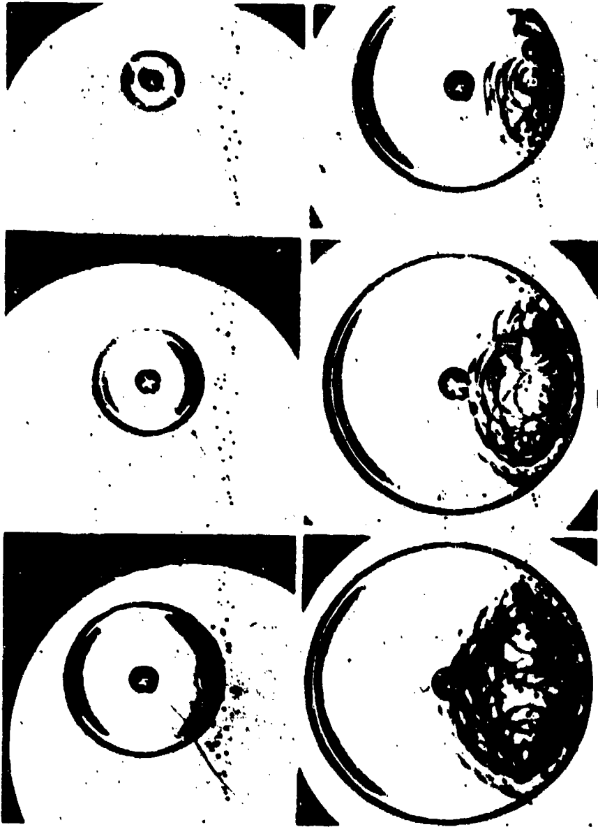
Figure 14. Six consecutive phases of an underwater bubble passing over enclosed air bubbles. Implosion of the air bubble.
