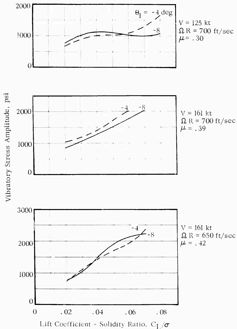
FIG.12. EXPERIMENTAL EFFECT OF BLADE TWIST AND LIFT ON FLATWISE STRESS, f/\pi R^2 = 0.005
