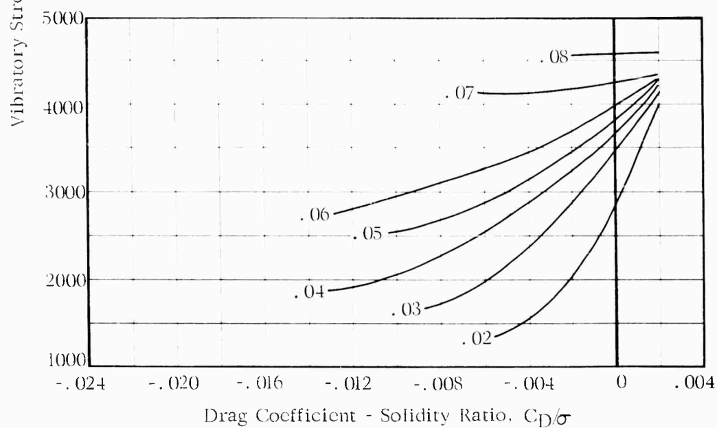
(b) Flatwise Stress, 33.4 % Radius
