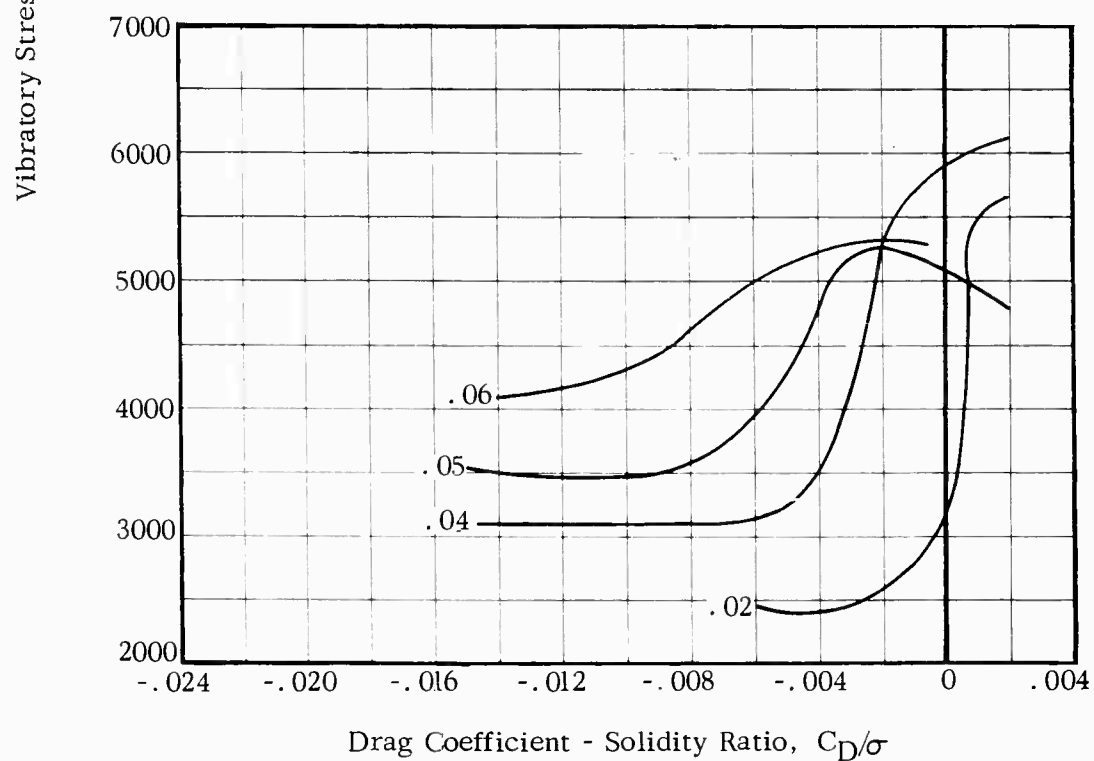
(e) Flatwise Stress, 80.5 % Radius
