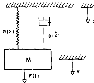
Fig. 1 - The simple oscillator
