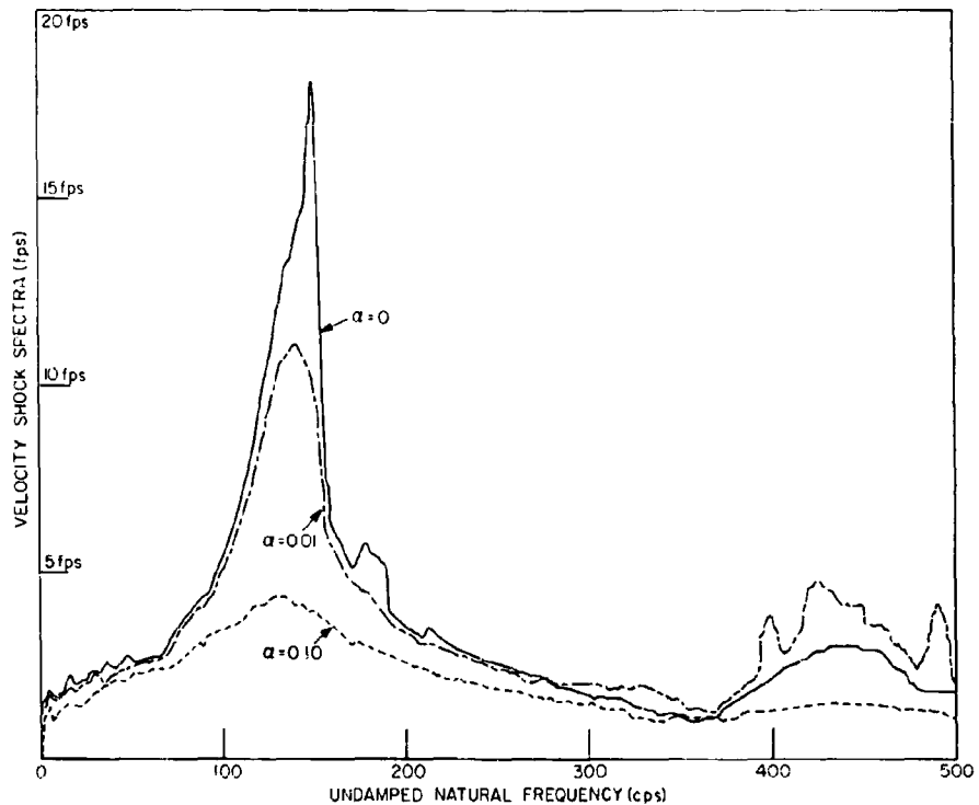
Fig. 5 - Undamped and damped shock spectra
