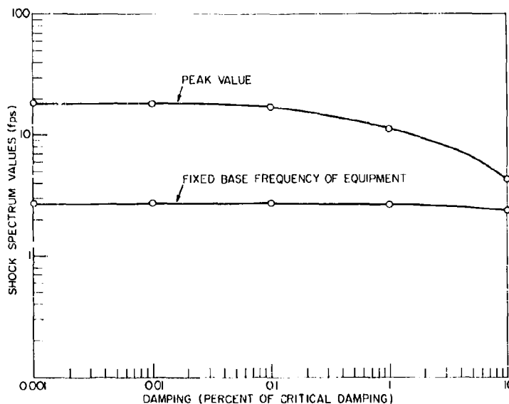
Fig. 6 - Effect of damping upon the shock spectrum values of interest
