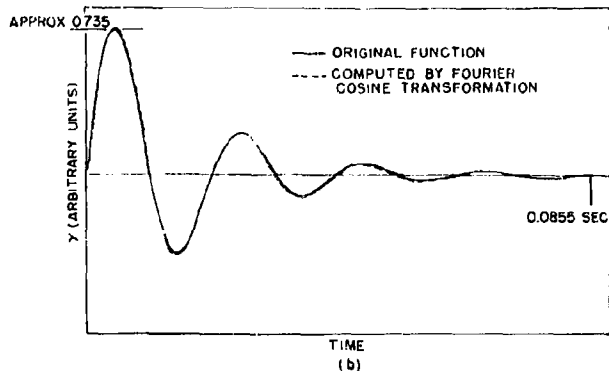
Fig. 3 - Comparison of results for Case II, a damped sine wave
