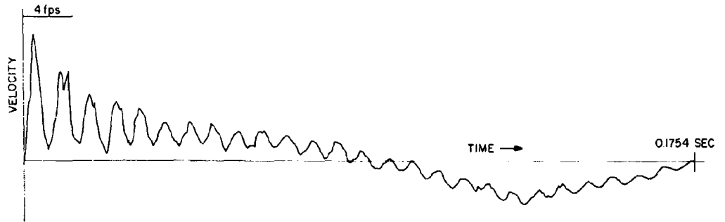
Fig. 4 - Foundation velocity
