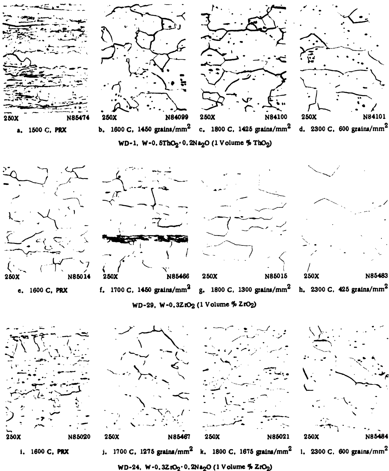
FIGURE 16. LONGITUDINAL MICROSTRUCTURES OF THE 1 VOLUME PER CENT DISPERSOID ALLOYS ILLUSTRATING STRUCTURAL CHANGES OCCURRING AFTER ANNEALING 1 HOUR AT THE INDICATED TEMPERATURES
