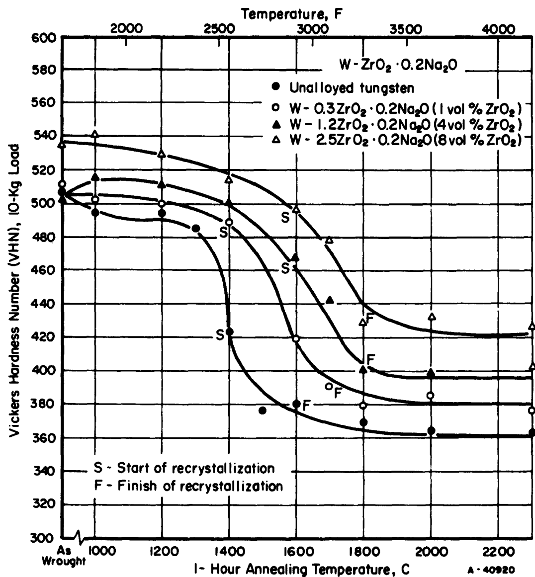
FIGURE 9. SOFTENING CURVES FOR WROUGHT UNALLOYED TUNGSTEN AND THE 1, 4, AND 8 VOLUME PER CENT ZIRCONIA DISPERSOID ALLOYS PREPARED FROM 0.01-MICRON COLLOIDAL ZIRCONIA
