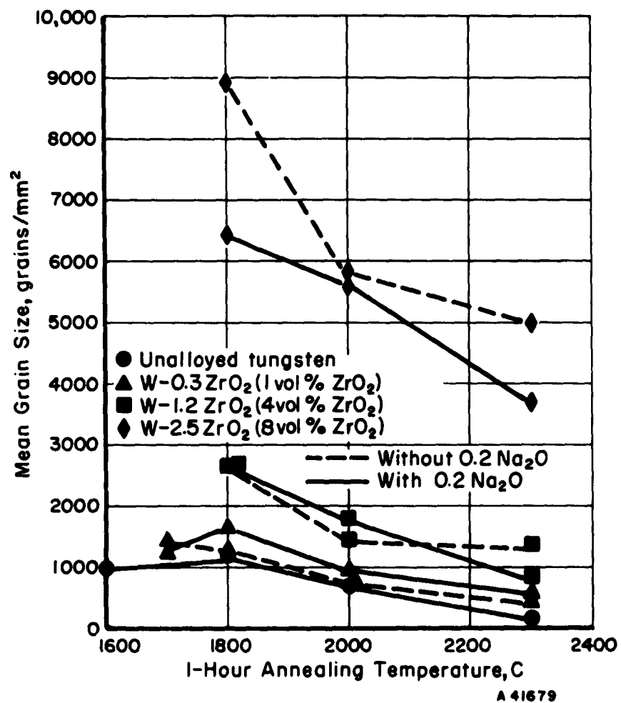
FIGURE 14. GRAIN-GROWTH BEHAVIOR AT UNALLOYED TUNGSTEN AND THE 1, 4, AND 8 VOLUME PER CENT ZIRCONIA DISPERSOID ALLOYS PREPARED FROM 0.01-MICRON COLLOIDAL ZIRCONIA
