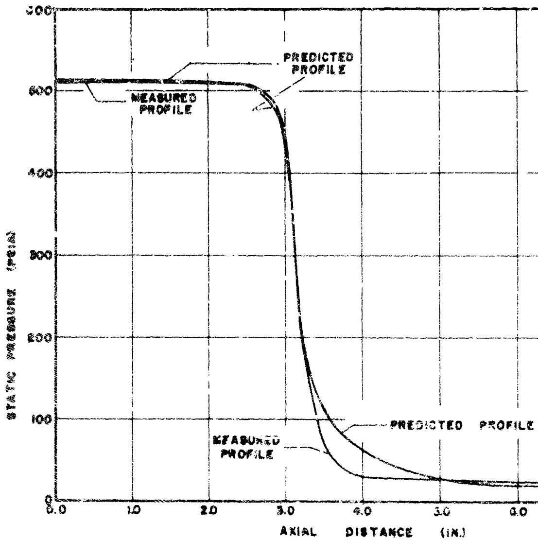
FIG. 13 PREDICTED AND MEASURED STATIC PRESSURE PROFILES FOR NOZZLE I ( W_2/W_1 = 0.18 )
