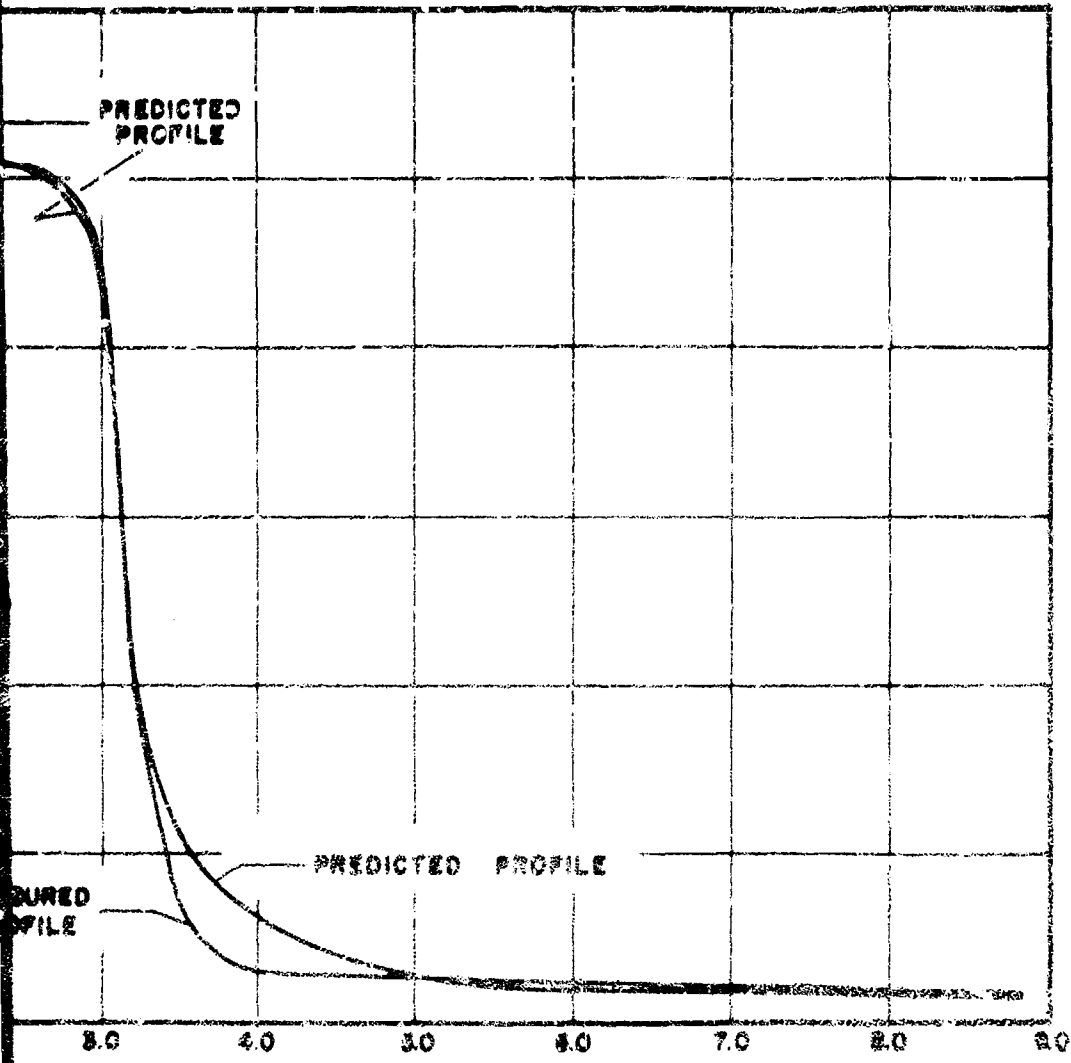
AXIAL DISTANCE (IN.) PREDICTED AND MEASURED STATIC PRESSURE PROFILES FOR NOZZLE 2 ( M_0/M_1 = 0.16 )
