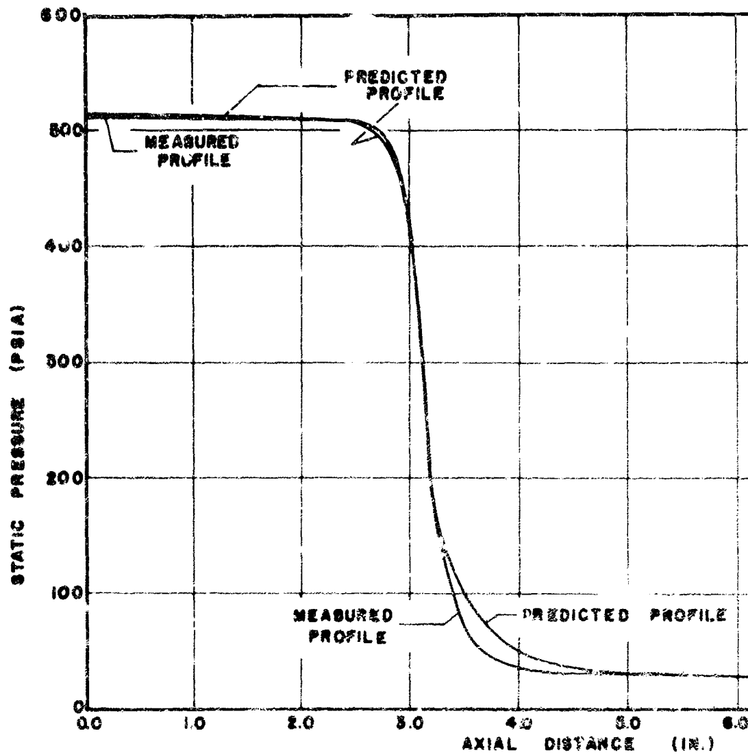
FIG. 12 PREDICTED AND MEASURED STATIC PRESSURE PROFILES FOR NOZZLE I ( M_0/W_0 = 0.10 )
