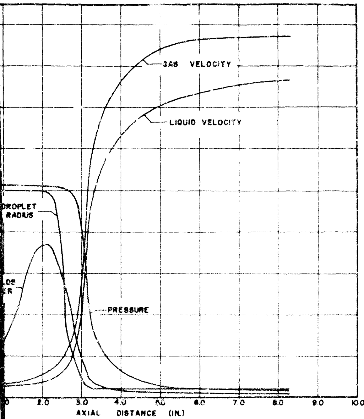
RELATED FLOW PARAMETERS FOR NOZZLE I ( N_0/W = 0.15 ) A FUNCTION OF THE AXIAL DISTANCE ALONG THE NOZZLE
