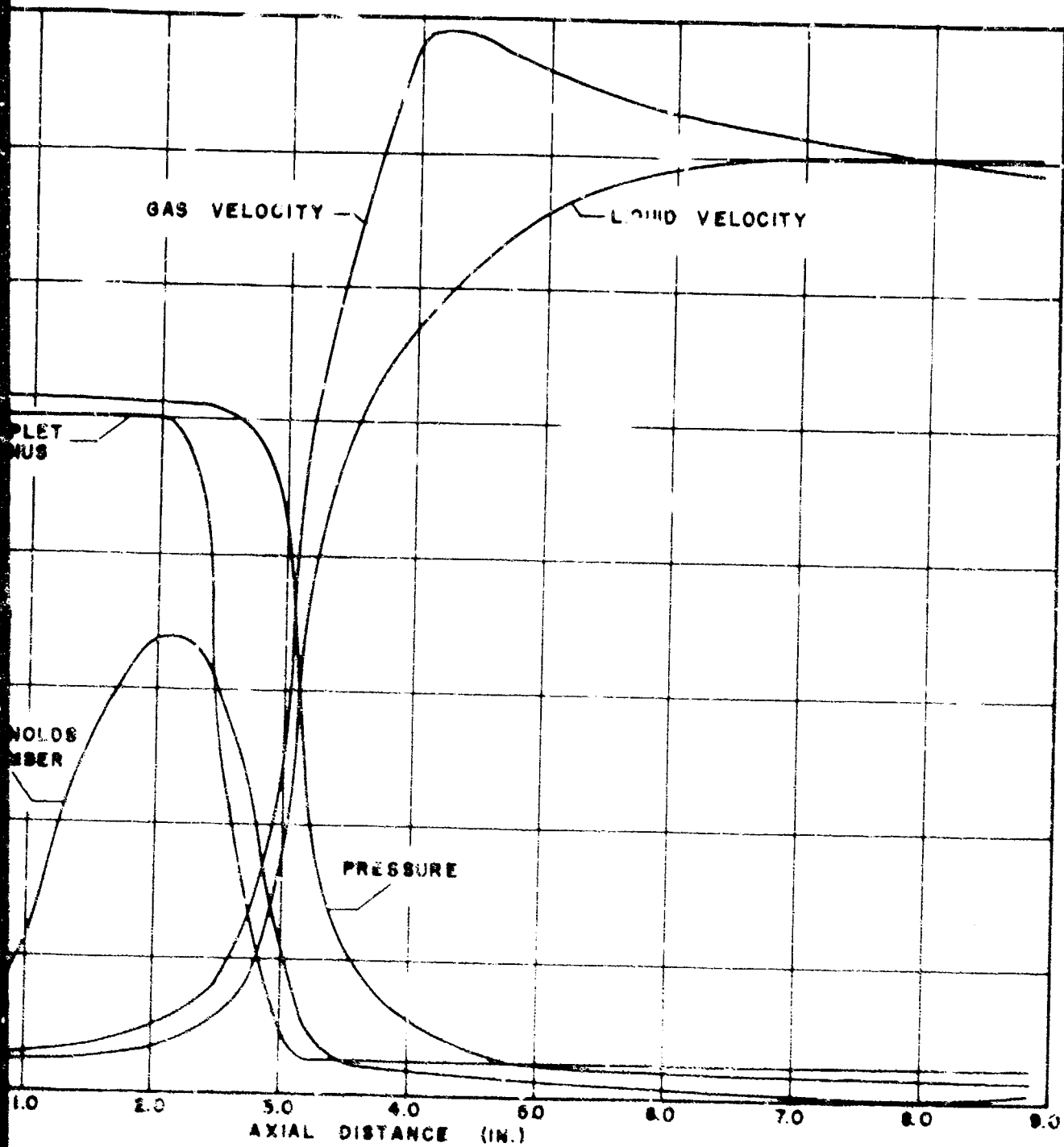
CALCULATED FLOW PARAMETERS FOR NOZZLE I ( W_g/W_L = 0.10 ) AS A FUNCTION OF THE AXIAL DISTANCE ALONG THE NOZZLE
