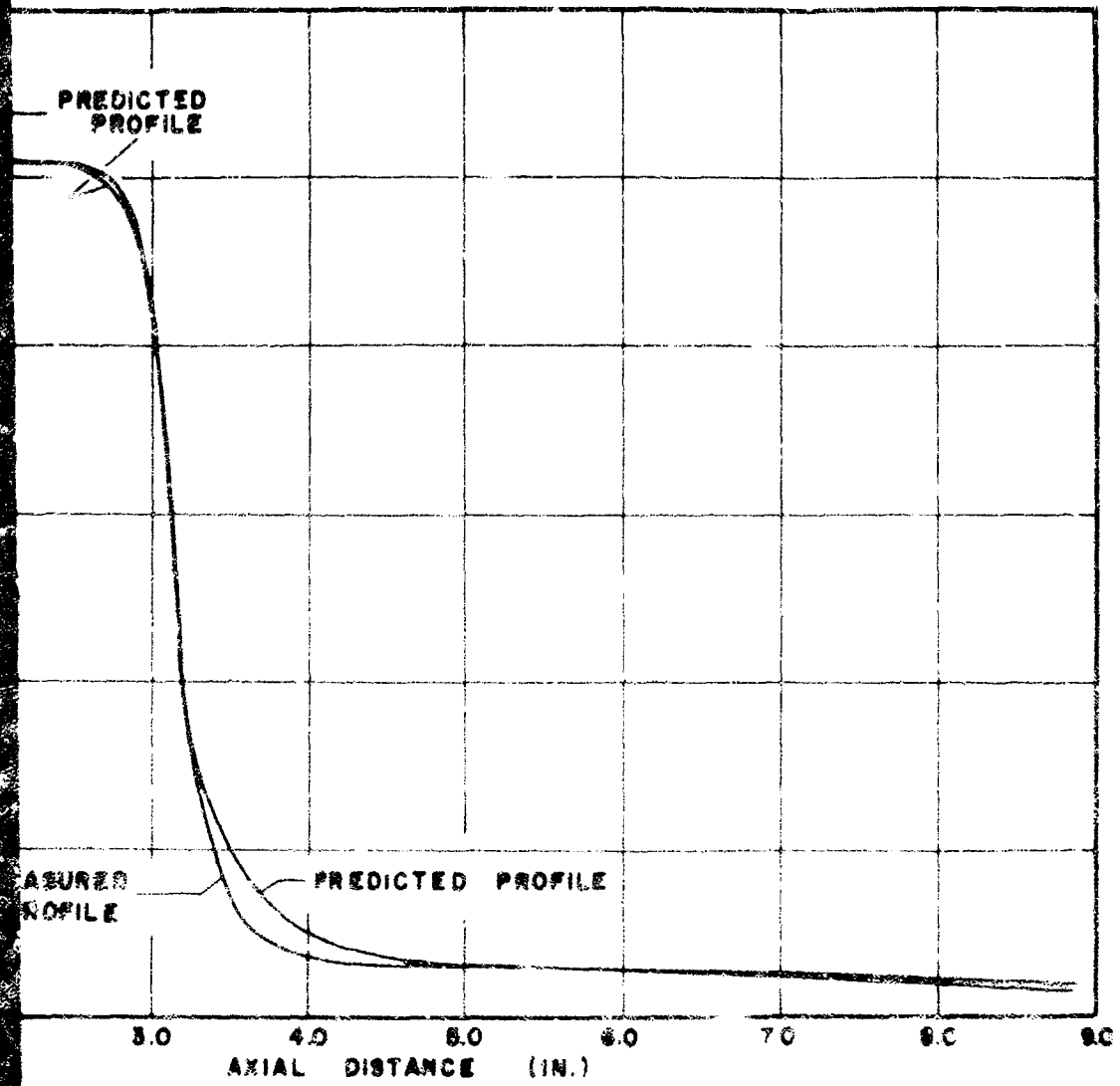
PREDICTED AND MEASURED STATIC PRESSURE PROFILES FOR NOZZLE I ( v_0/v_L = 0.10 )
