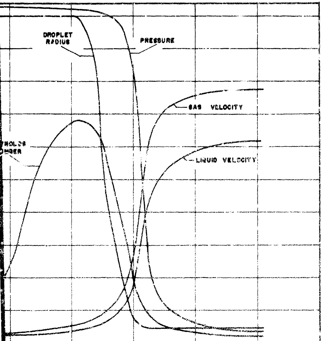
AXIAL DISTANCE (MM) PARAMETERS FOR NOZZLE X ( W/W_0 = 0.10 ) THE AXIAL DISTANCE ALONG THE NOZZLE
