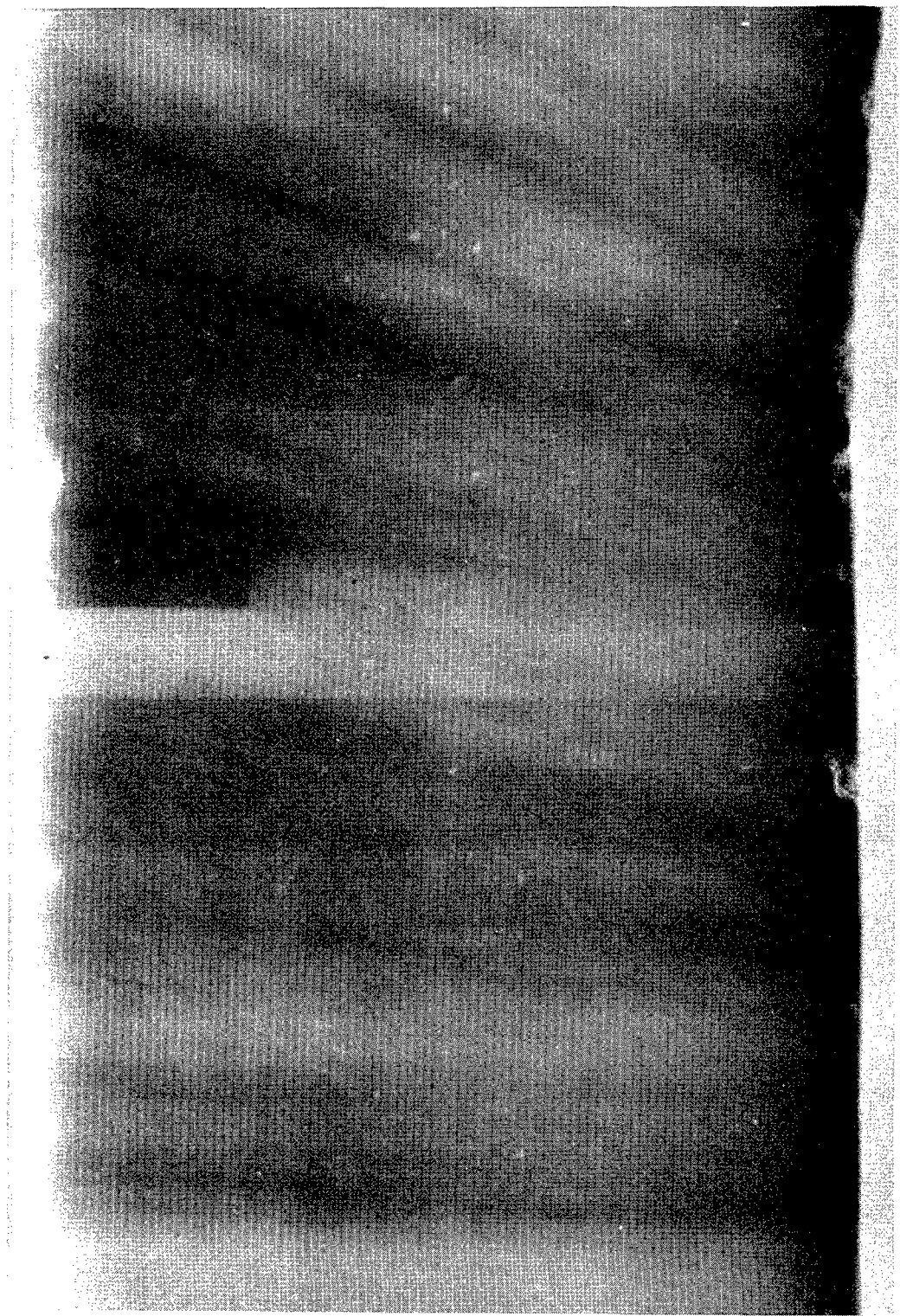
FIG. 18 - RADIOGRAPH OF 5-INCH THICK SAND-CAST SLAB; 1/2-INCH THICK SLICE (RADIATING LINES ARE SAW MARKS.)
