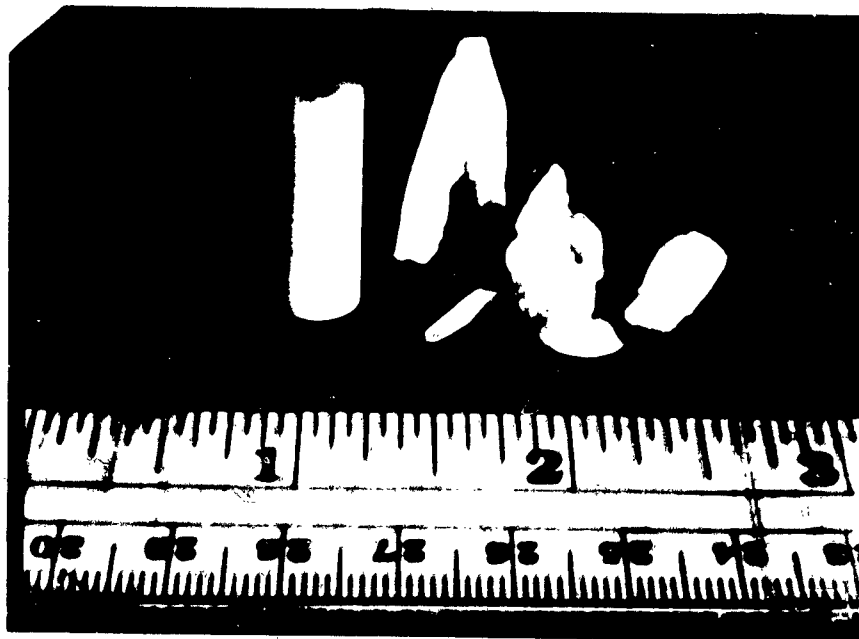
Fig. 4-14 LUCALOX SPECIMENS BEFORE AND AFTER TESTING UNDER COMPRESSIVE LOADING AT 1600°C Grain Size = 0.005 mm
