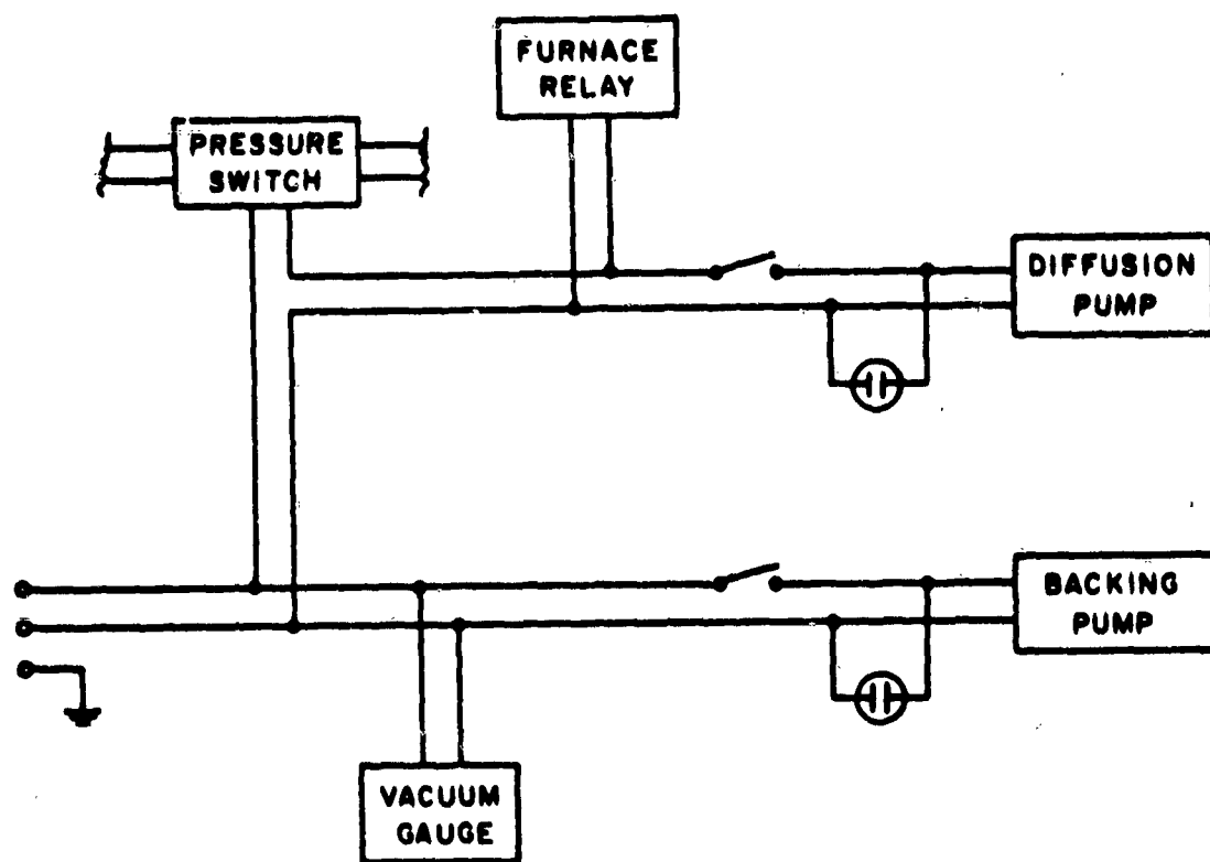
Fig. 5-10 CART CONNECTIONS
