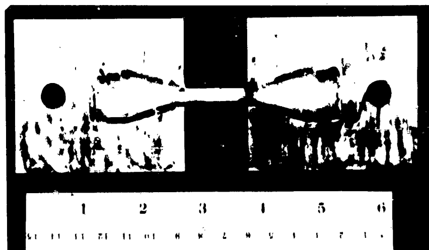
Fig. 2-10 PRECISION TENSILE SPECIMEN CEMENTED IN TENSILE GRIPS
