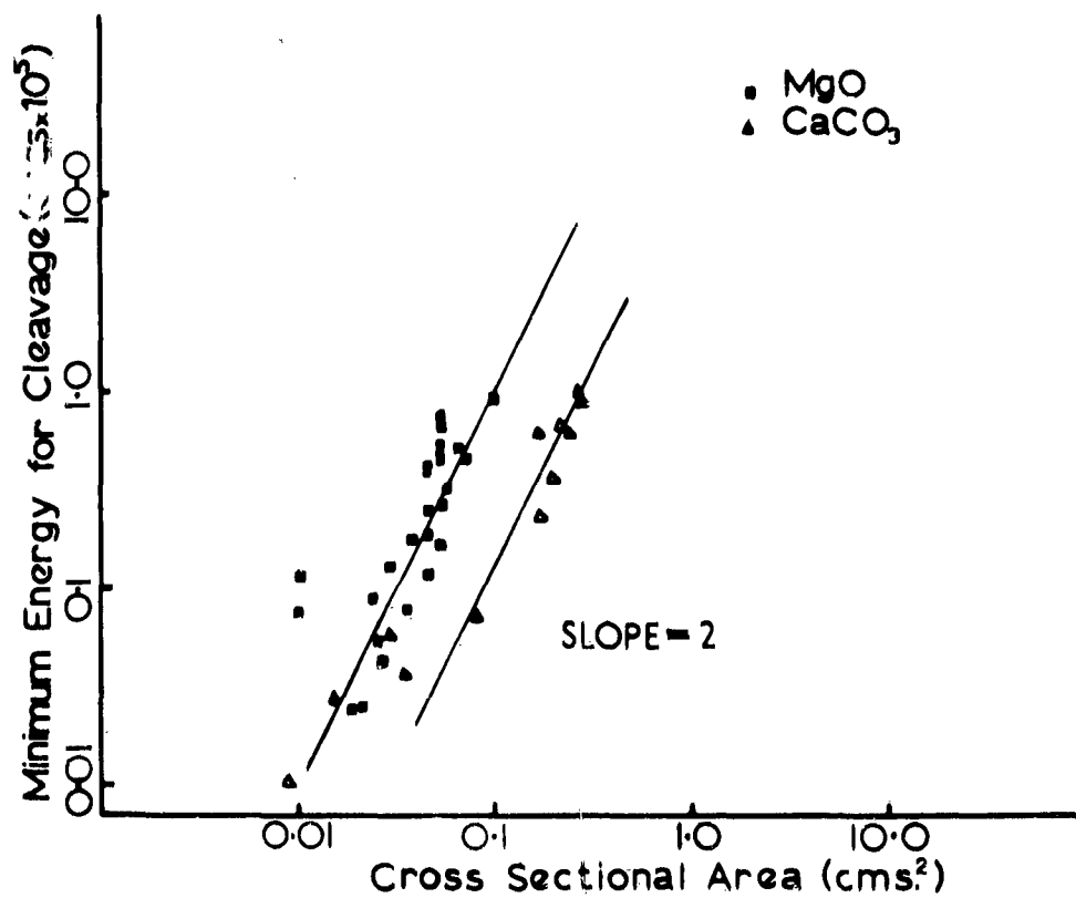
Fig. 6-2 MINIMUM TUP ENERGY FOR CLEAVAGE VERSUS CROSS SECTIONAL AREA OF CRYSTAL FOR MgO AND CaCO 3 CRYSTALS
