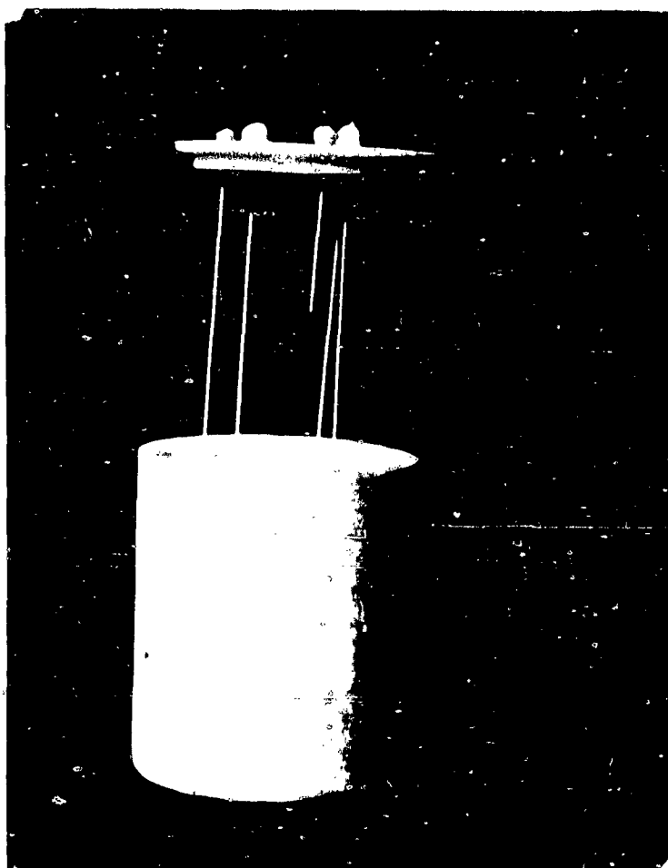
Fig. 6-11 GENERAL VIEW OF \text{Al}_2\text{O}_3 ROD ASSEMBLY USED
