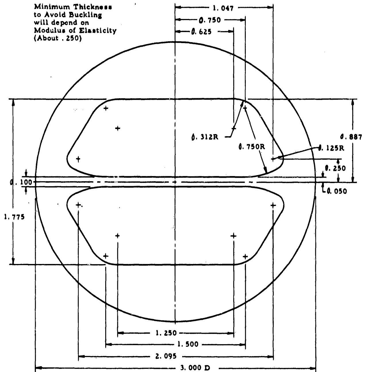
Fig. 3-3 THETA SPECIMEN GEOMETRY
