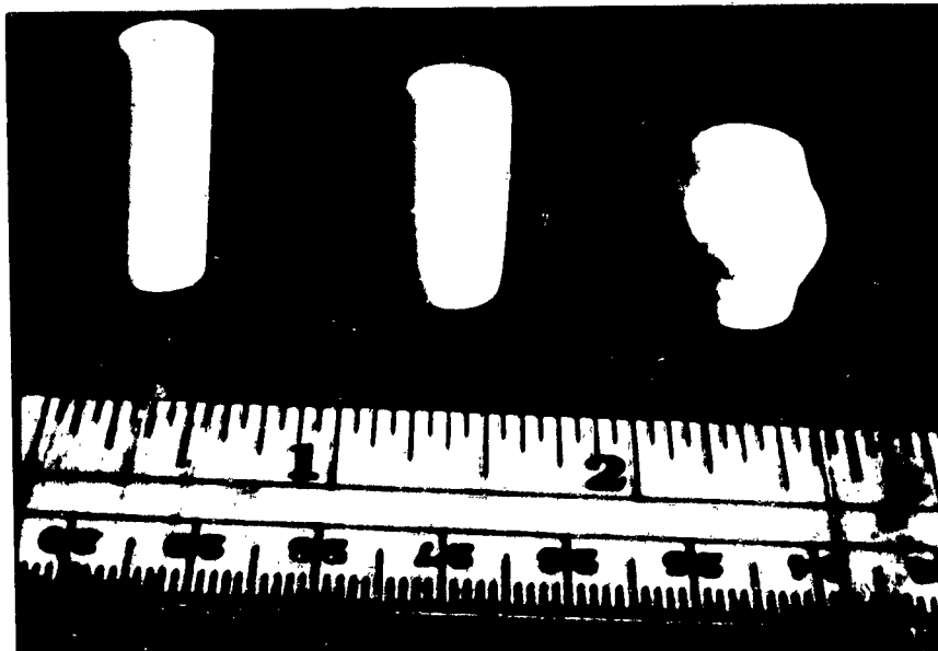
Fig. 4-16 LUCALOX SPECIMENS BEFORE AND AFTER TESTING UNDER COMPRESSIVE LOADING AT 1900°C Grain Size = 0.005
