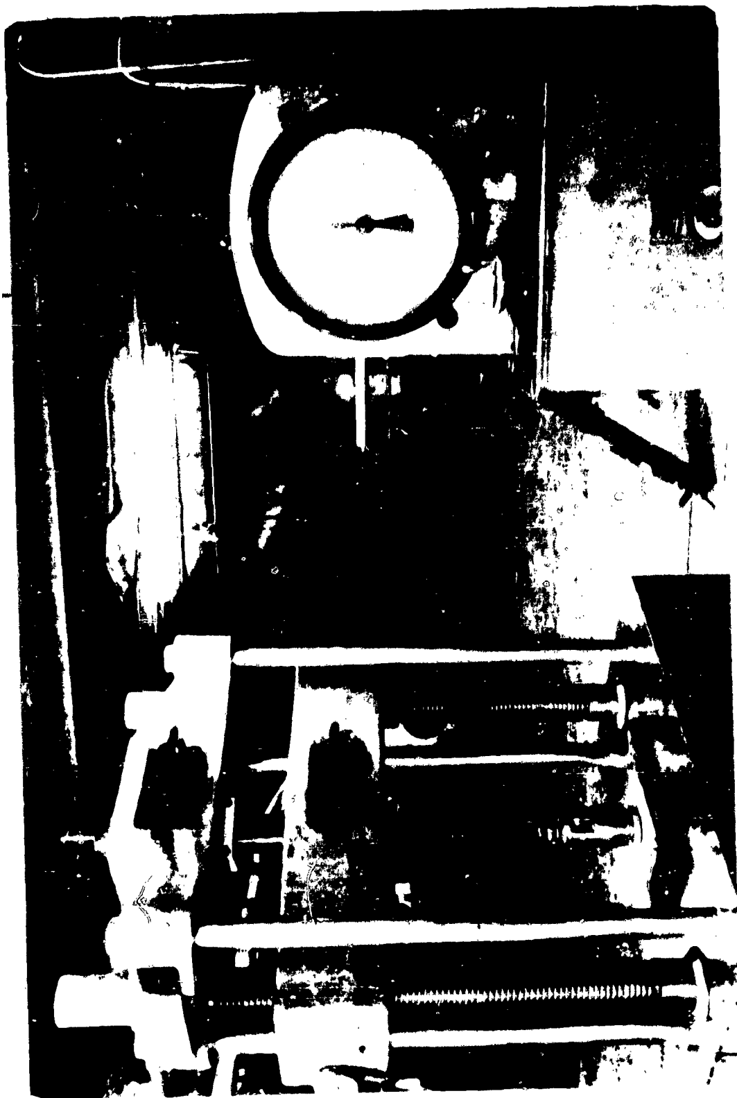
Fig. 2-3 INSTALLATION OF SPRING LOADED DEVICE IN TESTING MACHINE
