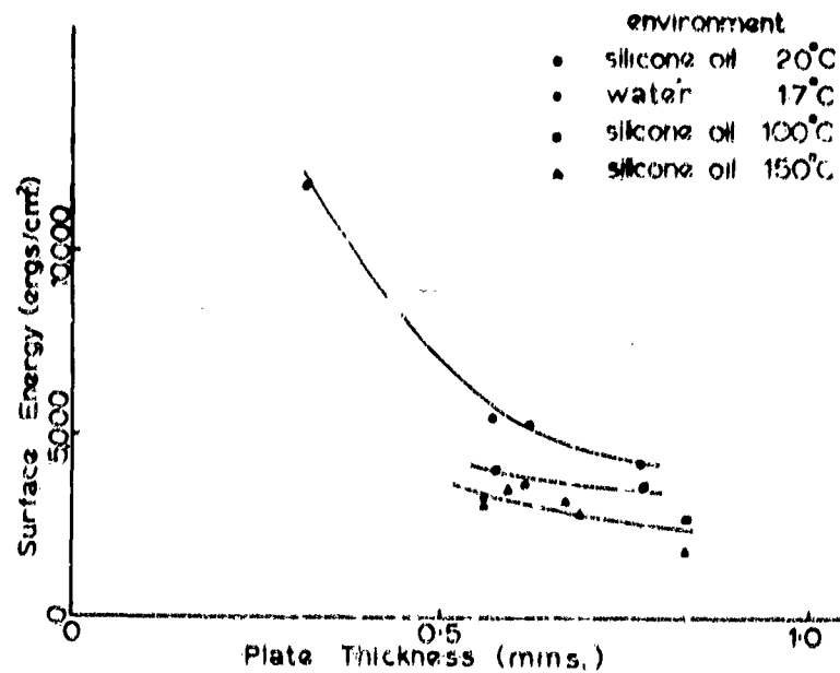
Fig. 6-5(a) CALCULATED SURFACE ENERGY OF Al_2O_3 FROM BREAKING STRESS DATA VERSUS PLATE THICKNESS
