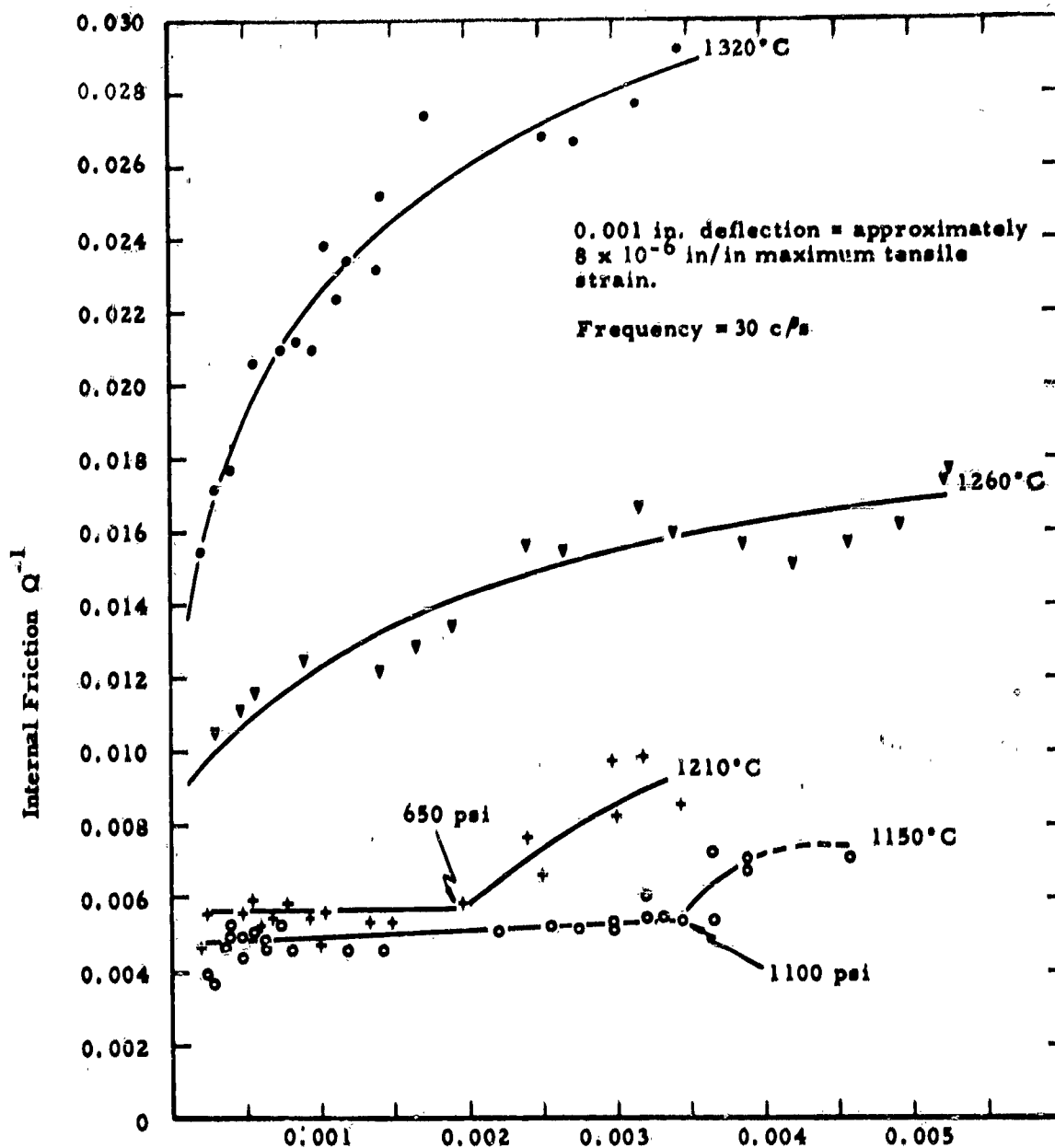
Fig. A-4 AMPLITUDE VARIATION OF Q^{-1}
