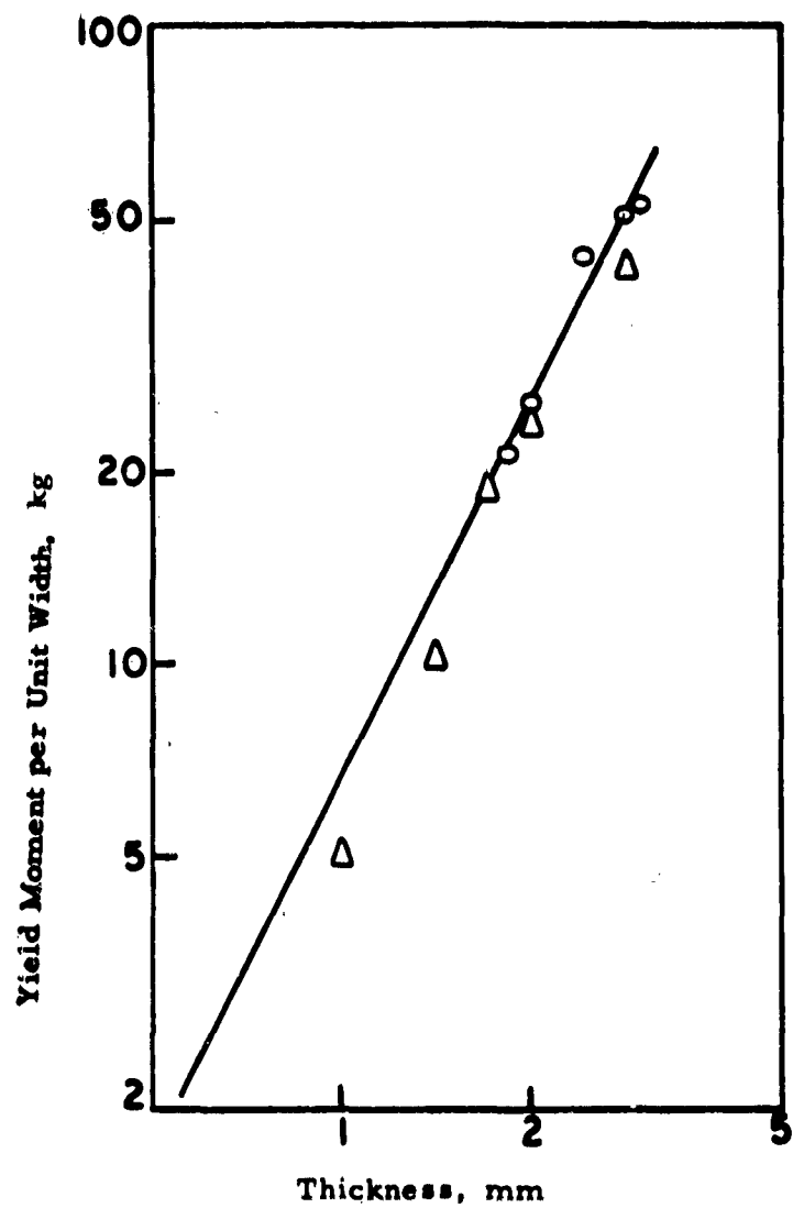
Fig. 5-15 YIELD MOMENT VS. BEAM THICKNESS FOR MgO SINGLE CRYSTALS AT ROOM TEMPERATURE
