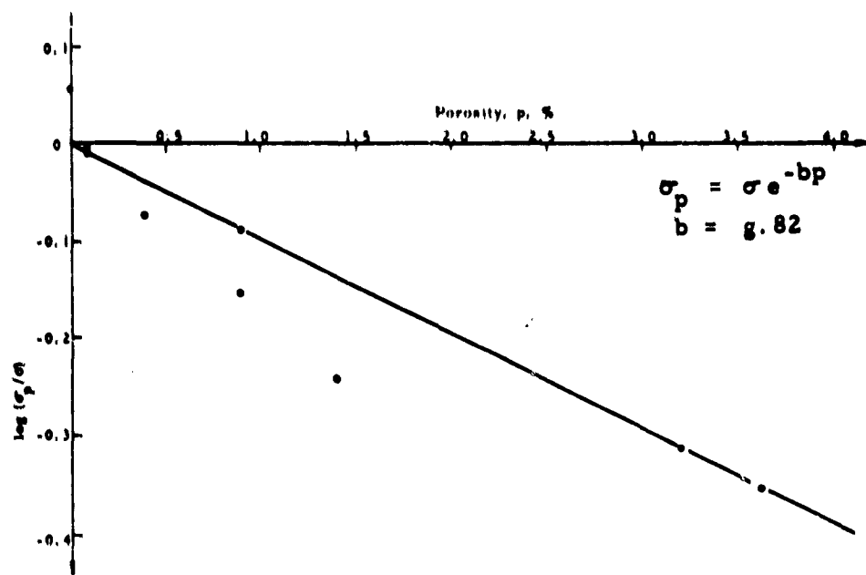
Fig. 5 DEPENDENCE OF STRENGTH ON POROSITY IN LUCALOX
