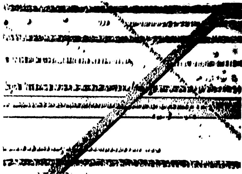
Fig. 10-13 THE REACTIVATION OF SHORT SLIP BAND SEGMENTS FOLLOWING AN ANNEAL (a) at 600°C, (b) at 800°C (X250)
