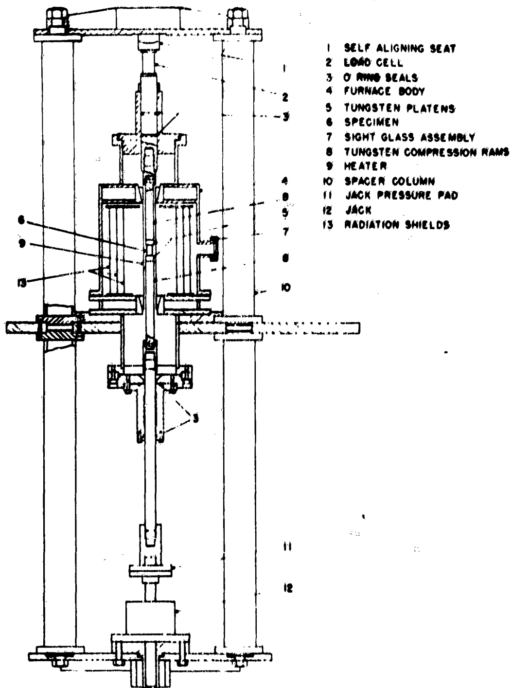
Fig. 4-1 HIGH TEMPERATURE COMPRESSION TESTING APPARATUS
