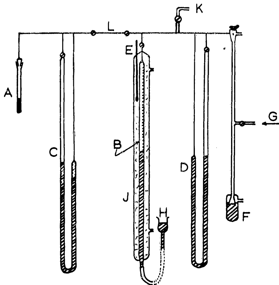
Fig. 6-6 DIAGRAMMATIC SKETCH OF ADSORPTION SYSTEM (Capillary sections are represented by a single line.)
