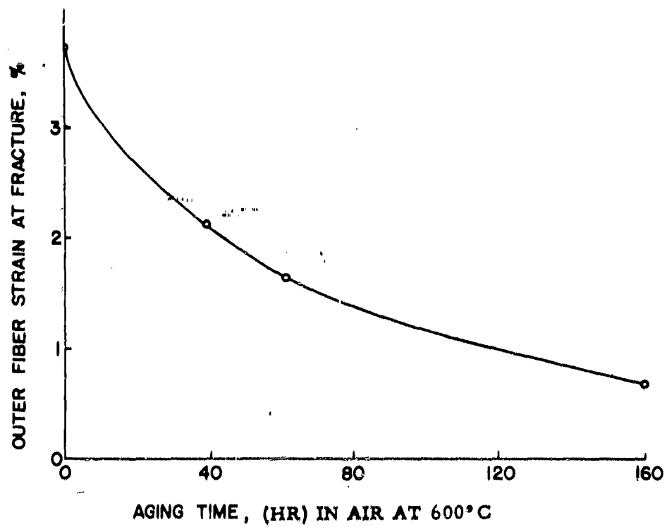
Fig. 11-8 EFFECT OF AGING AT 600°C ON DUCTILITY OF MgO SINGLE CRYSTALS
