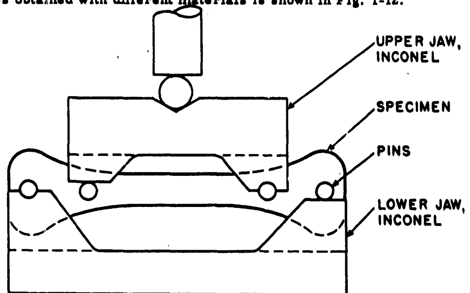
Fig. 1-11 FLEXURE TEST FIXTURE
