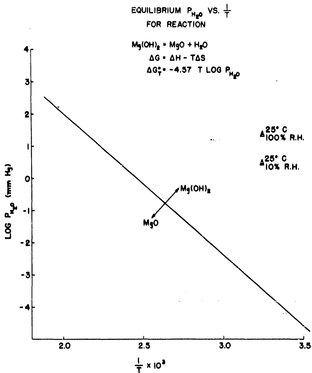
Fig. 11-3 EQUILIBRIUM CONDITIONS FOR Mg(OH)_2 REACTION
