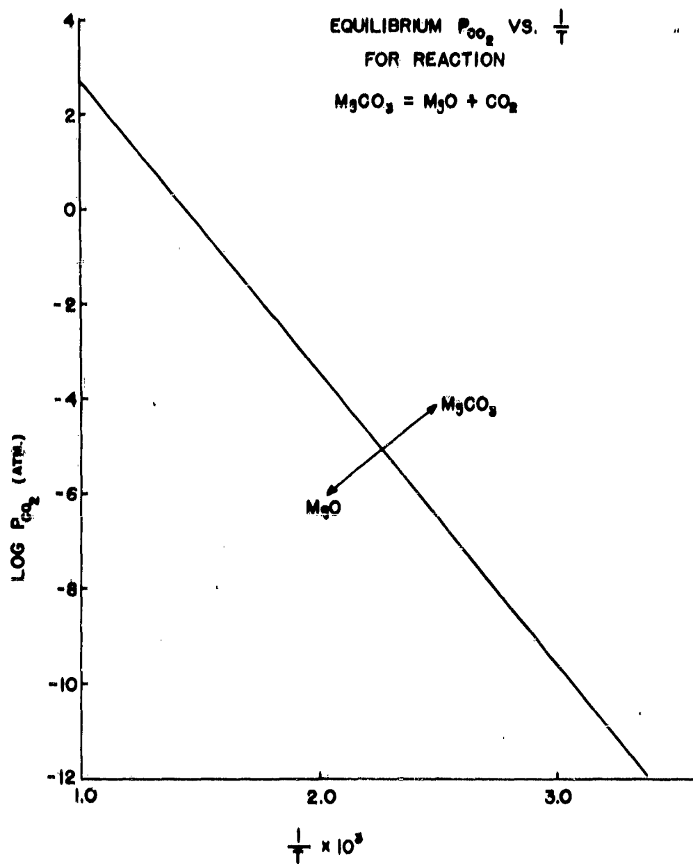
Fig. 11-2 EQUILIBRIUM CONDITIONS FOR \text{MgCO}_3 REACTION
