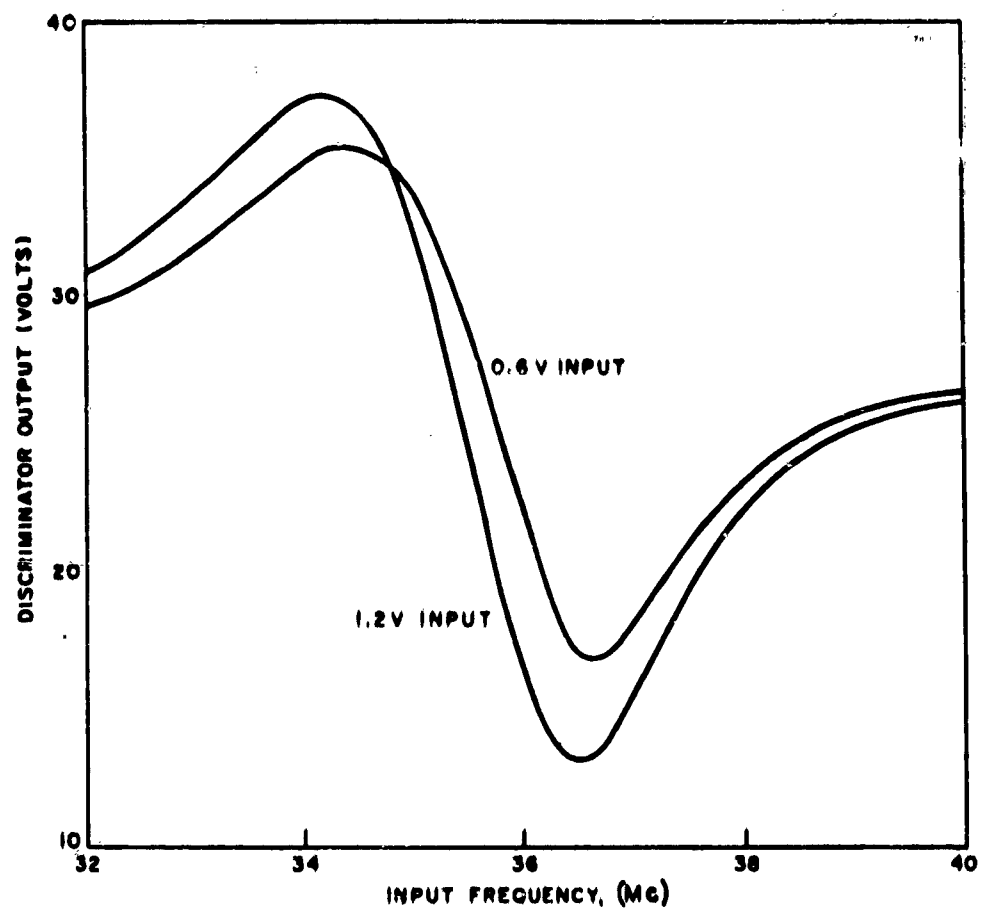
Fig. 5-6 DISCRIMINATOR CURVE
