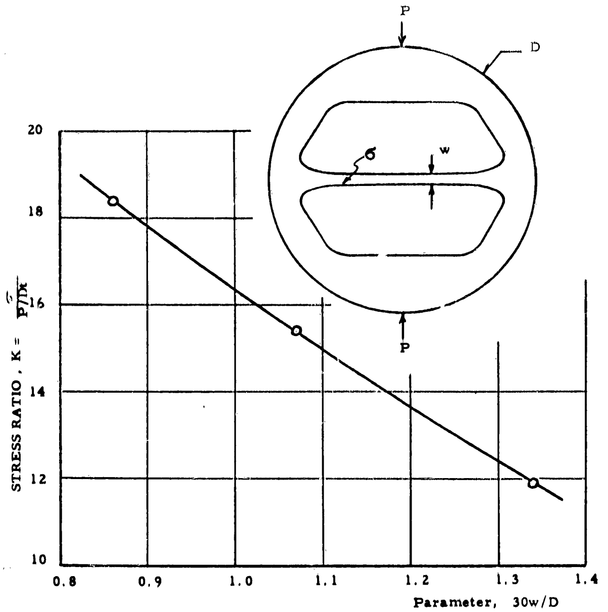
Fig. 3-9 STRESS-LOAD RELATION FOR GEOMETRIC VARIATIONS IN THE THETA SPECIMEN
