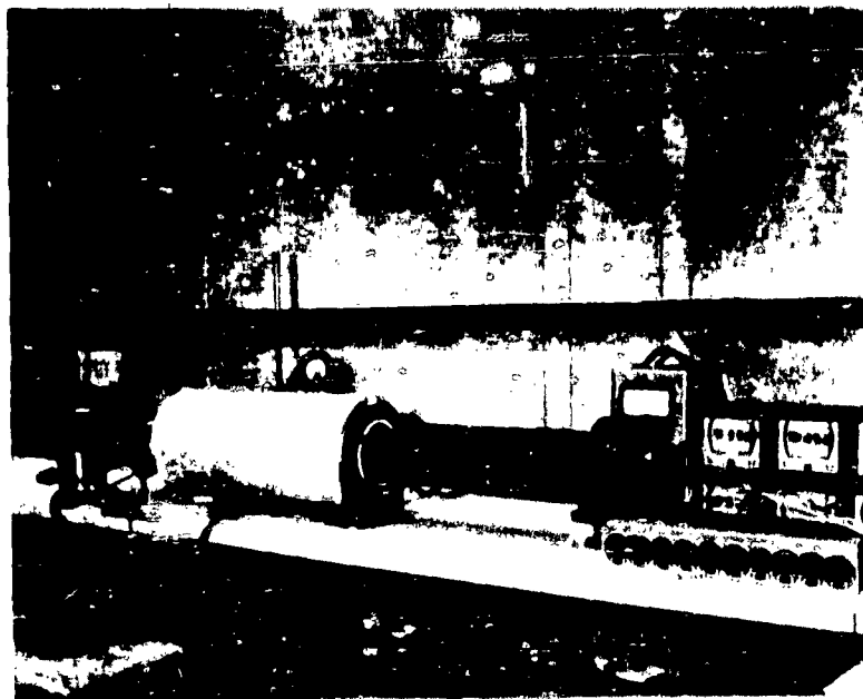
Fig. 9-6 LOW-TEMPERATURE AUTOCLAVE TEST APPARATUS
