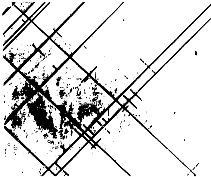
Fig. 10-2 NUCLEATION SLIP ON INTERSECTING SYSTEMS BY A PASSING SLIP BAND FOR SPECIMENS SUBJECTED TO TENSION (X75)
