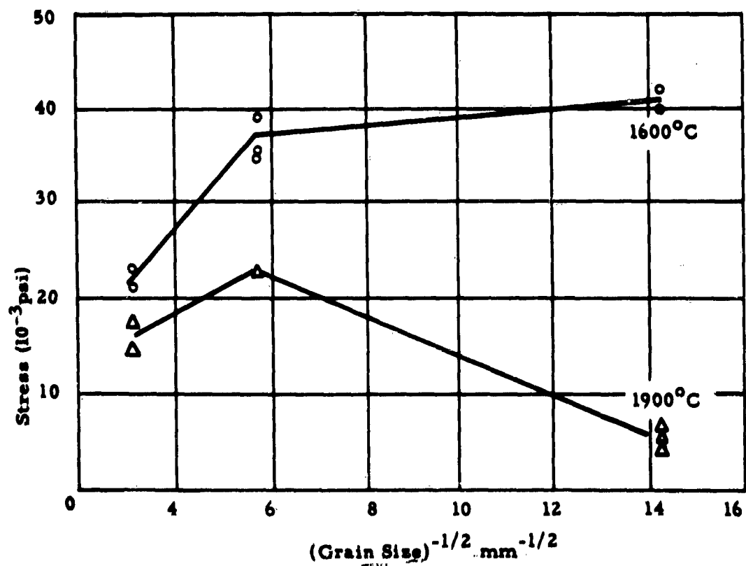
Fig. 4-20 PETCH-TYPE ANALYSIS OF THE FRACTURE STRESS-GRAIN SIZE DATA
