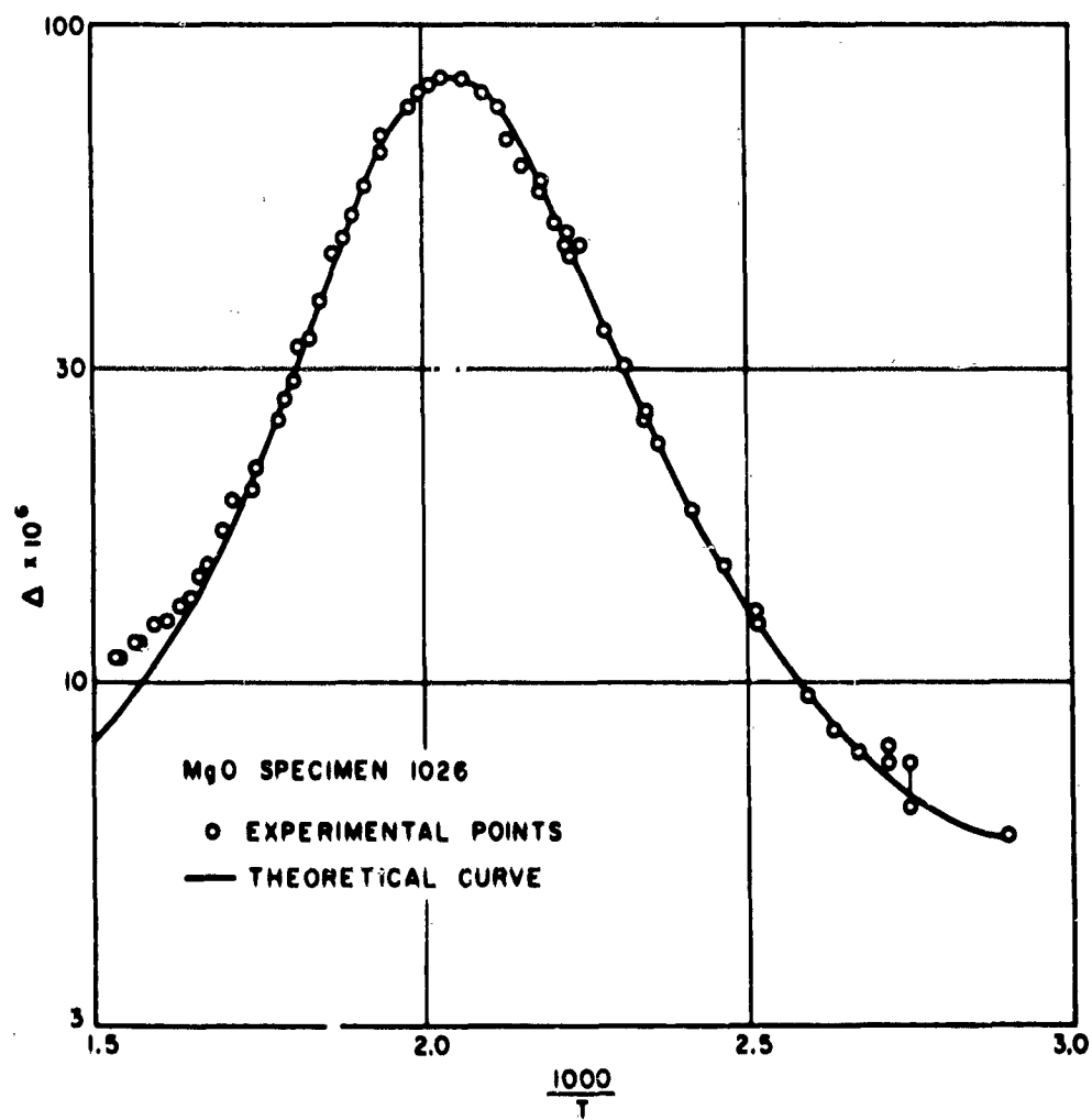
Fig. 5-23 RELAXATION PEAK OF COMPLEX AT 45 kc/s
