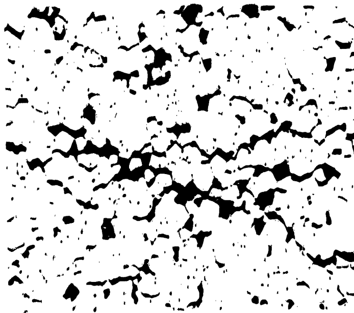
Fig. 4-10 PHOTOMICROGRAPH OF MgO SPECIMEN FRACTURED AT 1400°C X250 (Note profuse intergranular cracking)
