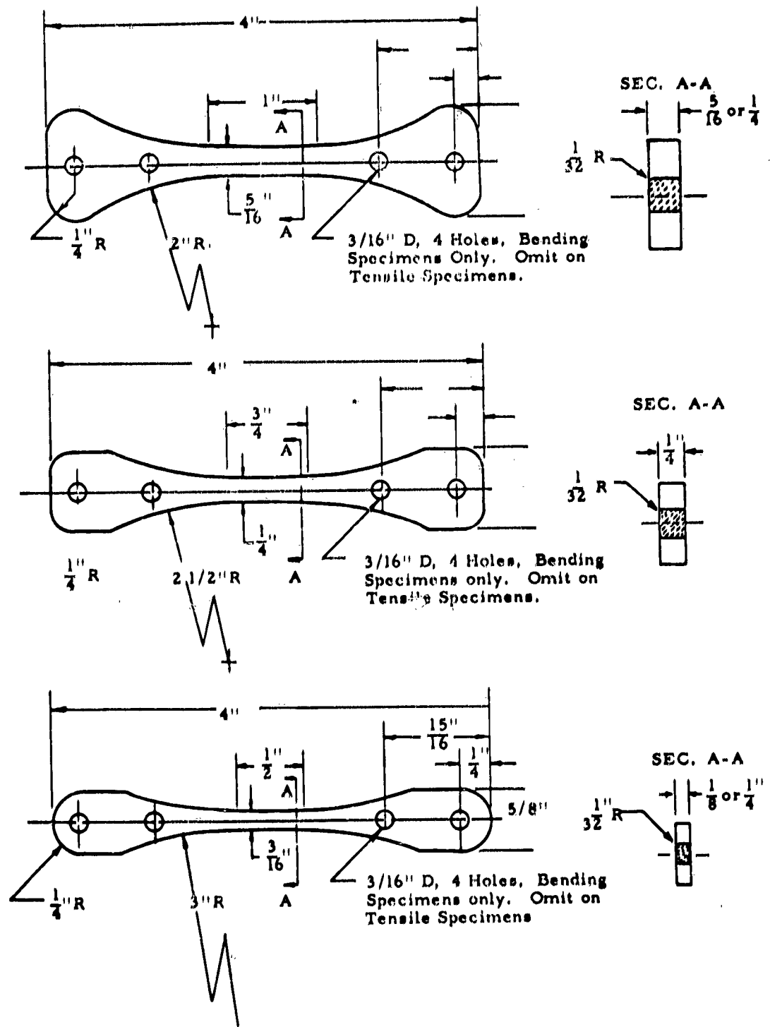
Fig. 3-2 DOGBONE USED IN TENSION BENDING TESTS
