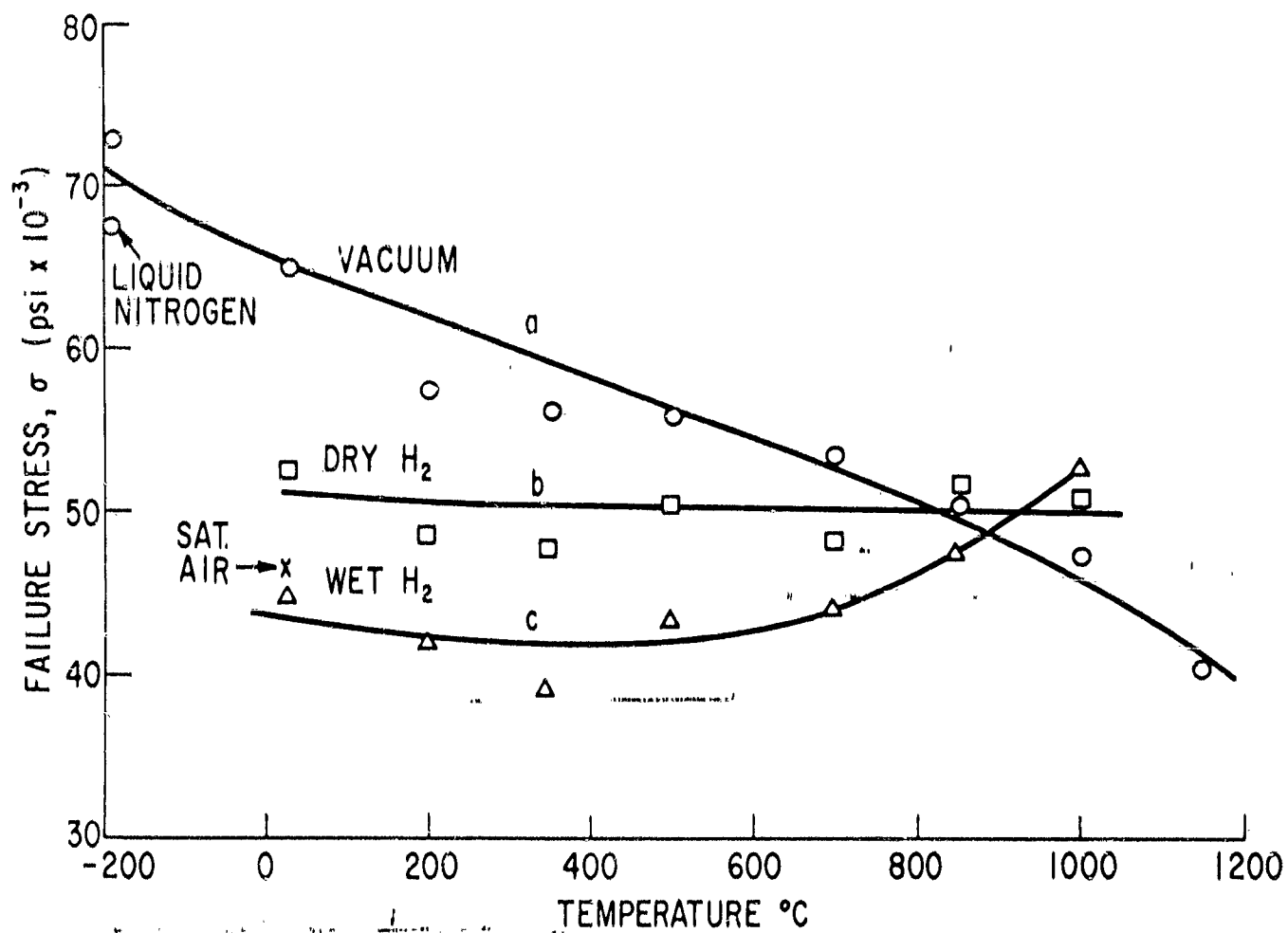
Fig. 9-12 TEMPERATURE-ENVIRONMENTAL EFFECTS ON THE RUPTURE STRENGTH OF STANDARD LUCALOX SPECIMENS
