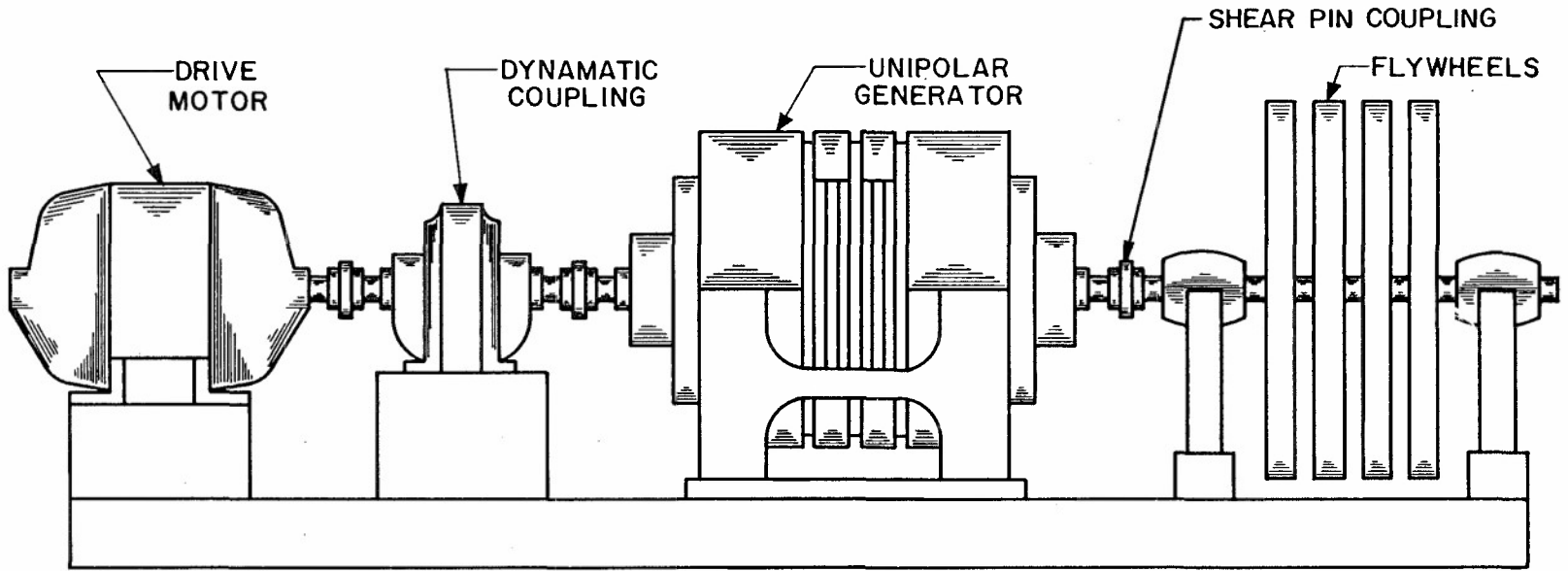
Fig. 4 Unipolar Generator Drive Unit
