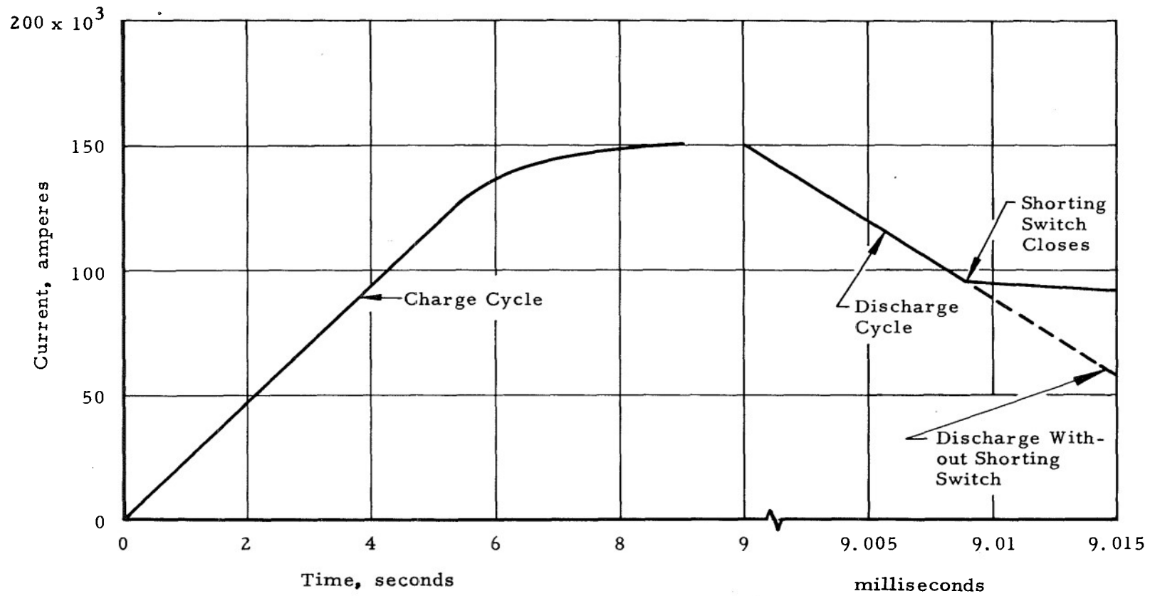
Fig. 1 Curve of Buildup and Decay of Current
