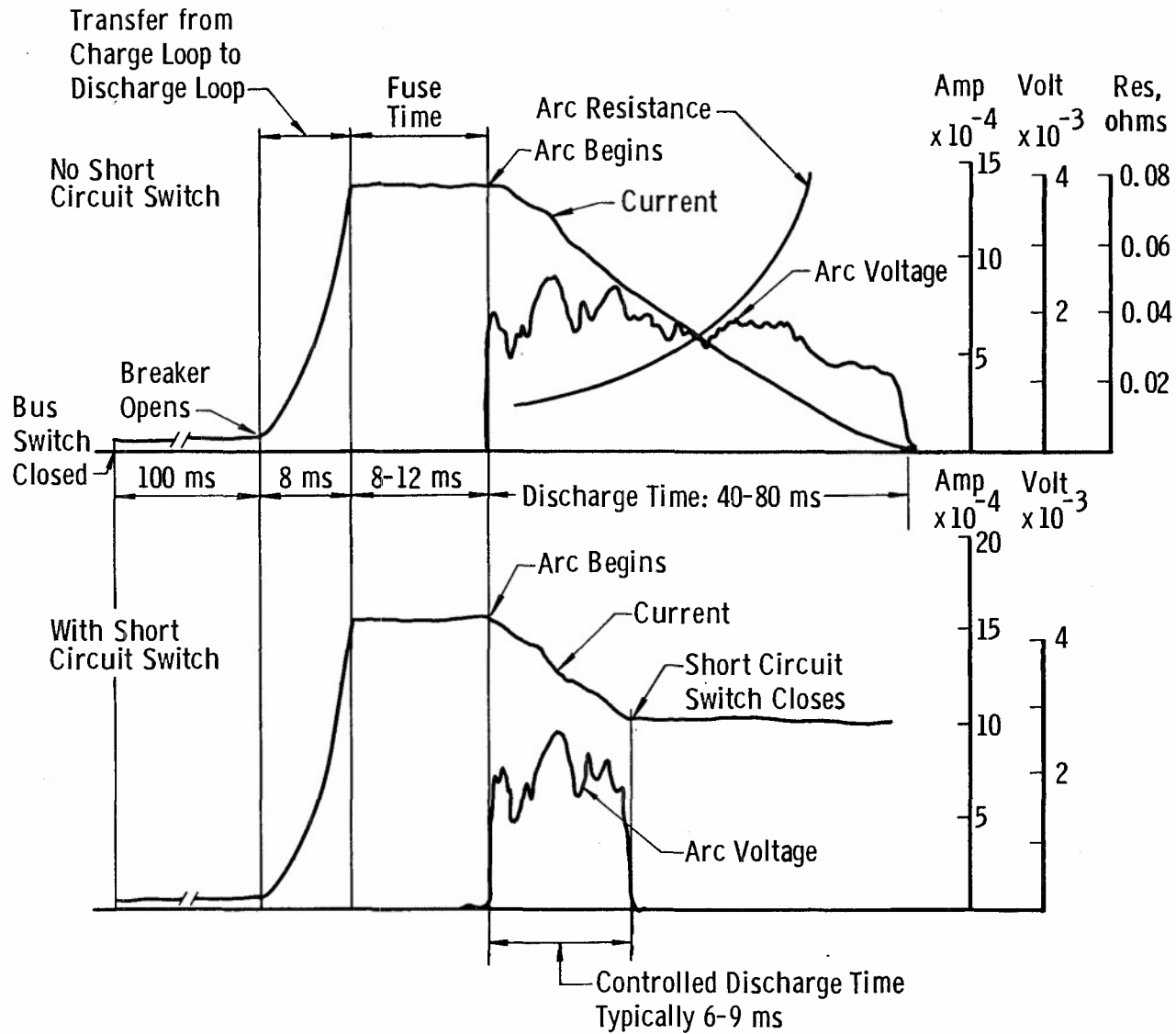
Fig. 2 Typical Current, Voltage, and Resistance Traces with and without Short Circuit Switch
