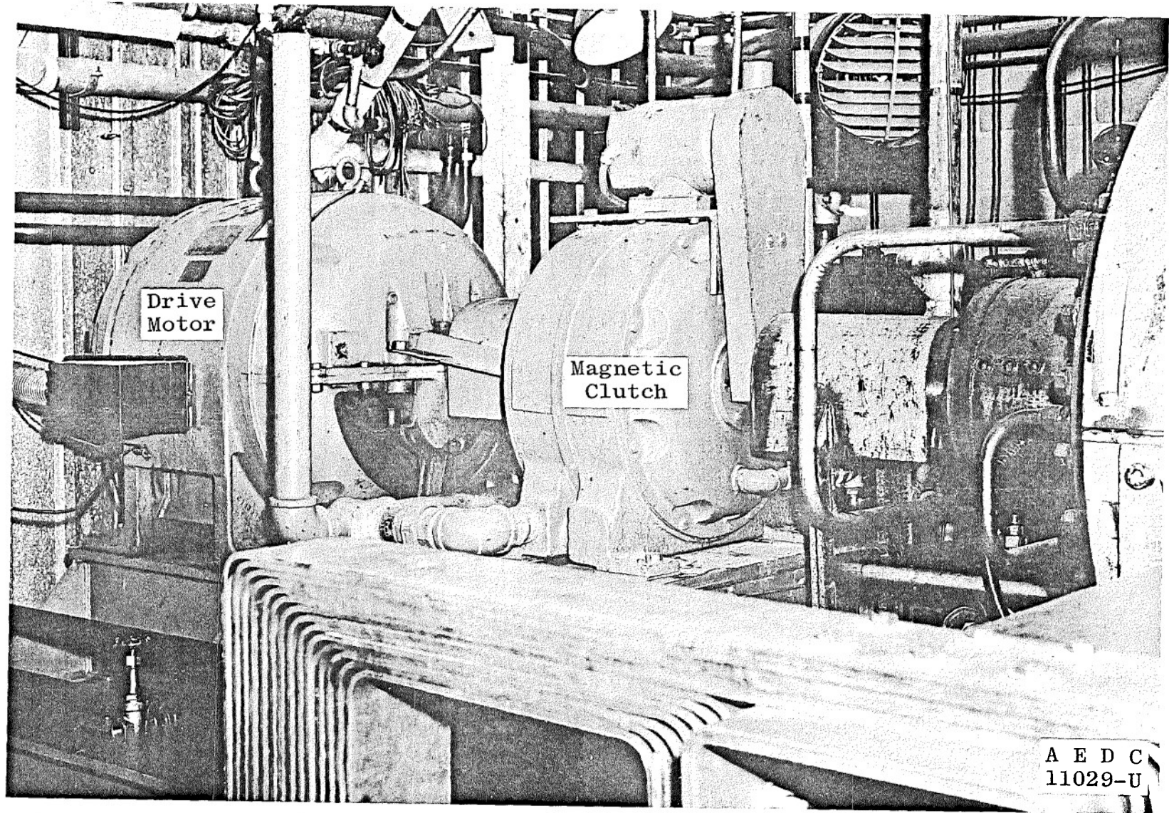
Fig. 8 Drive Motor and Magnetic Clutch
