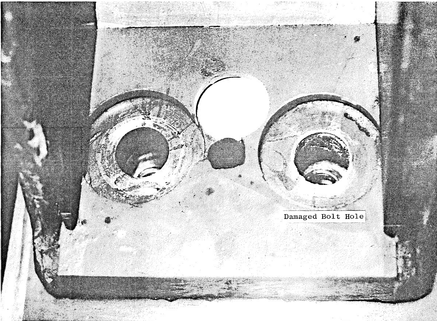
Fig. 16 Flywheel Insulation Damage
