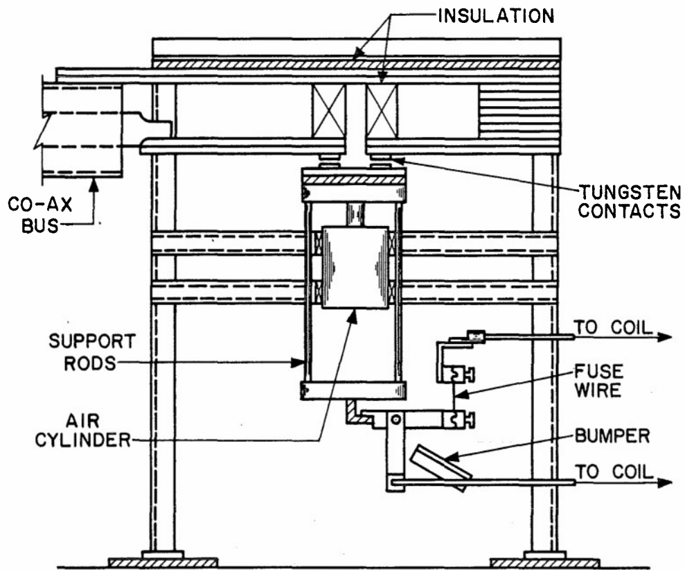
Fig. 14 Shorting Switch
