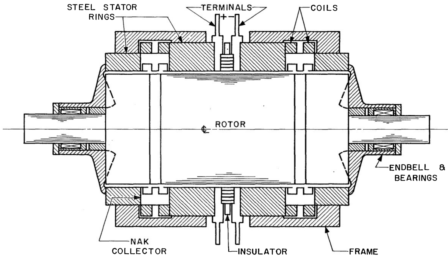
Fig. 5 Cross Section - Unipolar Generator
