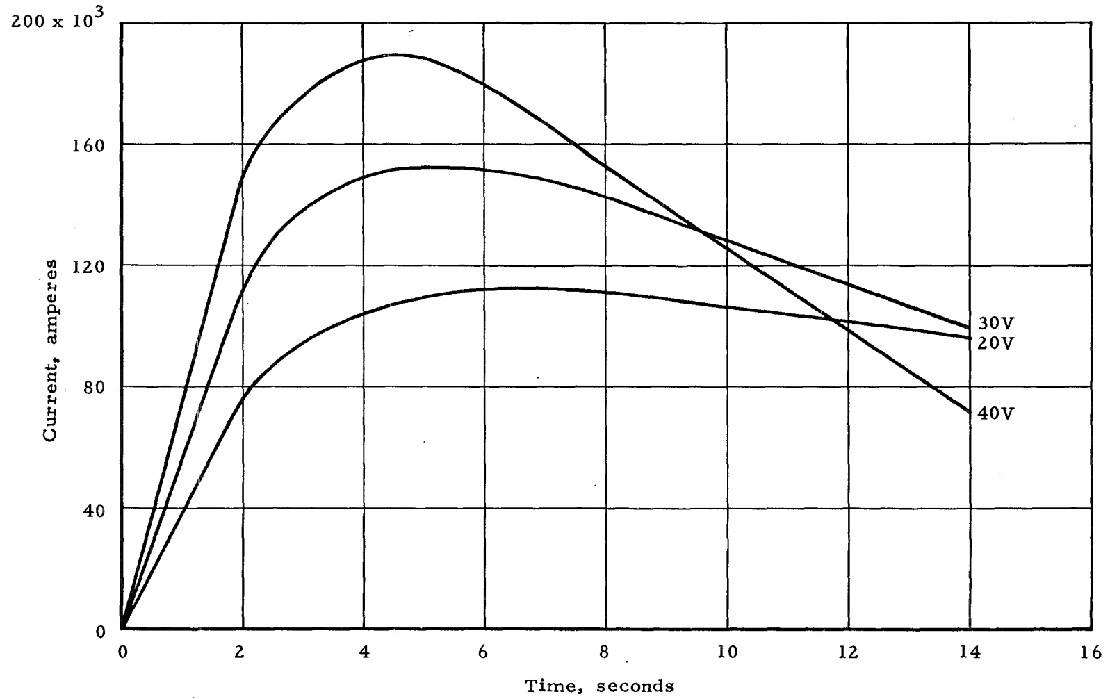
Fig. 3 Calculated Generator Performance
