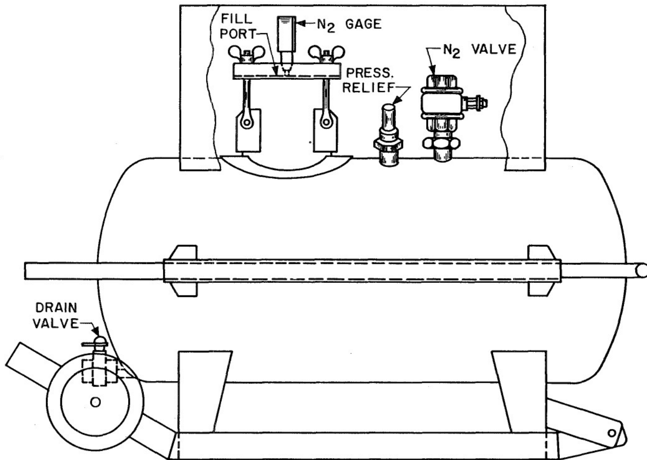
Fig. 17 NaK Transfer Tank
