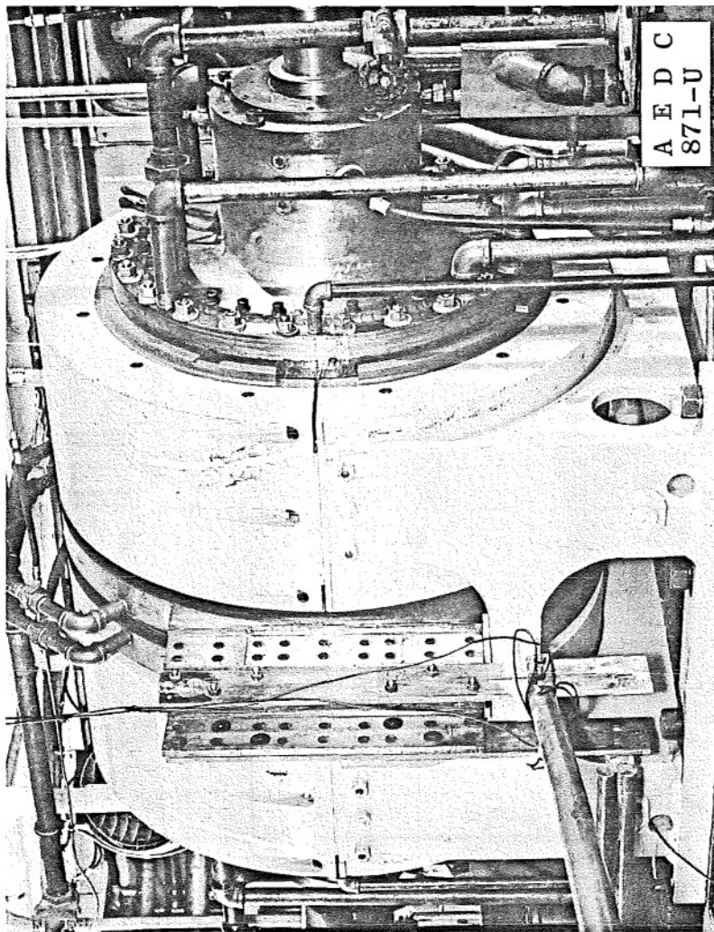
Fig. 6 Unipolar Generator
