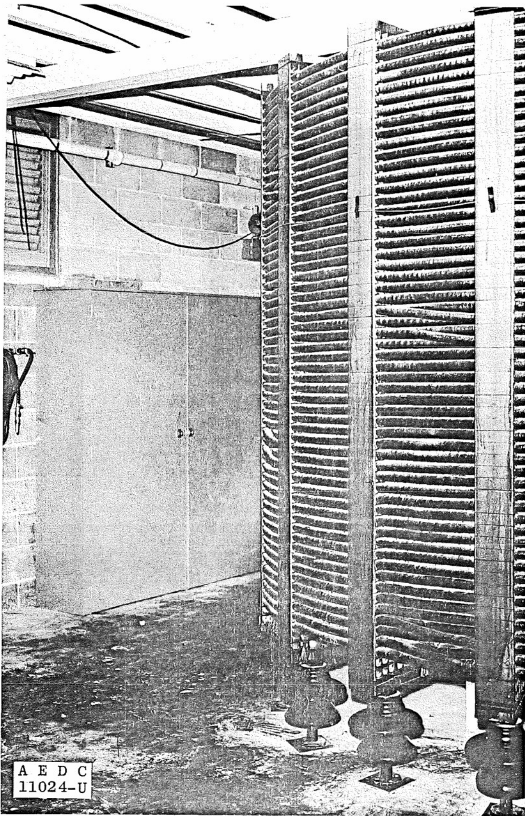
Fig. 10 Magnetic Energy Storage Coil
