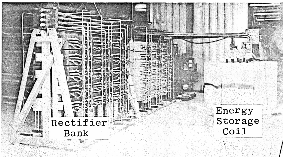
Fig. 20 Selenium Rectifier and Temporary Coil
