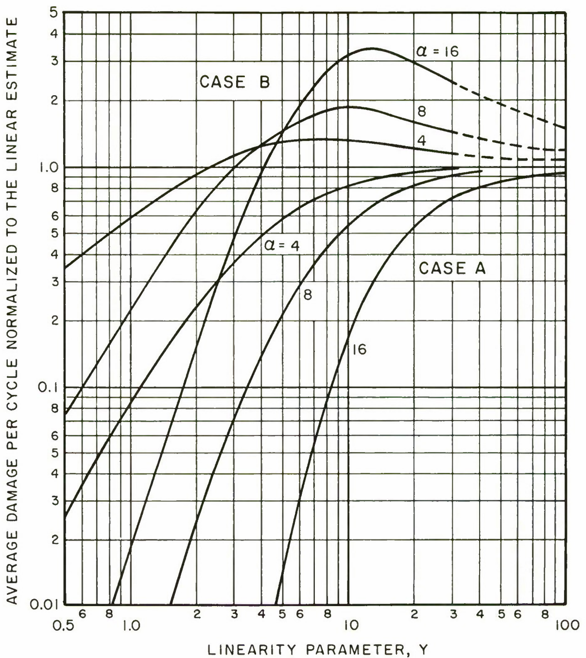
FIG. 2 AVERAGE RATE OF ACCUMULATION OF DAMAGE (PER CYCLE) IN RANDOM RESPONSE OF A HARD-SPRING RESONATOR
