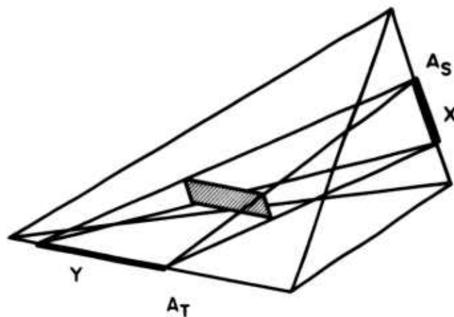
Fig. 1— Illustrating the operations X_\alpha and X
