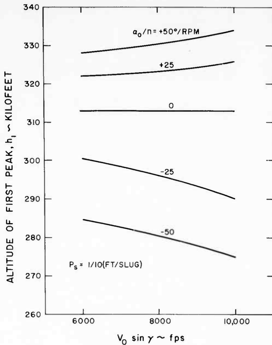
Fig. 7 Effect of descent velocity on altitude of first peak. This graph illustrates the effect of descent velocity on h_1 for various values of \alpha_0/n , assuming P_s = 1/10 .
