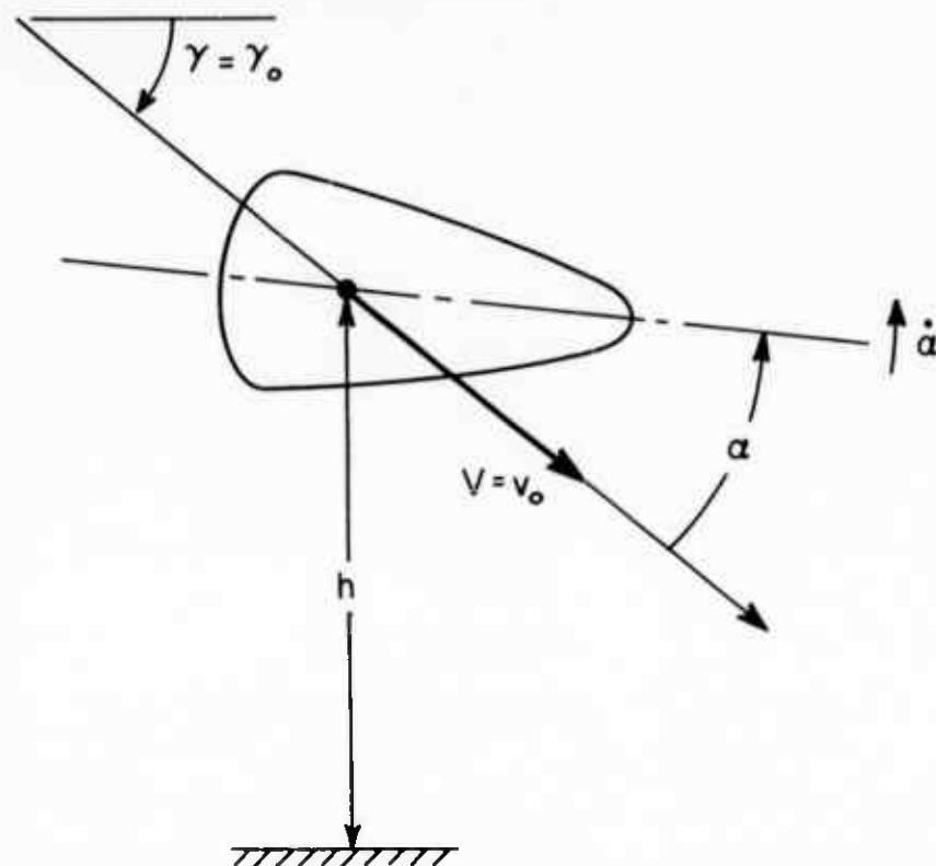
Fig. 2 Re-entry geometry.
