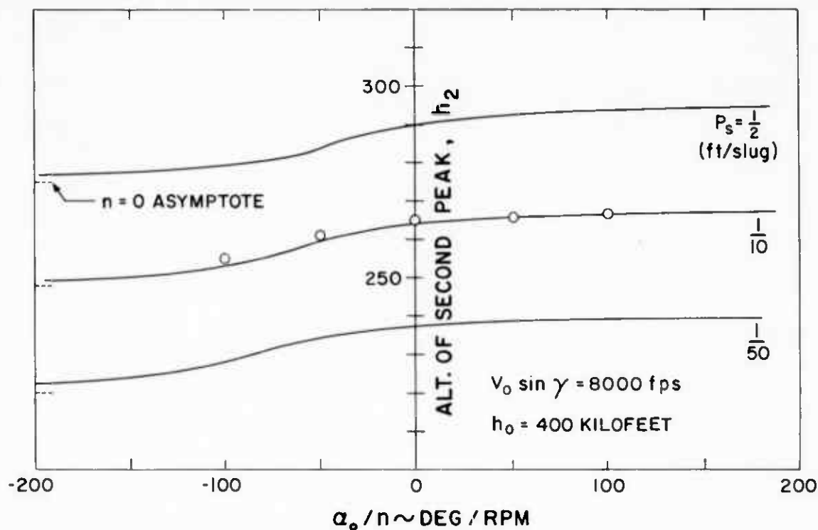
Fig. 4 Altitudes of second peak. This graph presents the altitudes at which the angle of attack rate vanishes the second time. Circles indicate results of exact integration of Eq. (1a).
