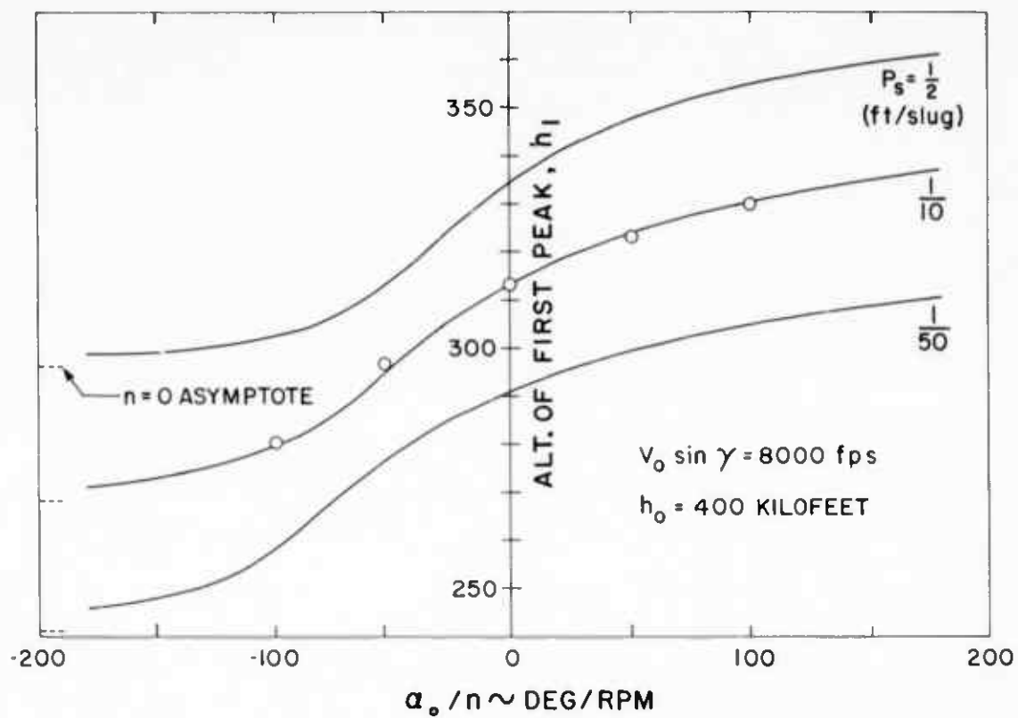
Fig. 3 Stabilization altitudes. This graph presents the altitudes of stabilization vs. (a_0/n) for various values of the stability parameter P_s . Circles indicate results of exact integration of Eq. (1a).
