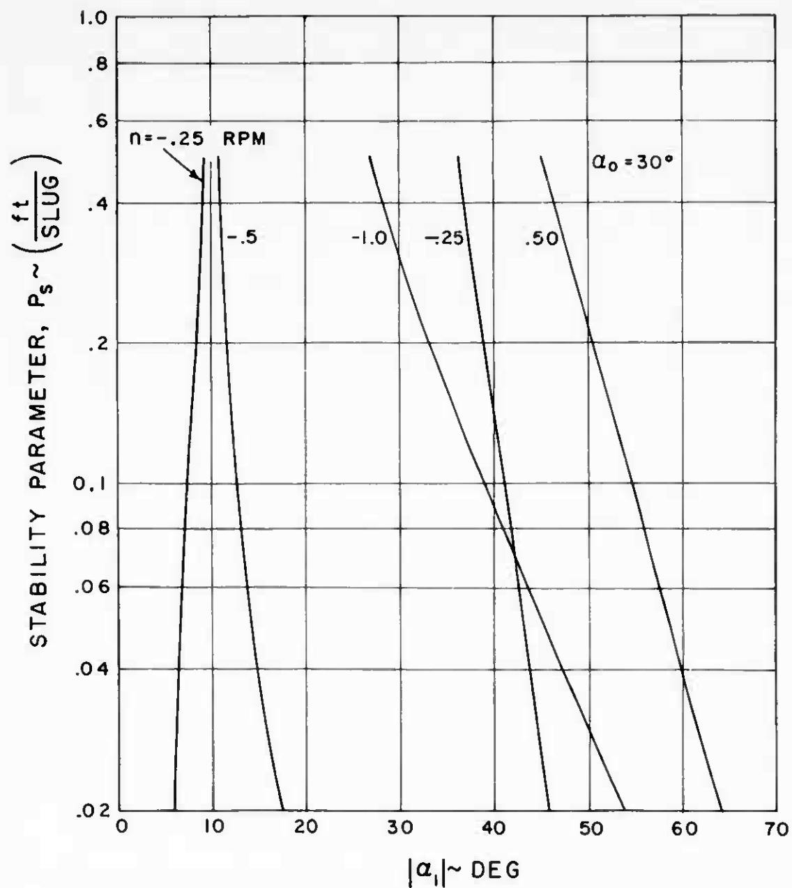
Fig. 6 Effect of stability parameter on |\alpha_1| . These curves illustrate the effect of P_s on |\alpha_1| for an initial angle of attack of 30^\circ .
