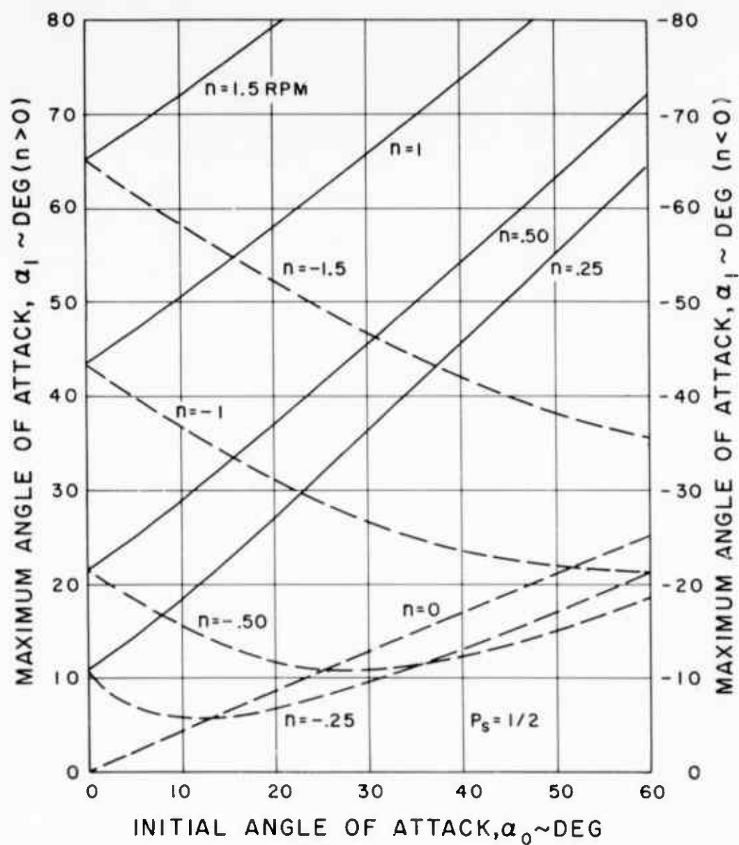
Fig. 5 Maximum angles of attack. This graph indicates the magnitude of the angle of attack at stabilization altitude as a function of initial angle of attack for P_s = 1/2 .
