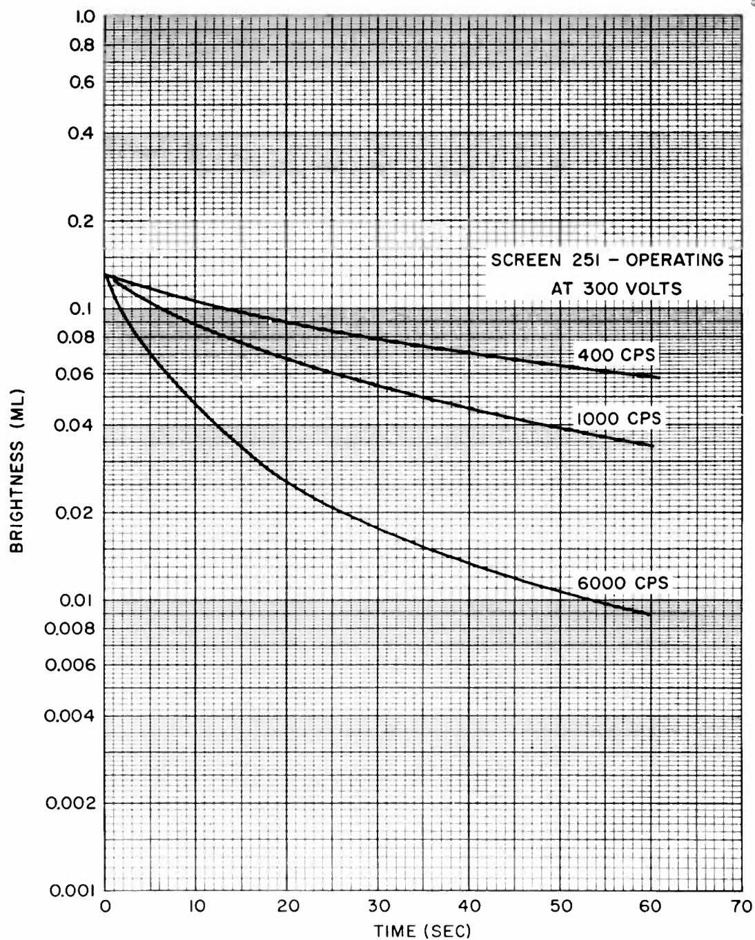
FIG. 23 DECAY CURVES FOR SCREEN 251 AT 2000 KVP
