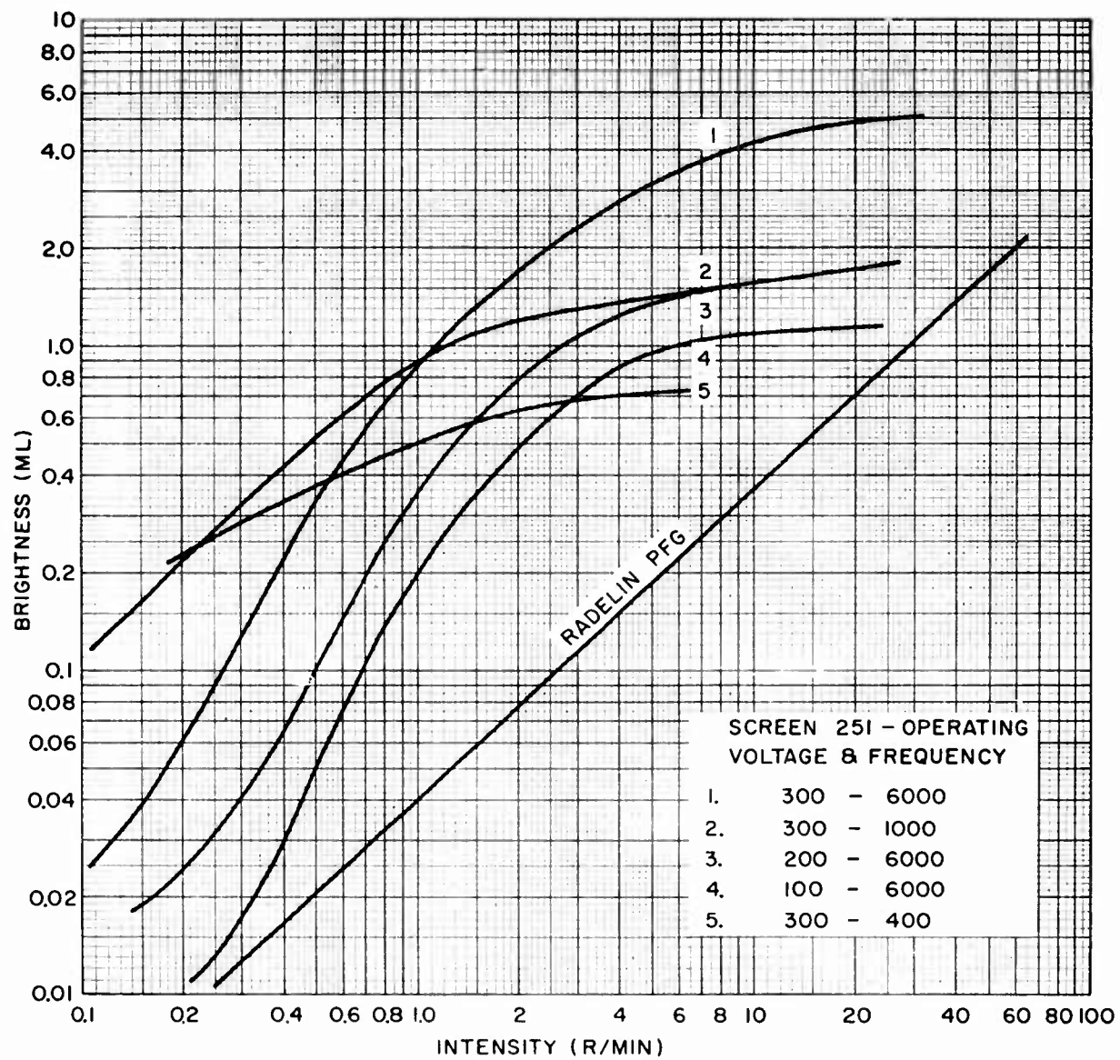
FIG. 9 BRIGHTNESS RESPONSE CURVES FOR SCREEN 251 AT 90 KVP
