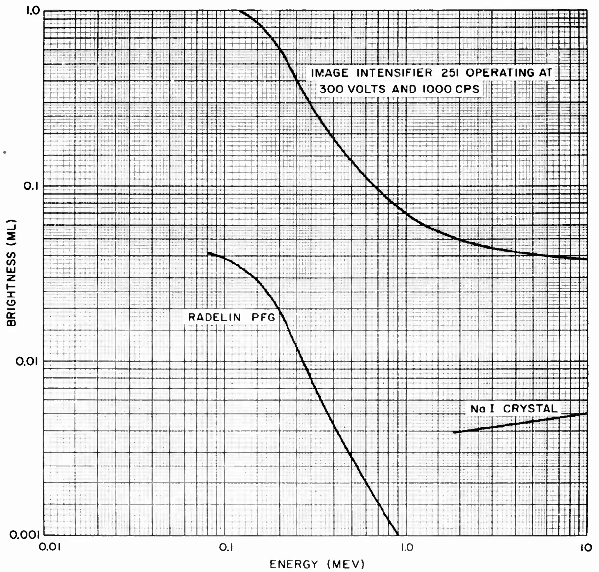
FIG. 15 BRIGHTNESS VS ENERGY FOR INTENSIFIER 251, RADELIN PFG AND NaI CRYSTAL AT 1.0 R/MIN
