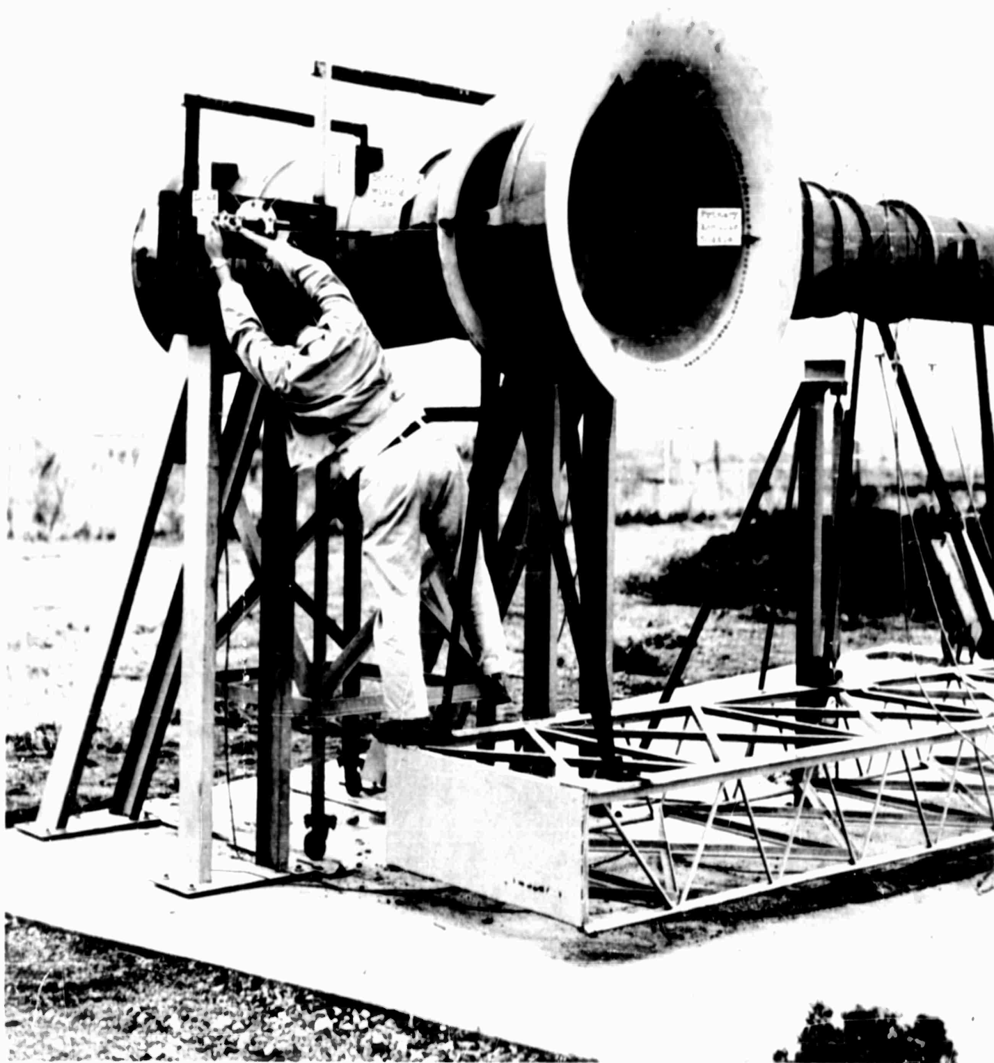
FIGURE 2: ANNULAR EJECTOR ASSEMBLY APPENDIX II
