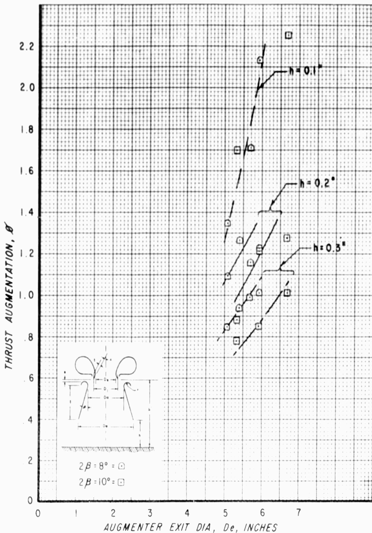
FIGURE THRUST AUGMENTATION IN GROUND EFFECT AS A FUNCTION OF AUGMENTER EXIT DIAMETER.
