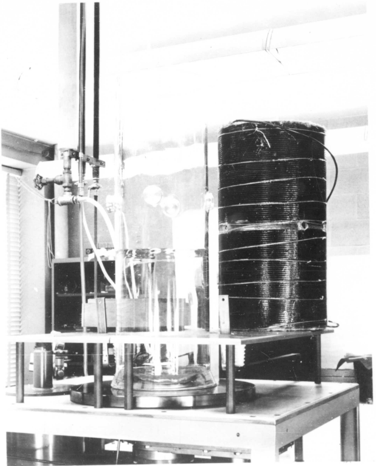
Figure 38. Vacuum Chamber.
