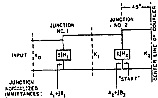
FIG. 8 EVEN- OR ODD-MODE EQUIVALENT CIRCUIT FOR DESIGN OF FOUR-BRANCH ( n = 3 ) COUPLER USED IN EXAMPLE III-1
