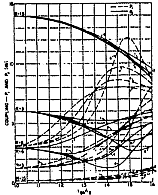
FIG. 16 COUPLING CHARACTERISTICS OF SOME MAXIMALLY FLAT COUPLERS (Impedances of these couplers are given in Tables I-1 and I-2 of Appendix I)
