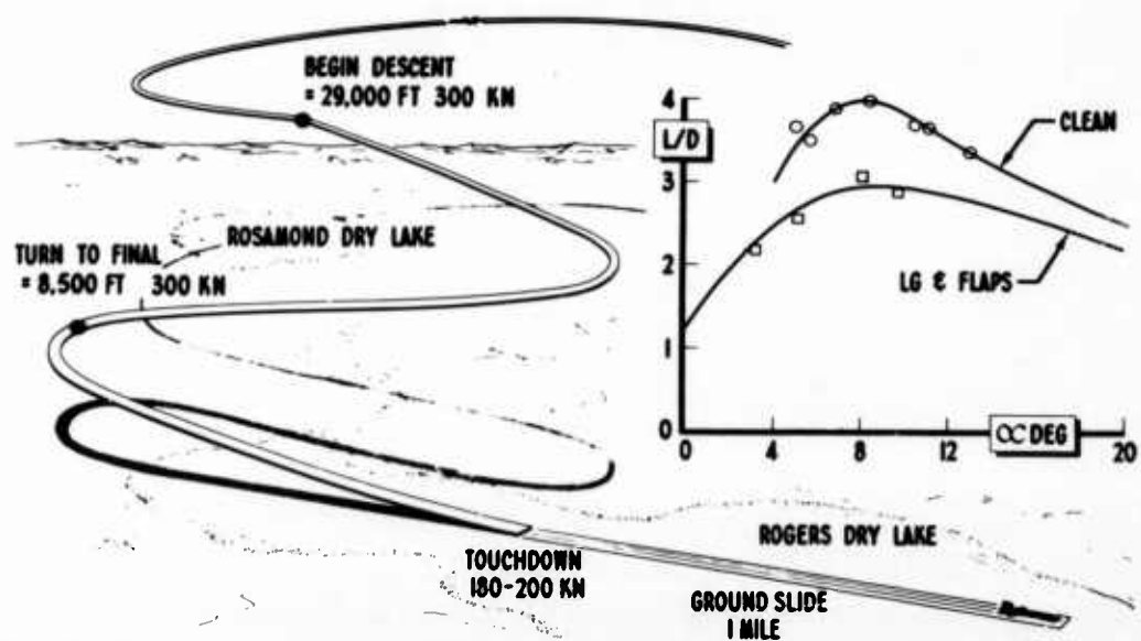
Fig.41 Landing characteristics flight test data
