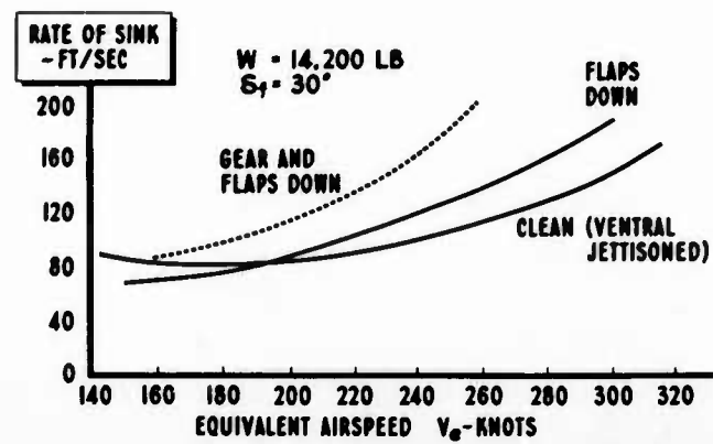
Fig.35 Rate-of-descent characteristics
