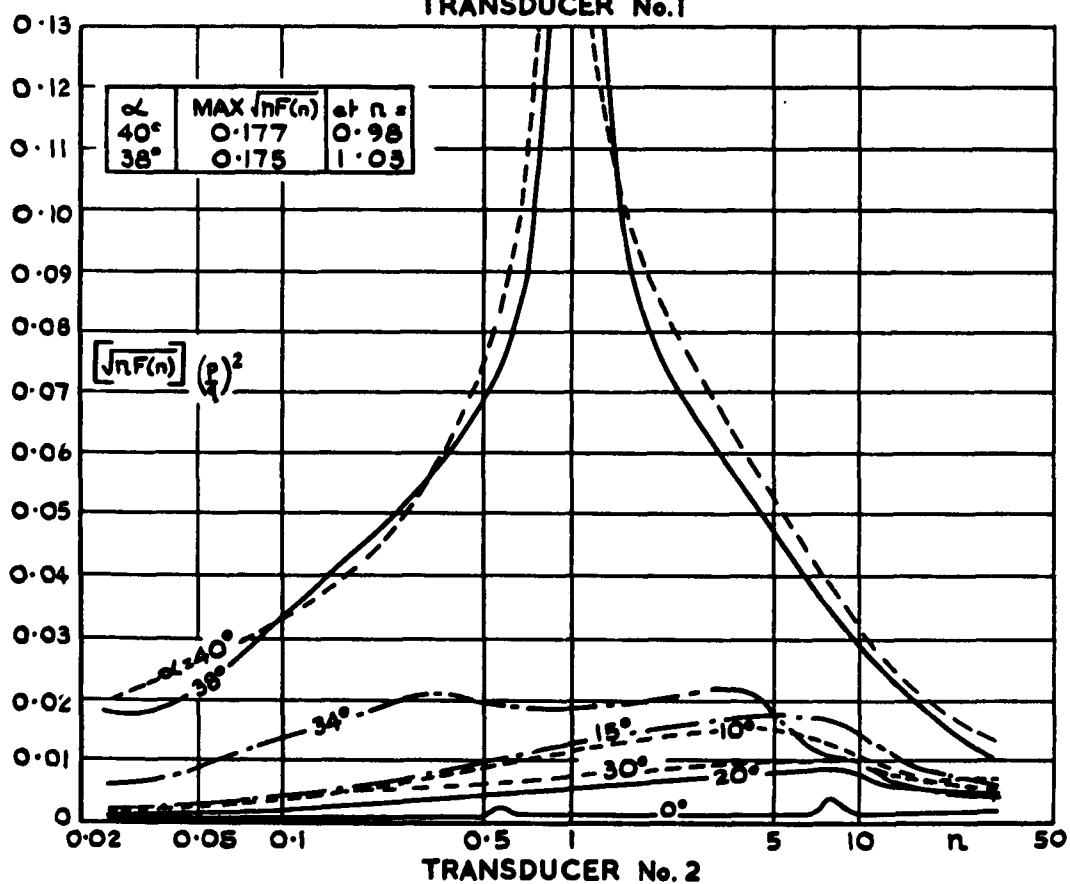
FIG. 4. SPECTRA OF PRESSURE FLUCTUATIONS.
