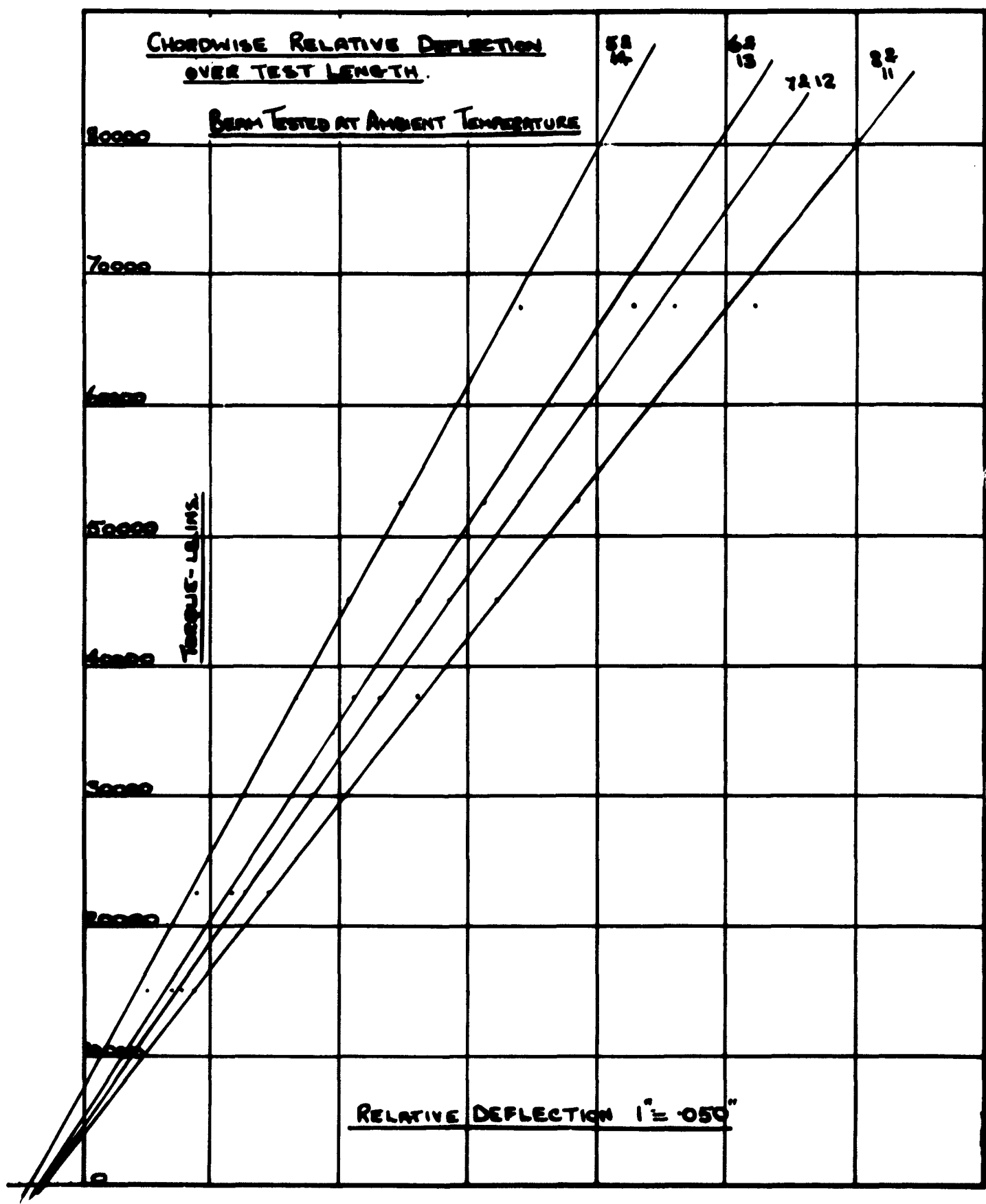
TORSION TEST ON BOX BEAMS (FIRTH VICKERS 520) SPEC. 4 | PG 18
