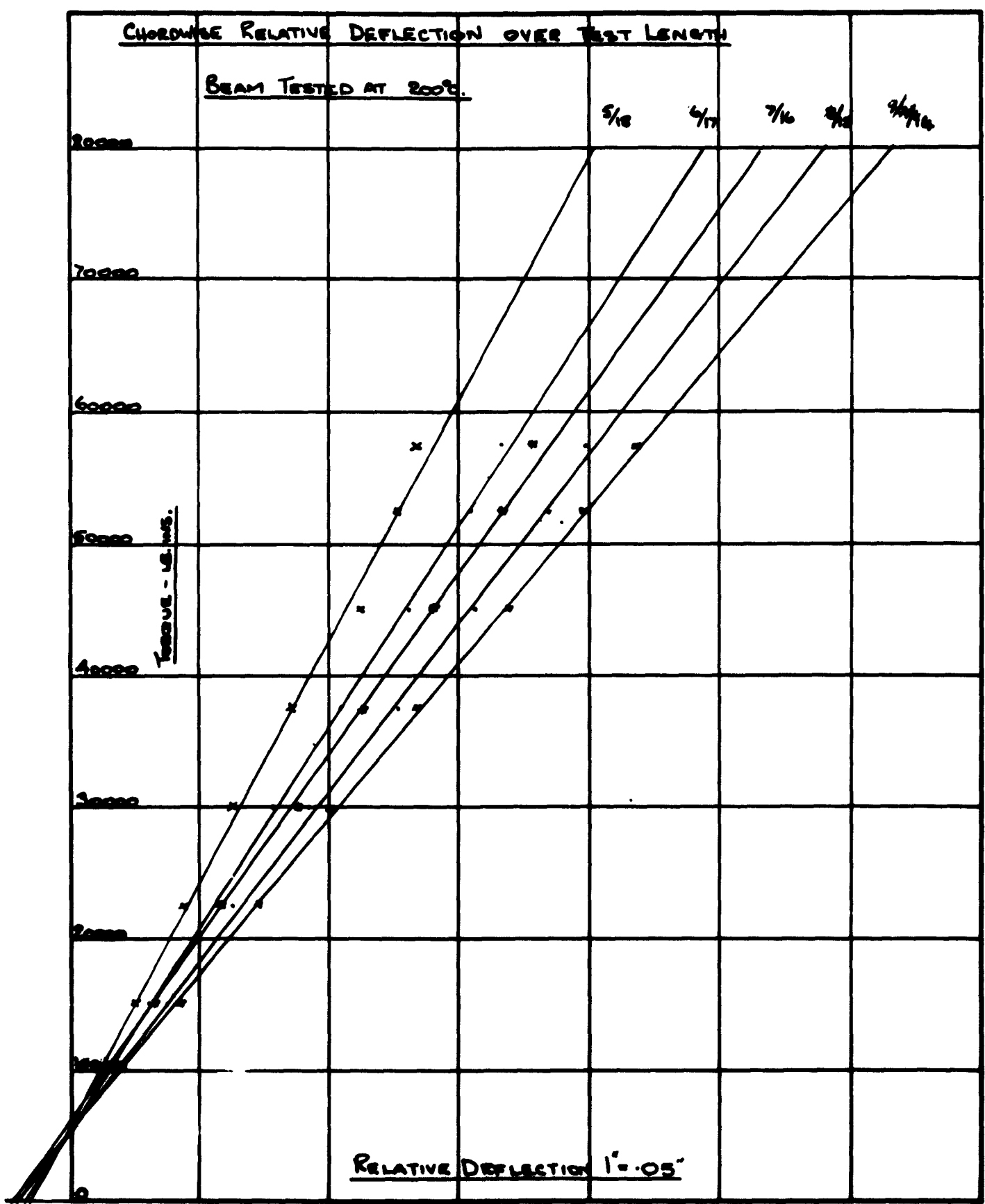
TORSION TEST ON BOX BEAMS (I.C.I. 717) SPEC. No. 8. FG. 22
