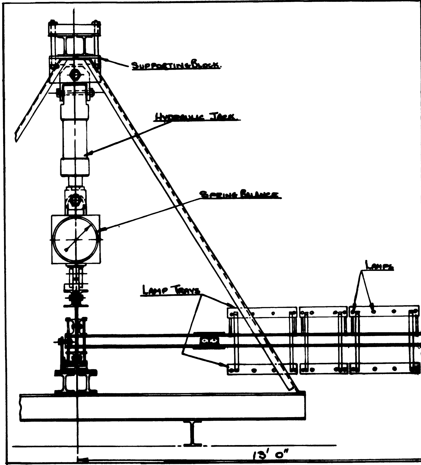
TORSION TEST RIG FOR TITANIUM & STEEL BOX
