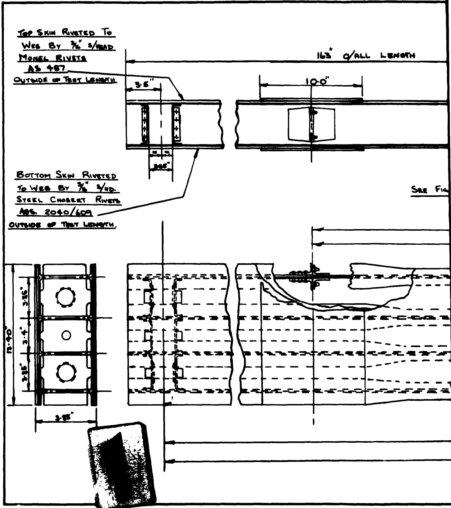
TITANIUM AND STEEL MULTIWEB BOX BEAM
