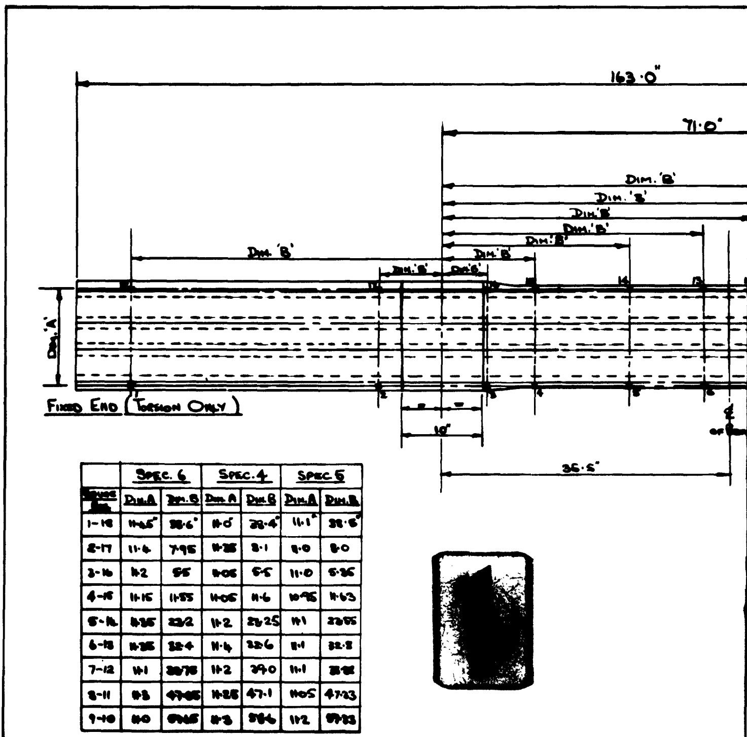
DIAL GAUGE POSITIONS FOR MULTIBES, BOX BEAMS (FIRM)
