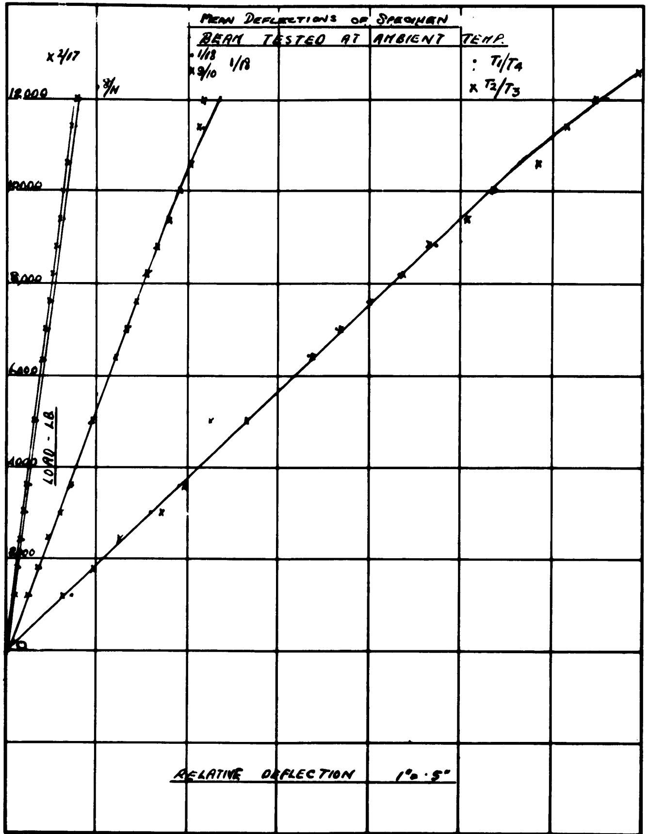
BENDING TESTS ON BOX BEAM (1U 317) SPEC 7
