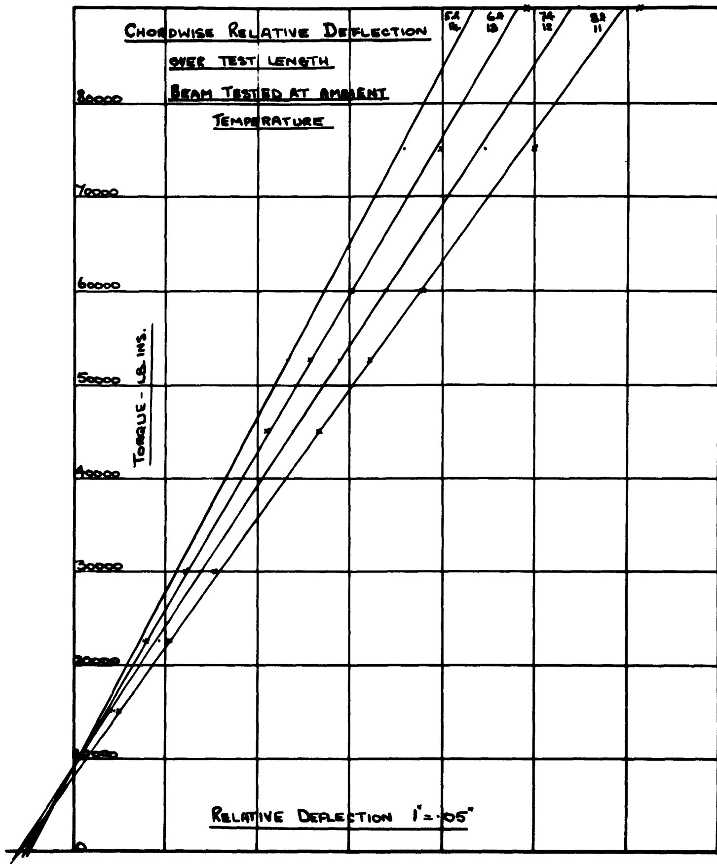
TORSION TEST ON BOX BEAMS (D.T.D. 146) SPEC. 1. FG. 15
