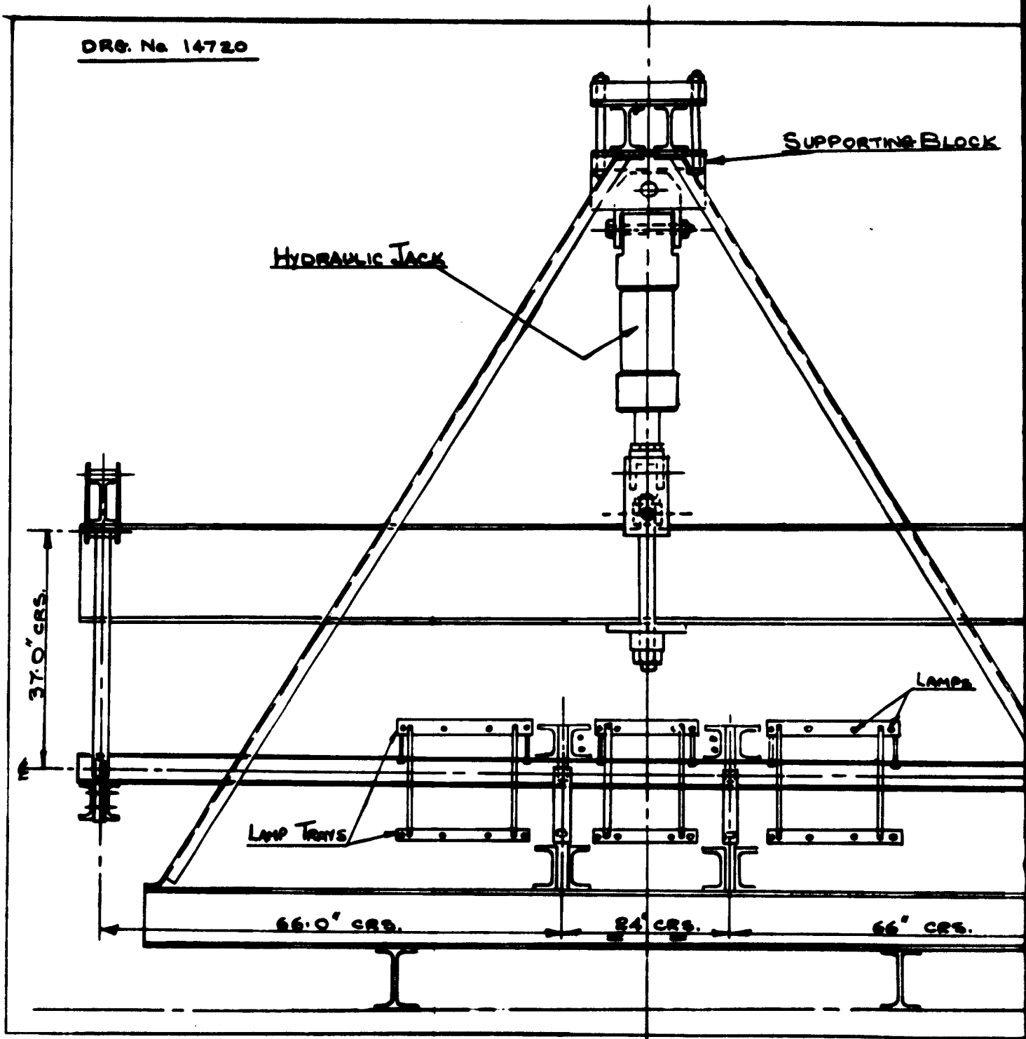
BENDING TEST RIG FOR TITANIUM & STEEL BOX BEAM
