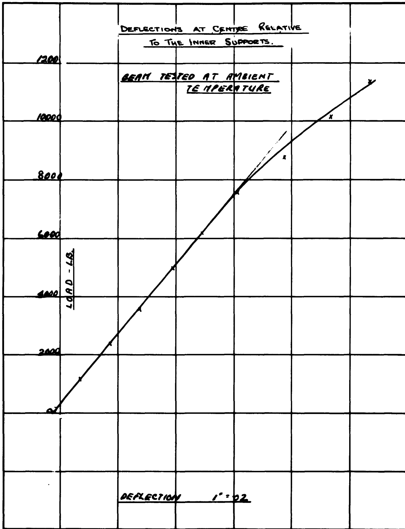
BENDING TEST ON BOX BEAM (DTD 166) SPEC N°1 FIG. 52
