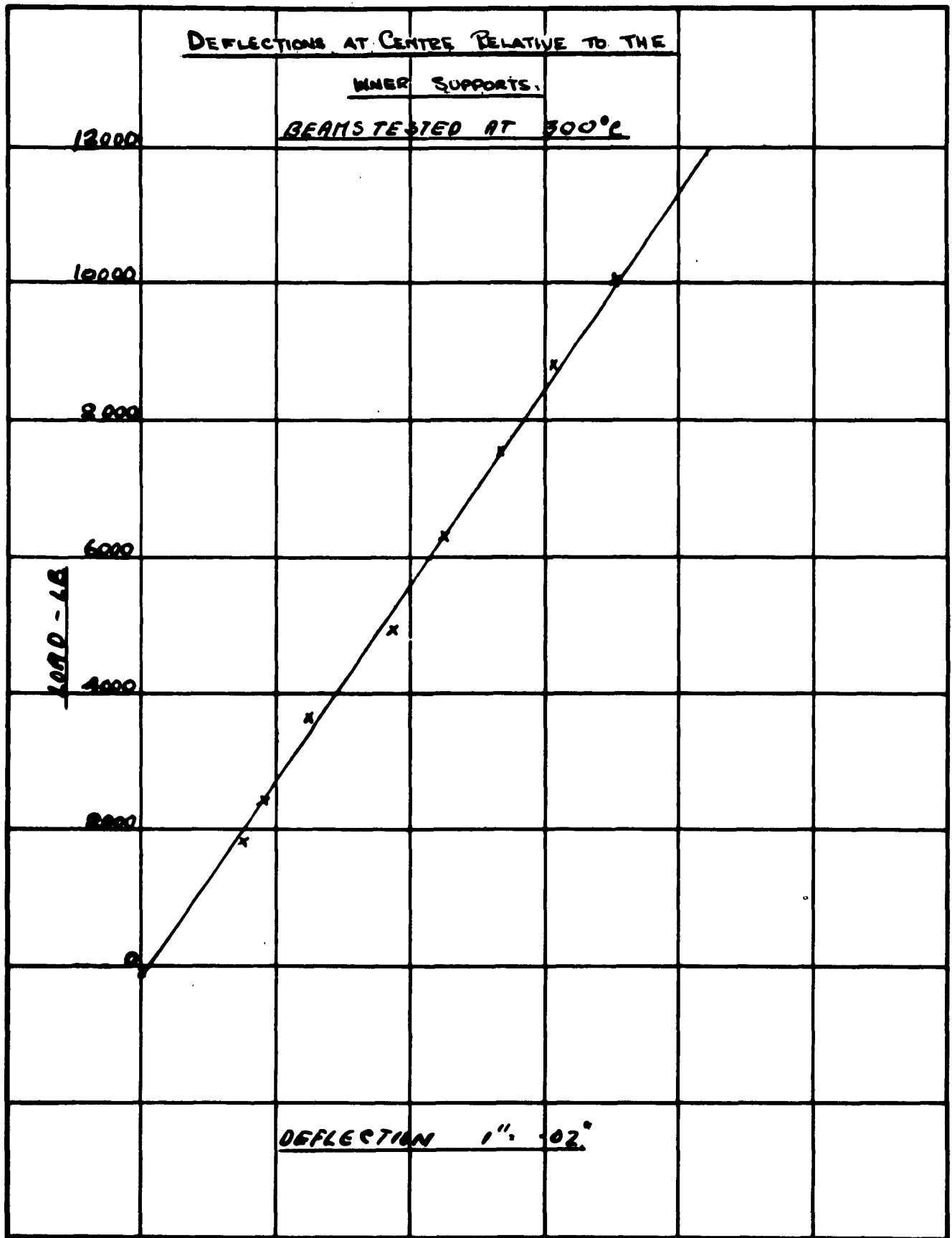
BENDING TEST ON BOX BEAM (FIRM VICKERS S20) SPEC N° 6 FIG. 54
