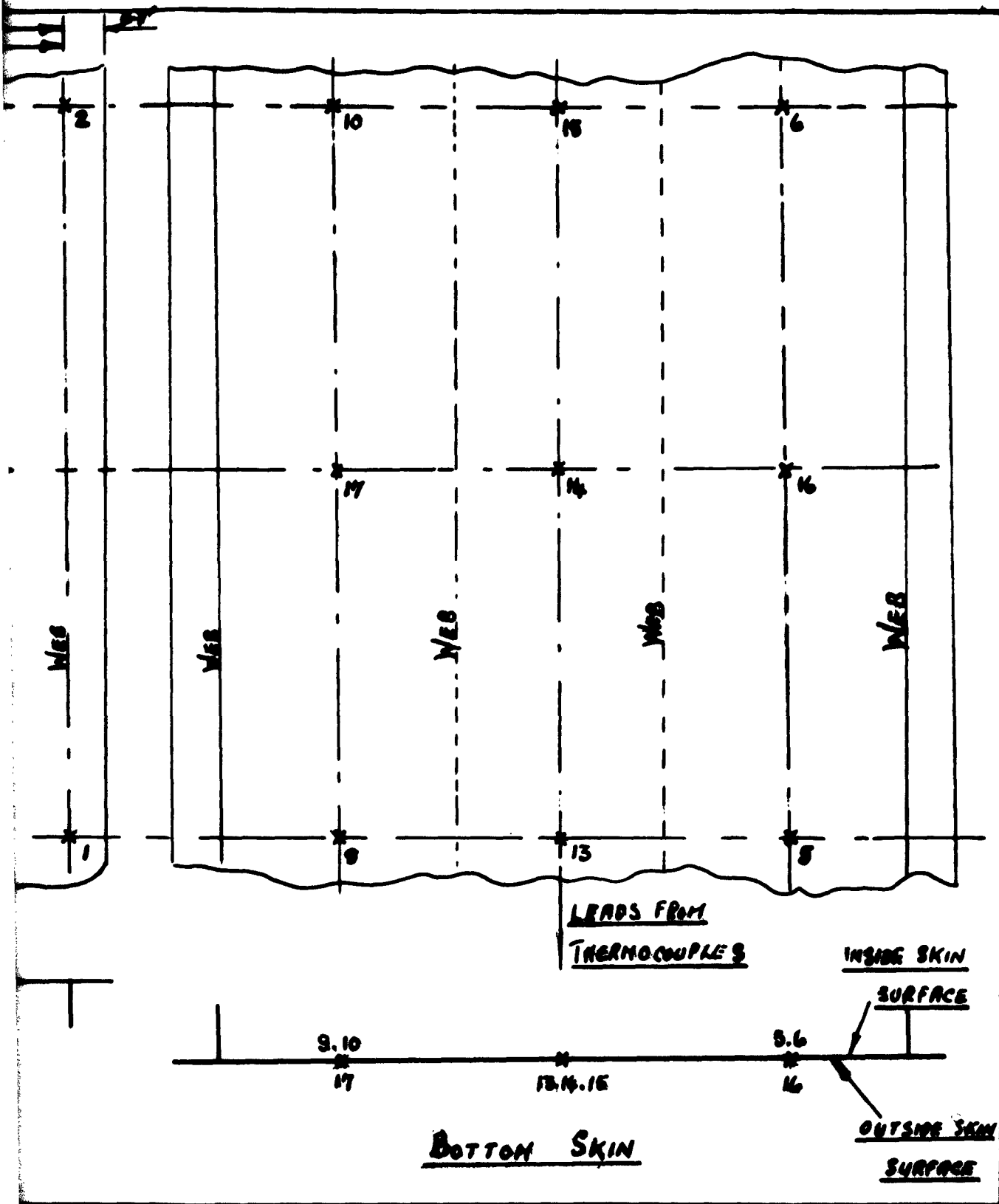
BOX BEAMS (D.T.O.166) SPEC 3 (FY 520) SPEC 5+6 SEE TABLES A + F FIG. FOR BEAM TEMPERATURES ↑
