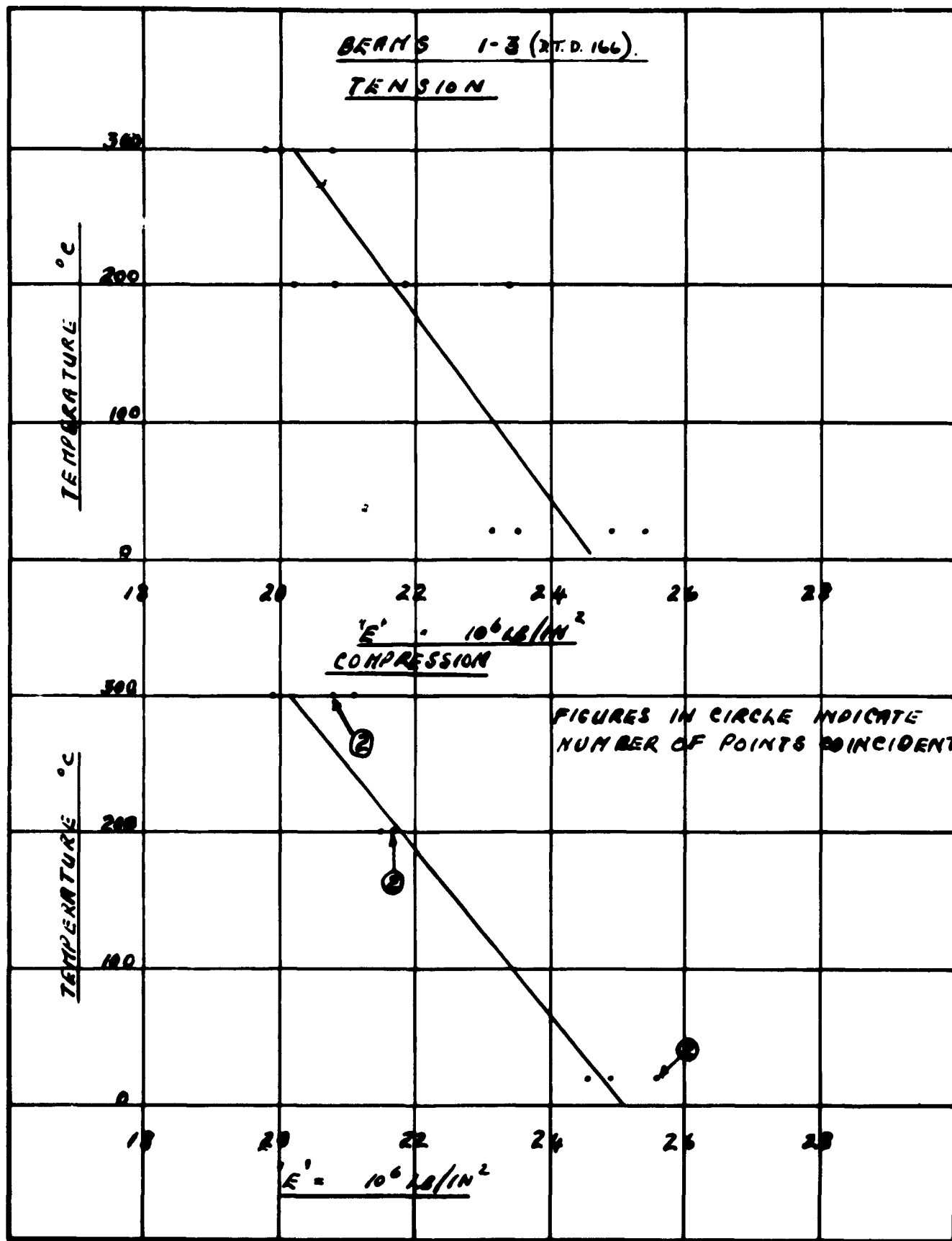
VARIATION OF 'E' WITH TEMPERATURE FIG. 76
