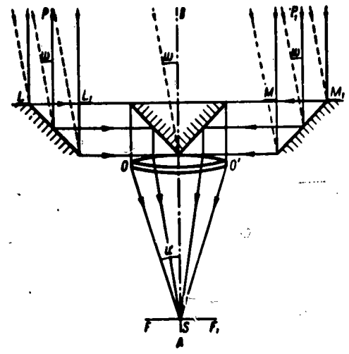
Fig. 20. Optical device for "amplifying" the illumination.
