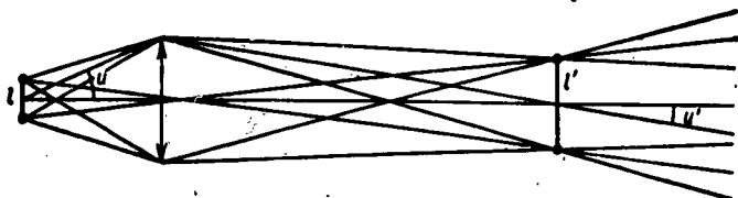
Fig. 6. Structure of an image.
