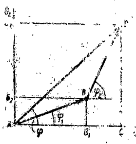
Fig. 58. Vector addition of light oscillation amplitudes.
