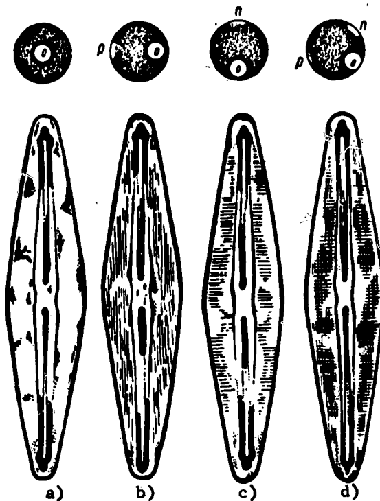
Fig. 43. Armor of the diatom Frusturia Rhomboides var. Saxonica , observed at different positions of the condenser diaphragm.
