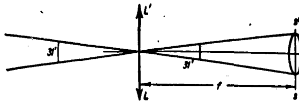
Fig. 2. Image of the sun projected through a lens
