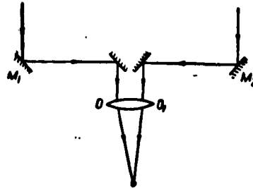
Fig. 46. Michelson's arrangement for determining the angular diameter of stars.
