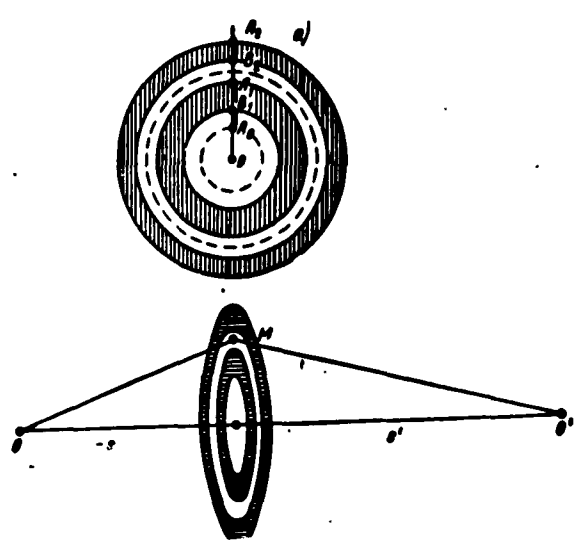
Fig. 66. Structure of Soret zone plate
