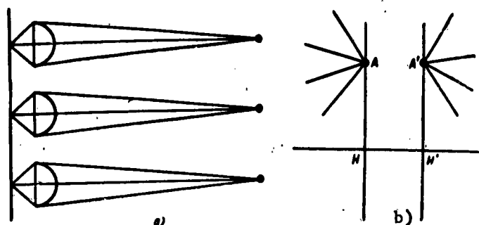
Fig. 15. Conversion of diffused into directed light.
