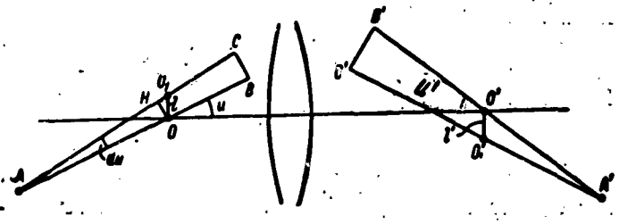
Fig. 7A Proof of the Lagrange-Helmholtz law.
