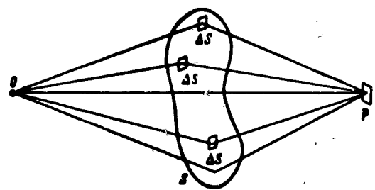
Fig. 31. Huygens-Fresnel principle.
