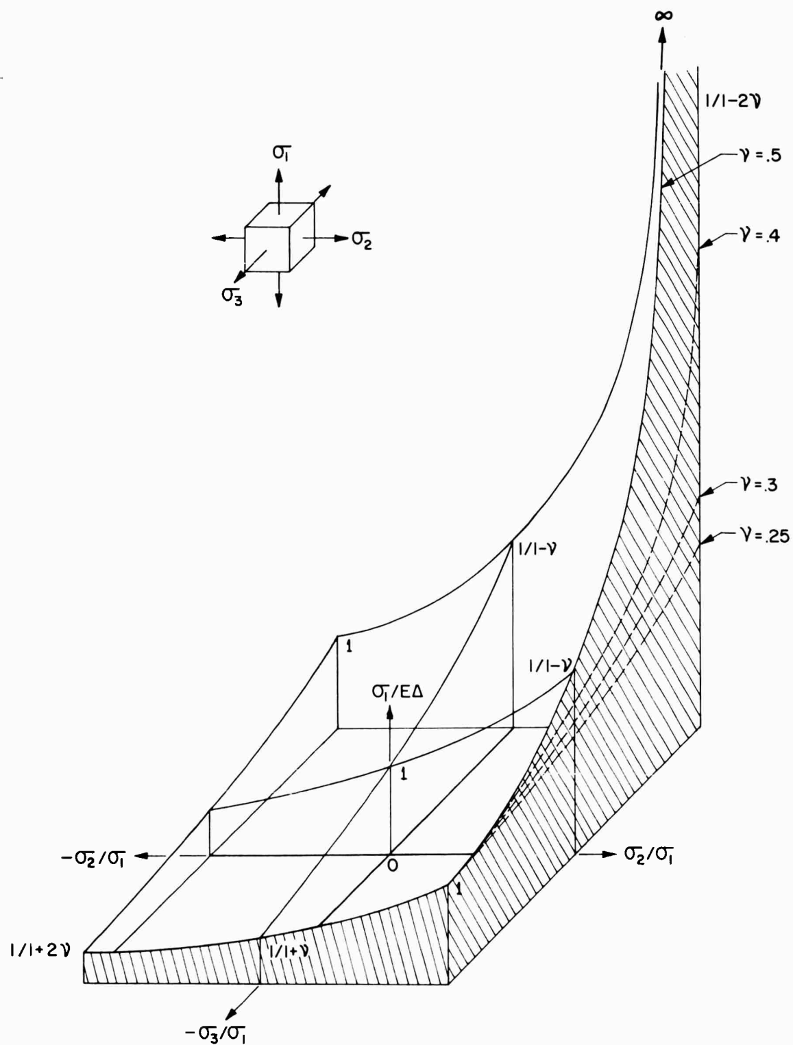
Figure 78. Variation of Restrained Thermal Contraction Stress With Lateral Restraint and Poisson's Ratio
