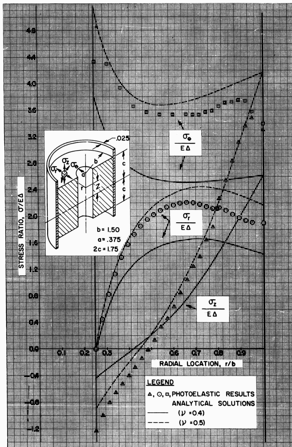
Figure 104. Stress Distribution on the Plane of Symmetry, Z = 0 , in a Case-Bonded Cylindrical Bore Grain Subjected to Thermal Cycling Stresses
