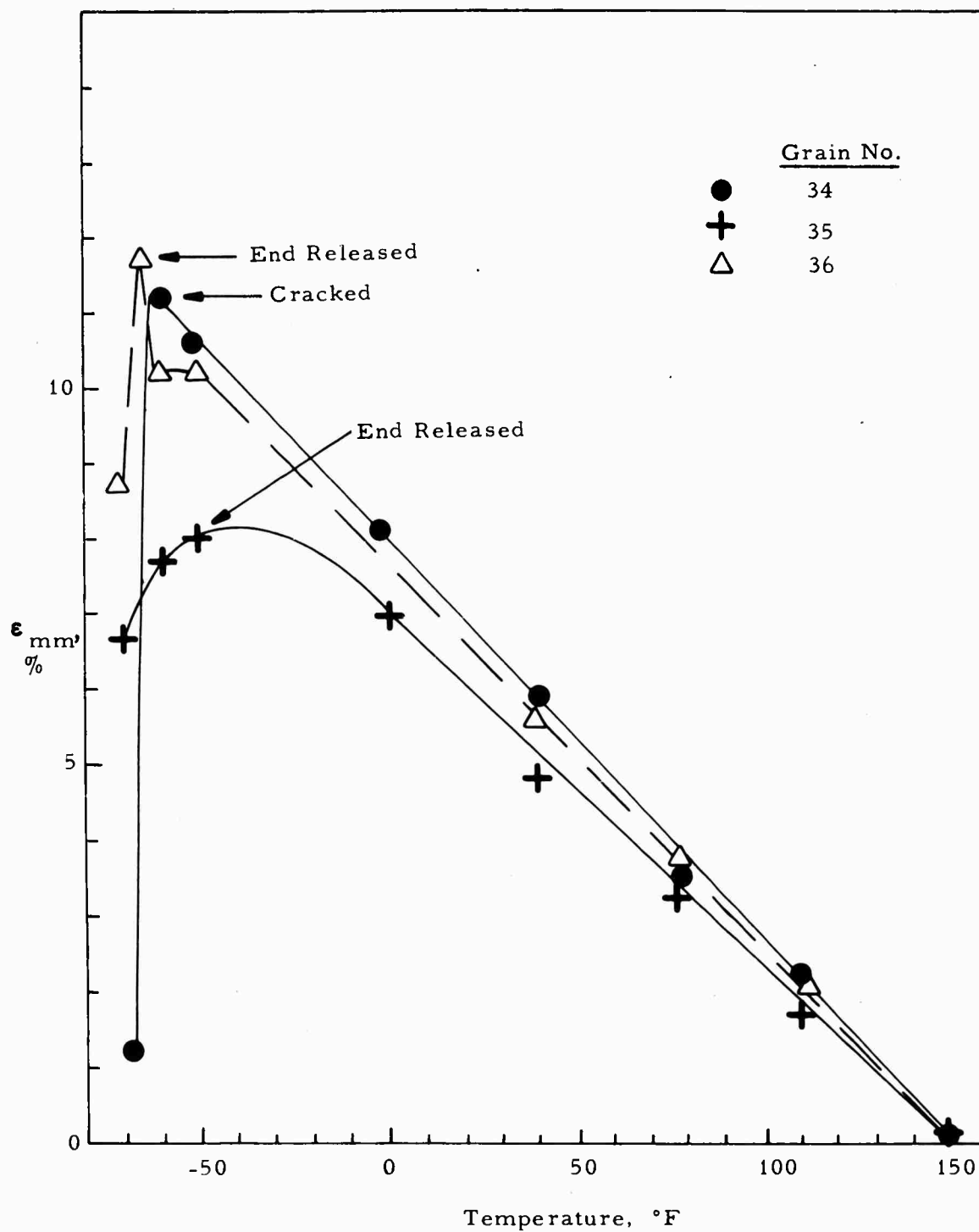
Figure 56. The Effect of Temperature on Maximum Bore Strain for PDB Propellant at B/A = 4 , L/B = 3.2
