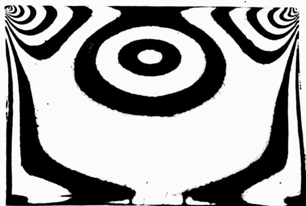
PHOTOELASTIC FRINGE PHOTOGRAPH
