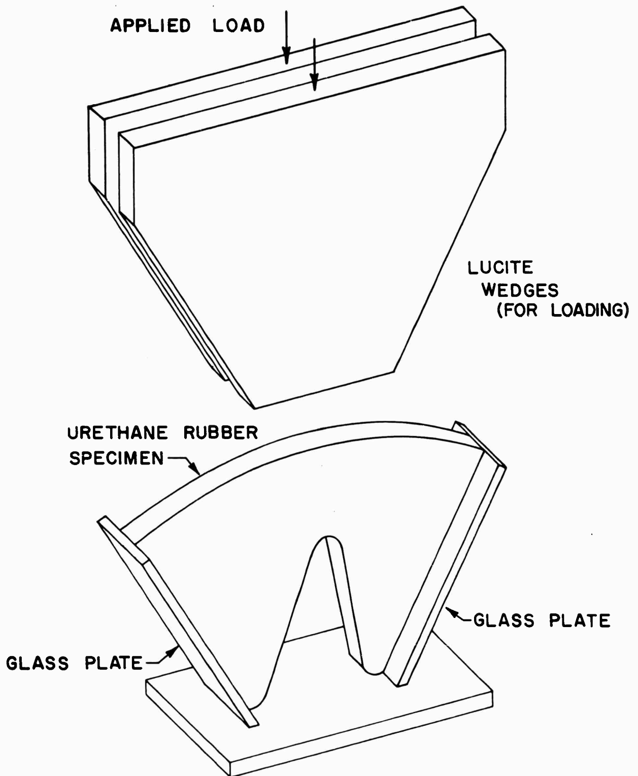
Figure 107. Loading Method
