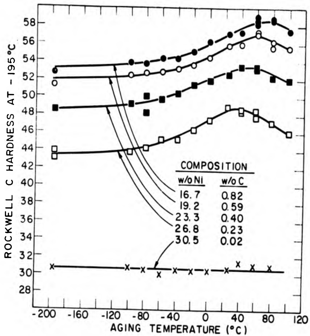
Fig. 8 Rockwell C Hardness of Iron - Nickel - Carbon Martensites as Measured at -195^{\circ}\text{C} after Aging for Three Hours at the Temperatures Shown.
