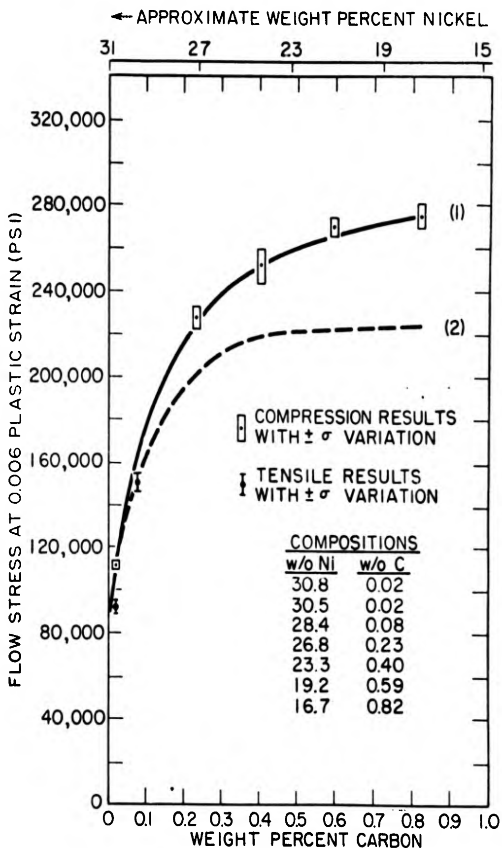
Fig. 6 Flow Stress (0.006 Plastic Strain) for 100 Percent Martensite at 0°C. Curve (1) - Experimental, Aged 3 Hours at 0°C. Curve (2) - Corrected for Aging.
