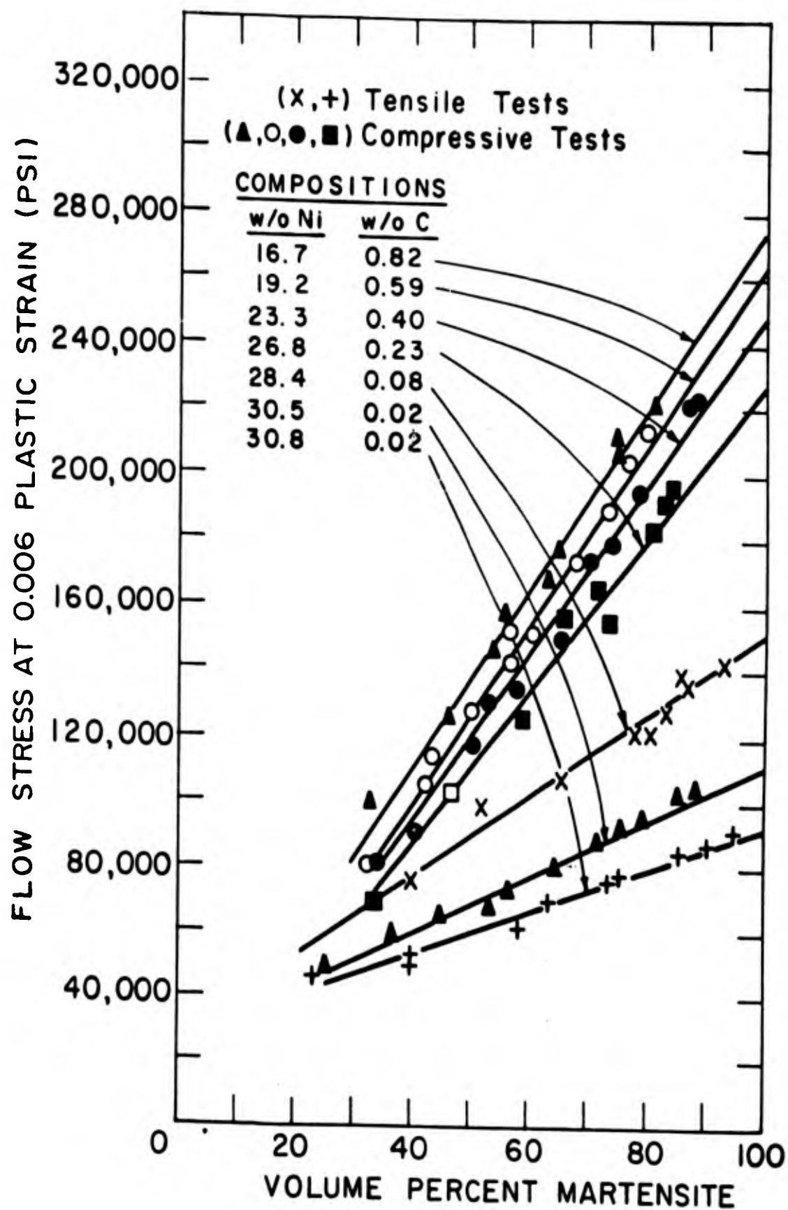
Fig. 5 Flow Stress (at 0.006 Plastic Strain) of Martensite - Austenite Mixtures after Aging 3 Hours at 0°C. Tested at 0°C.
