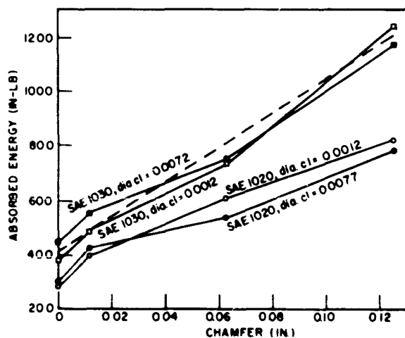
Fig. 11 - Absorbed energy versus chamfer size. The dotted lines represent a linear approximation and average for each specimen material.
