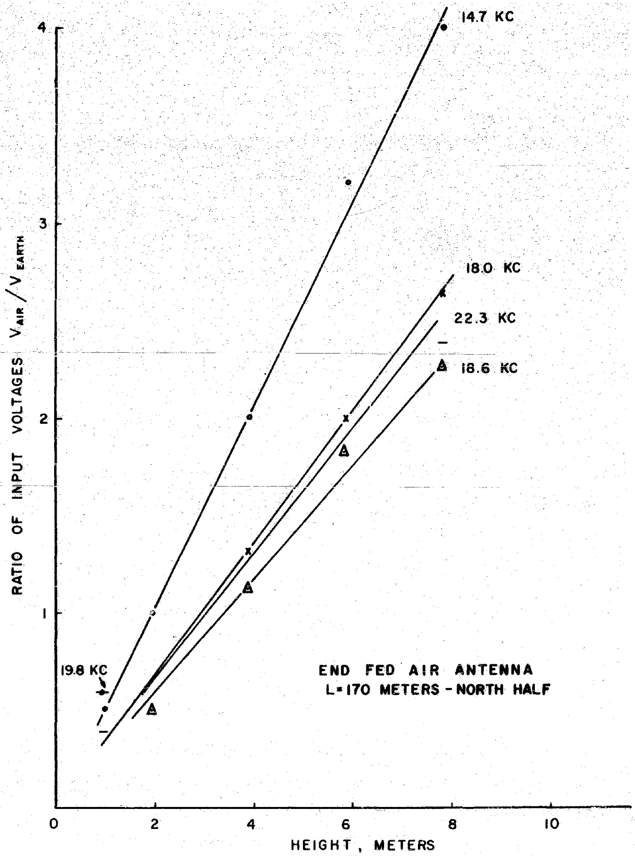
RATIO AIR ANTENNA SIGNAL TO EARTH PROBE SIGNAL FIG. 3.
