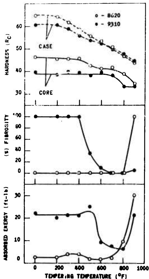
Figure 4. EFFECT OF TEMPERING TEMPERATURE ON HARDNESS AND V-NOTCH CHARPY IMPACT PROPERTIES AT -40 ° - CARBURIZED SAE 9310 AND 8620 STEELS
