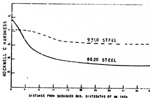
SAE C Mn Si Ni Cr Mo Austenizing Temp. F 9310 0.11 0.60 0.32 3.21 1.24 0.11 1650 8620 0.20 0.83 0.31 0.50 0.52 0.22 1575 Figure 1. END QUENCH HARDENABILITY CURVES OF SAE 9310 AND 8620 STEELS
