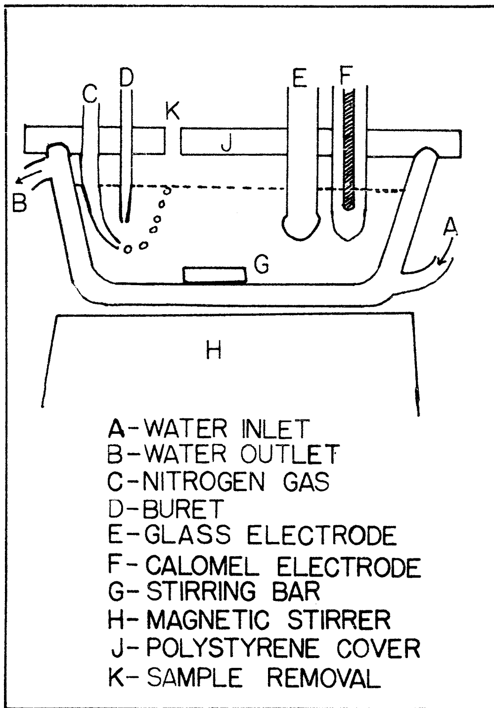
Figure 3 Reaction Assembly
