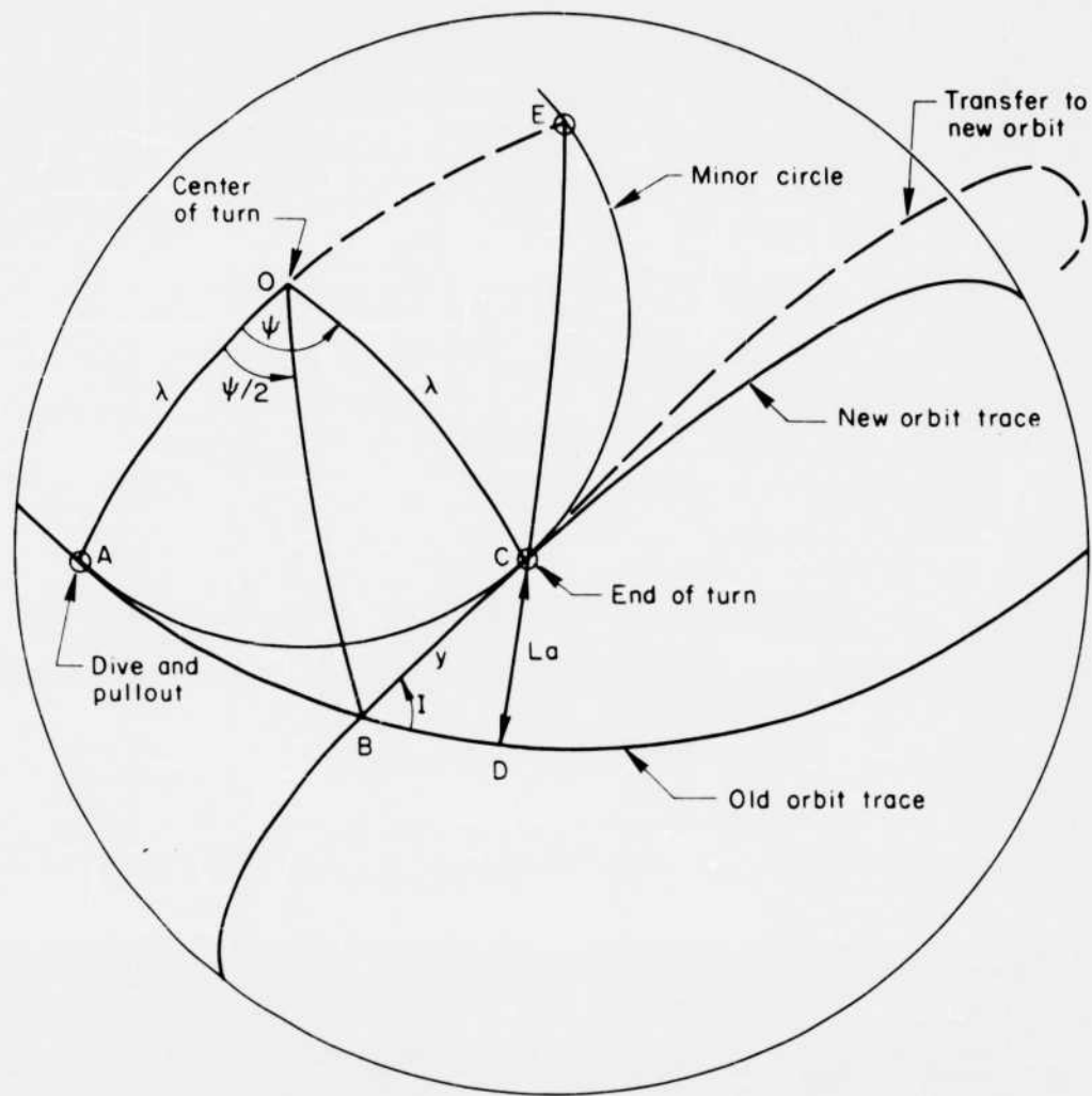
Fig. 10—Minor circle turn geometry
