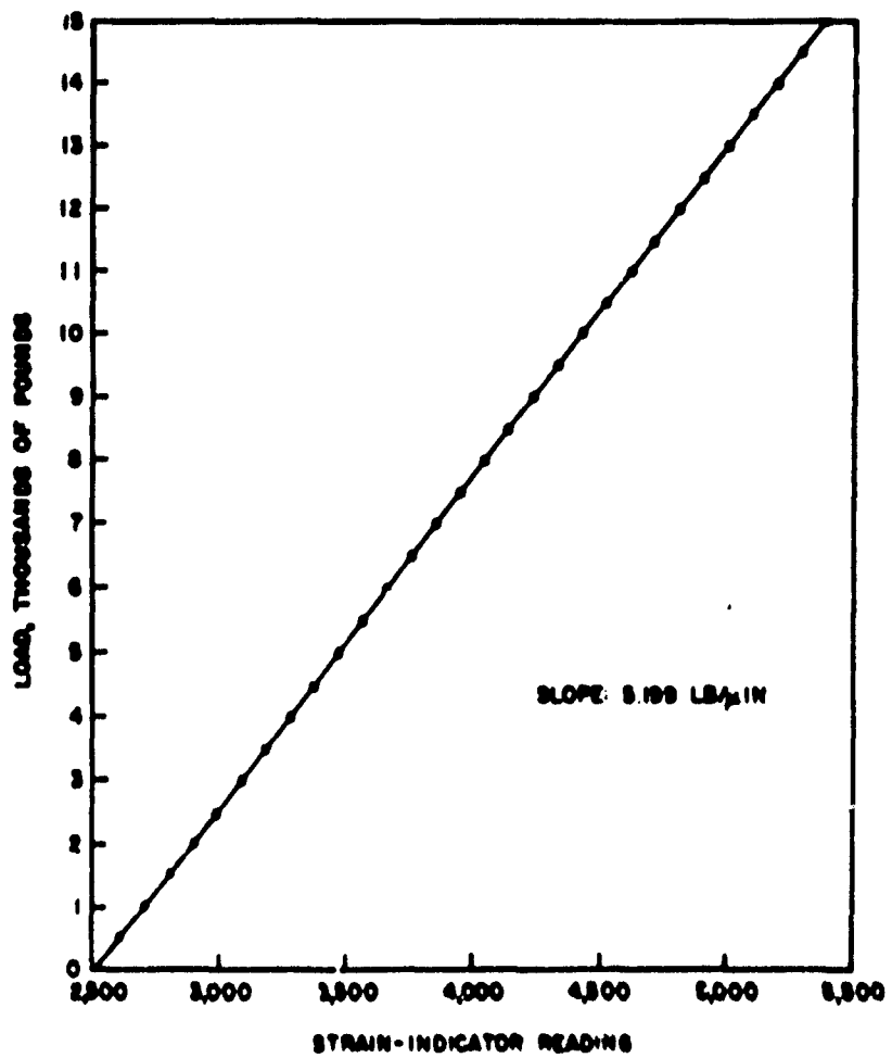
FIG. 13. Load Versus Strain-Indicator Reading for Bottom Flexure 3, Under Tension, No offset.
