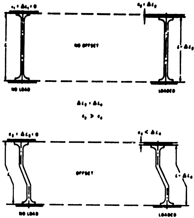
FIG. 8. Flexure-Cell Configuration With and Without Load and Offset. \epsilon Is the Measured Deflection Between Flange Faces.
