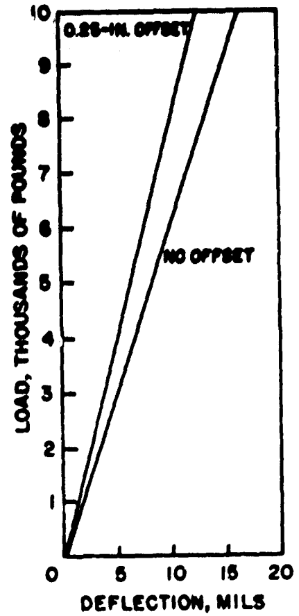
FIG. 7. Applied Load Versus Vertical Deflection Between Flange Faces of 0.60-Inch-Diameter Flexure-Cell.
