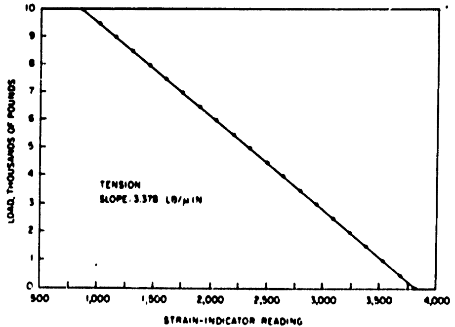
FIG. 9. Load Versus Strain-Indicator Reading for Side Flexure 1, No offset.
