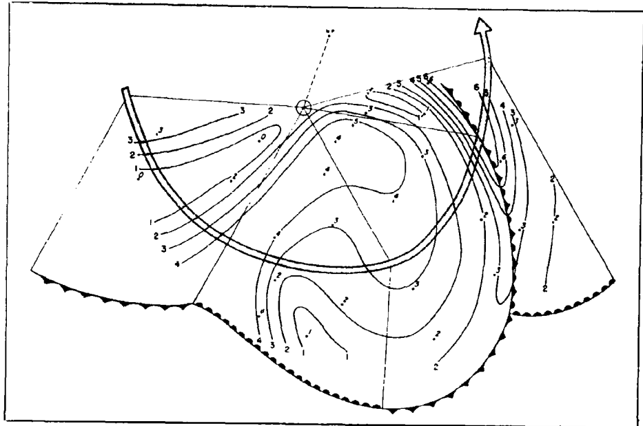
Figure 3.9. Composite Chart of Cloud Distribution in a Layer from 5,000 to 10,000 Feet. Mean Cloud Amounts in Oktas (Eights of Sky Covered) Are Plotted at Points of Averaging. Circle Denotes Low Center at 500-mb.; Arrow Denotes the Jet Axis at that level.
