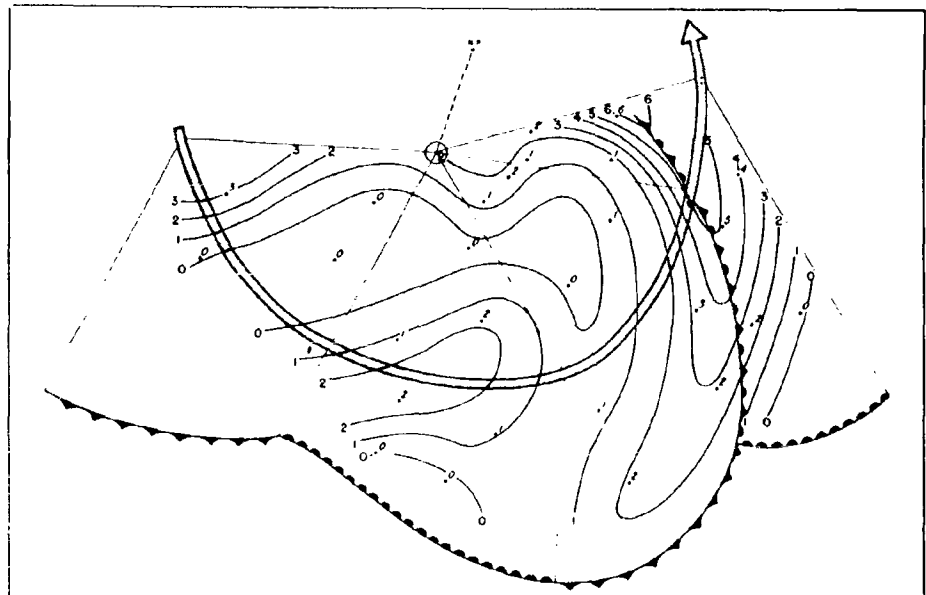
Figure 3.10. Composite Chart of Cloud Distribution in a Layer from 15,000 to 20,000 Feet. Mean Cloud Amounts in Oktas (Eights of Sky Covered) Are Plotted at Points of Averaging. Circle Denotes Low Center at 500-mb.; Arrow Denotes the Jet Axis at that level.
