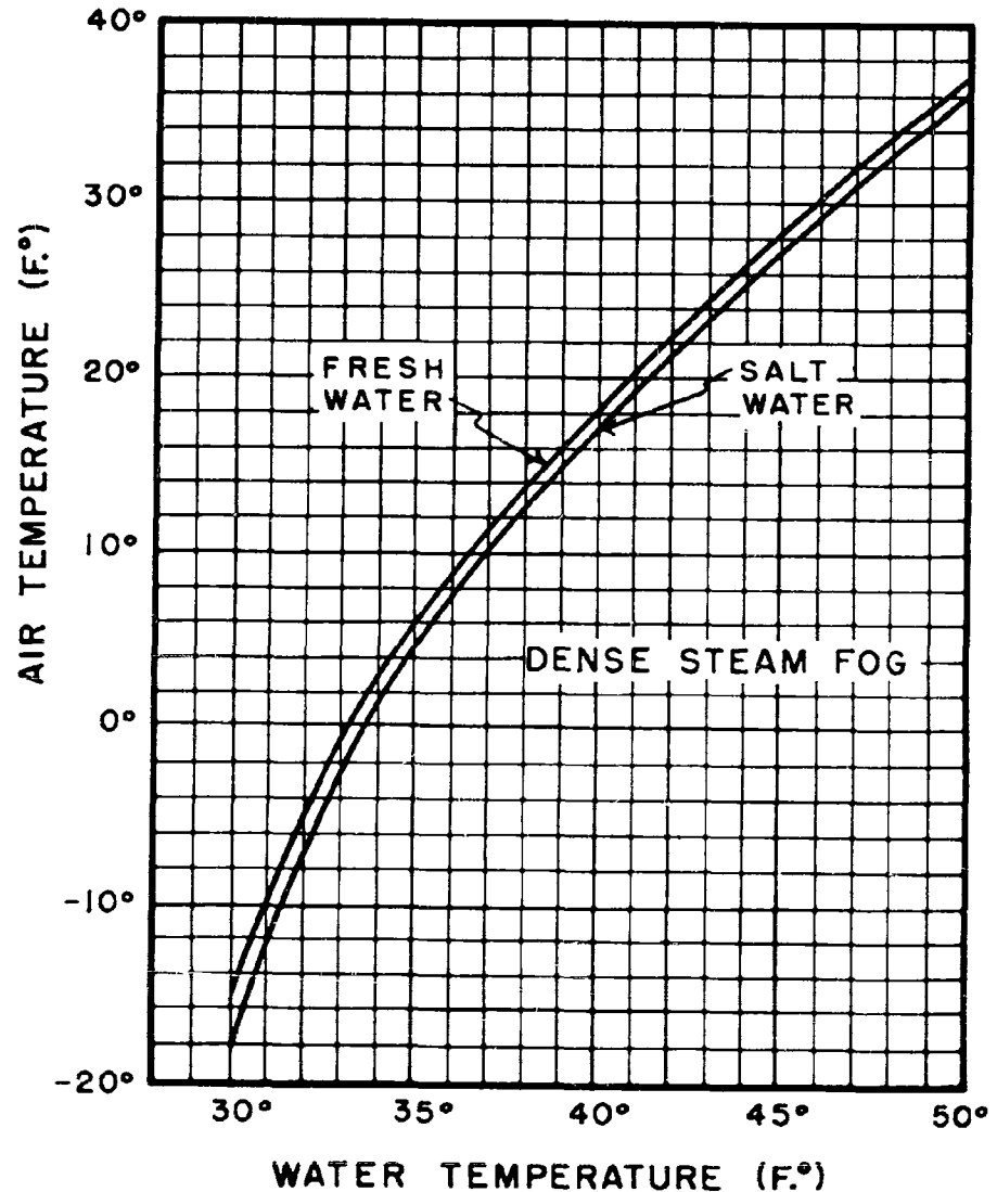
Figure 5.11. Graph for Prediction of Dense Steam Fog.
