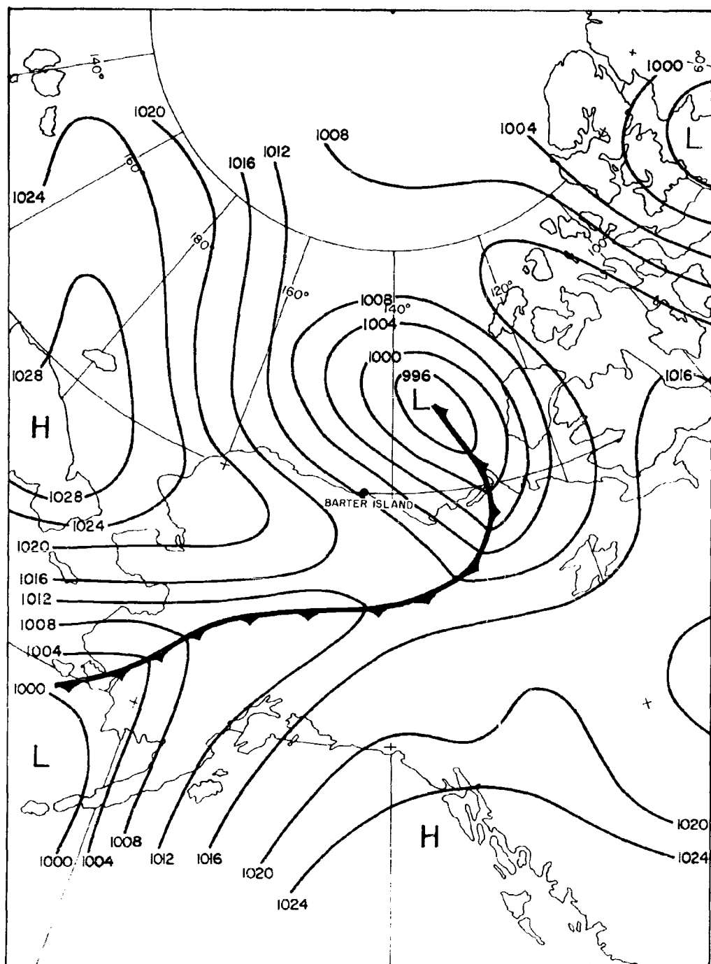
Figure 5.8. Surface Chart for 0630 G.M.T., 4 January 1957.
