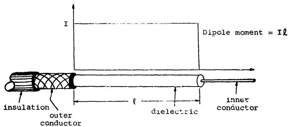
(a) Short-circuited dipole
