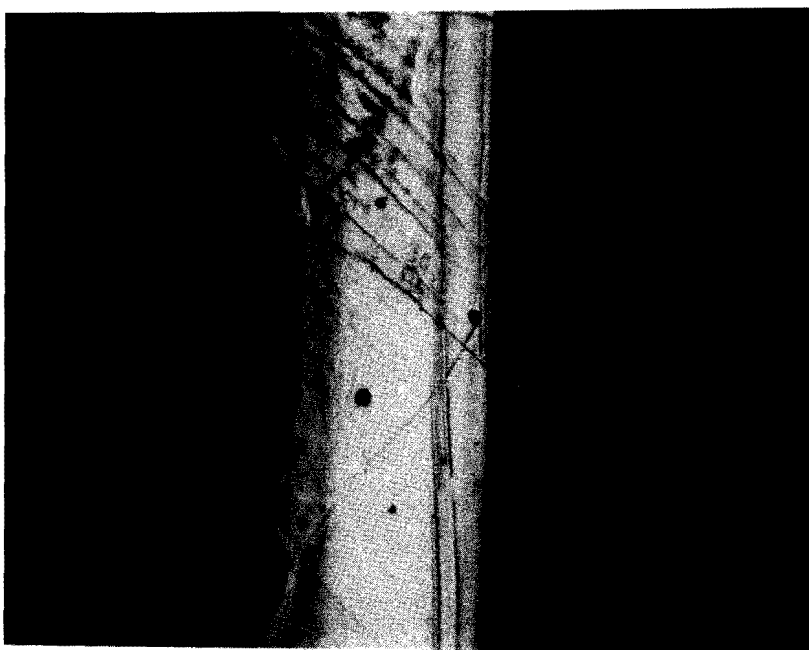
Figure 18. Nature of Slip Lines in Platinum as they Cross a Grain Boundary 375X
