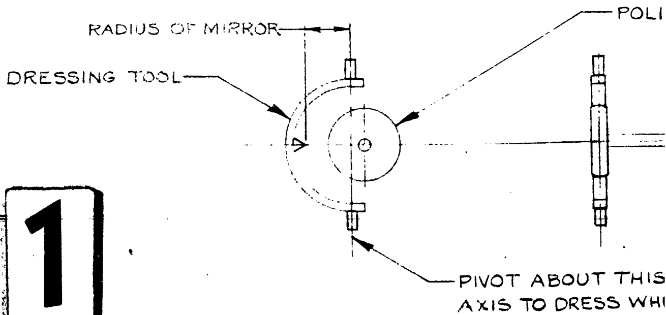
WHEEL DRESSING SET-UP
