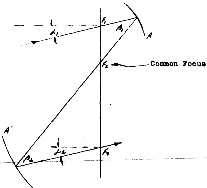
Basic Mirror Configuration - Inside Surfaces
