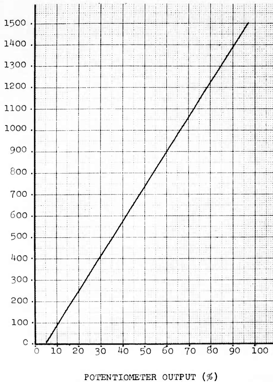
FIGURE 30 CALIBRATION CURVES FOR THE 0 TO 1500 PSIG GIANNINI PRESSURE TRANSDUCER MODEL 46119Y
