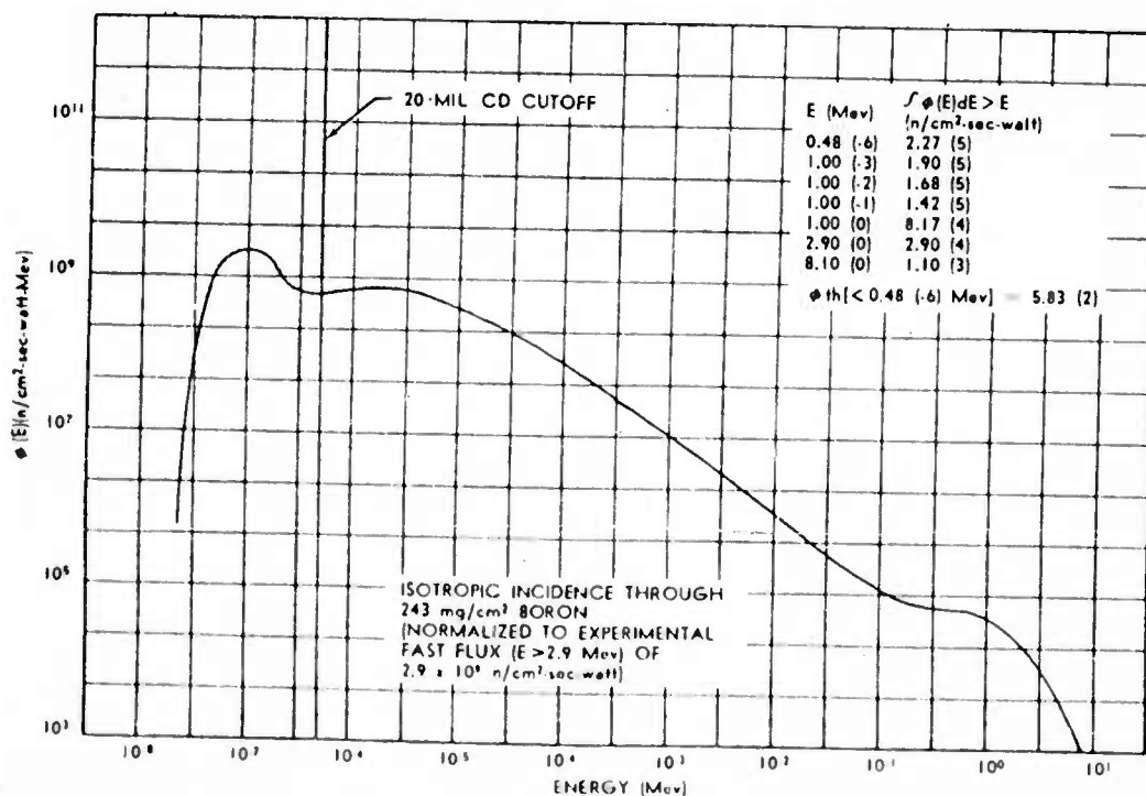
ANALYTIC GTR SPECTRA, BORAL ATTENUATED
