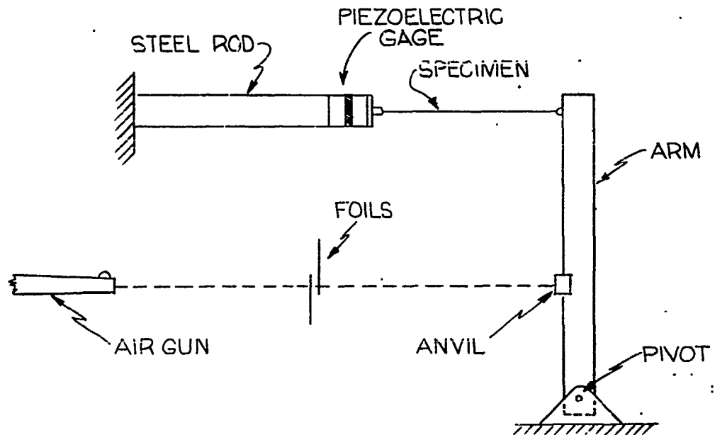
Fig. 3.27. Schematic diagram of ballistic apparatus used by Holden for impact tests on monofils and yarns [31].
