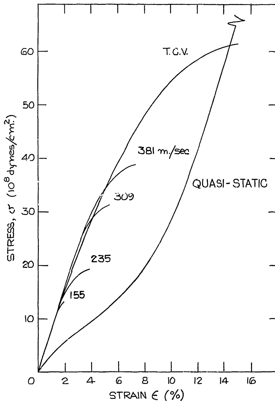
Fig. 4.12. Stress-strain curves of 210/5 nylon 66 yarn, in quasi-static test and for various transverse impact velocities [after Ref. 67].
