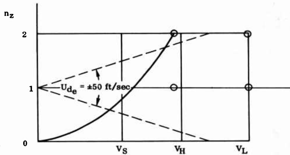
Figure 9.5 V-n_z Diagram
