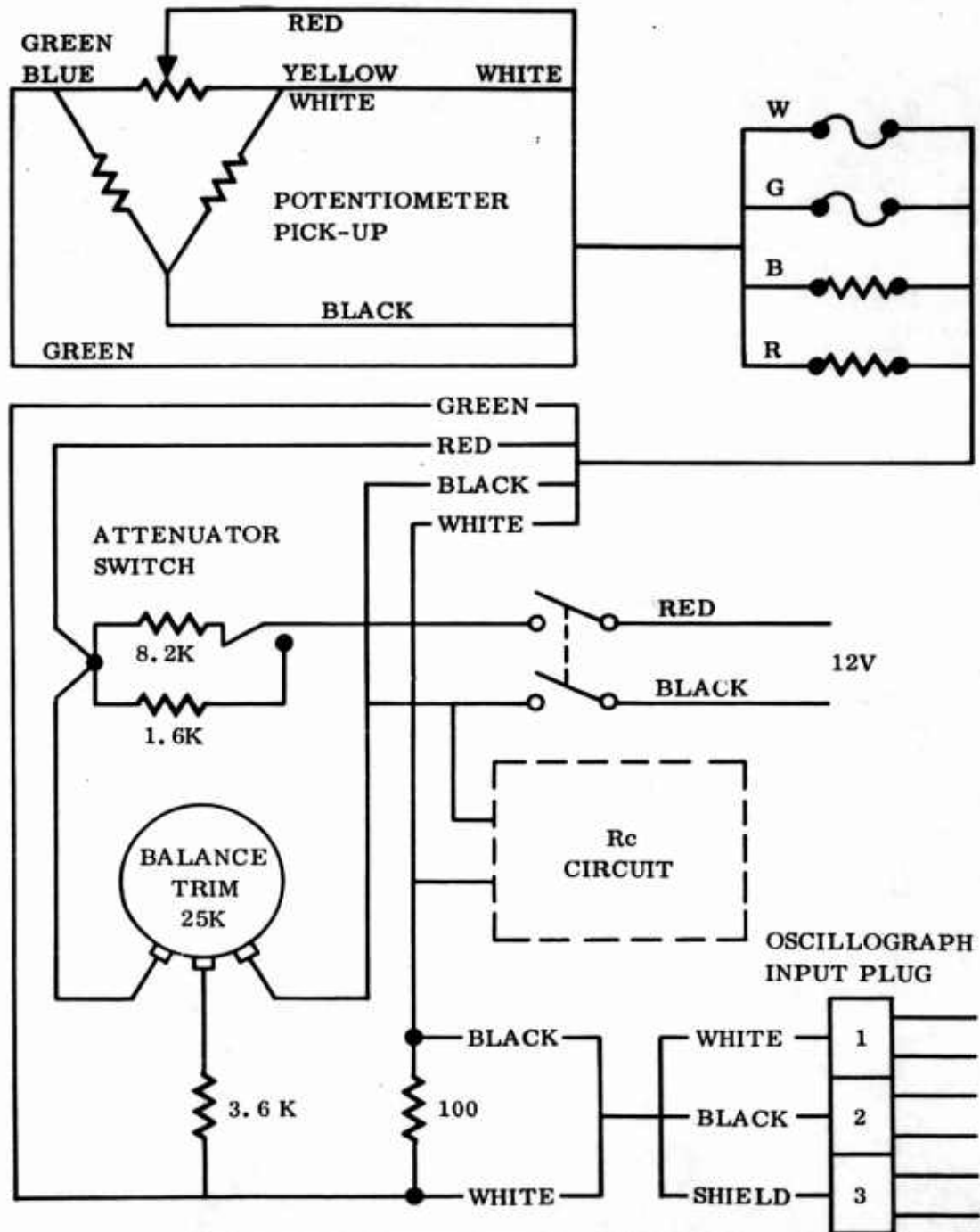
Figure 10.3 Typical Potentiometer Circuit
