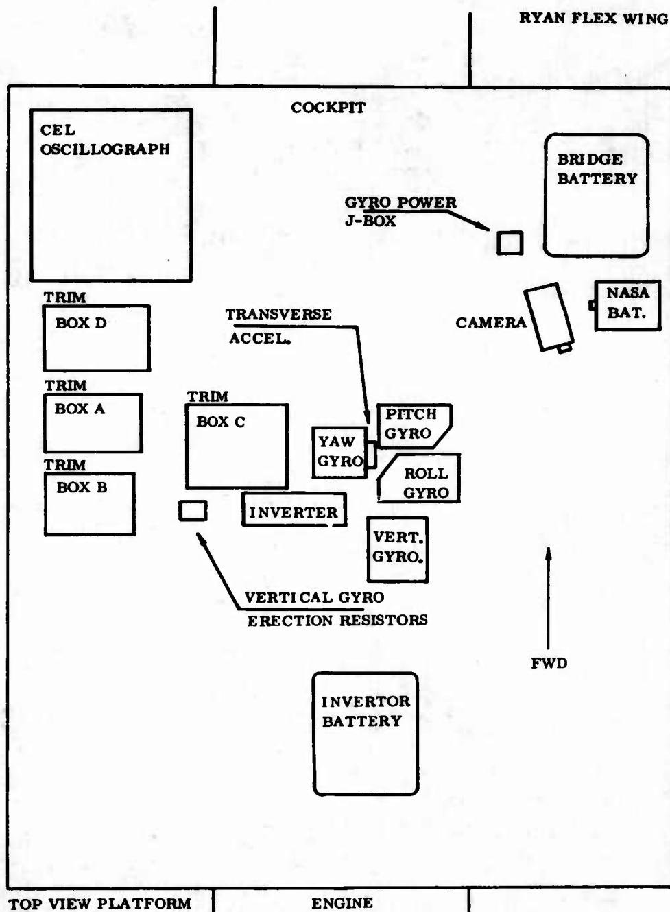
Figure 10.2 Instrumentation Layout
