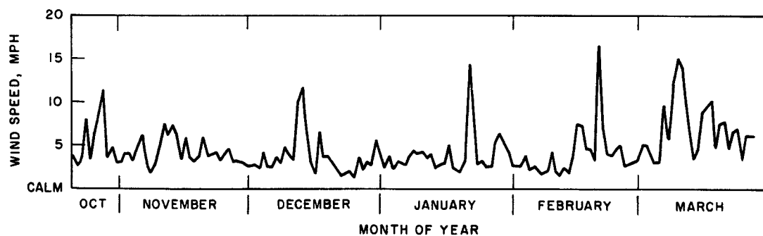
FIG. 47. Average Daily Wind Speed at Fairbanks During Winter 1961-62.
