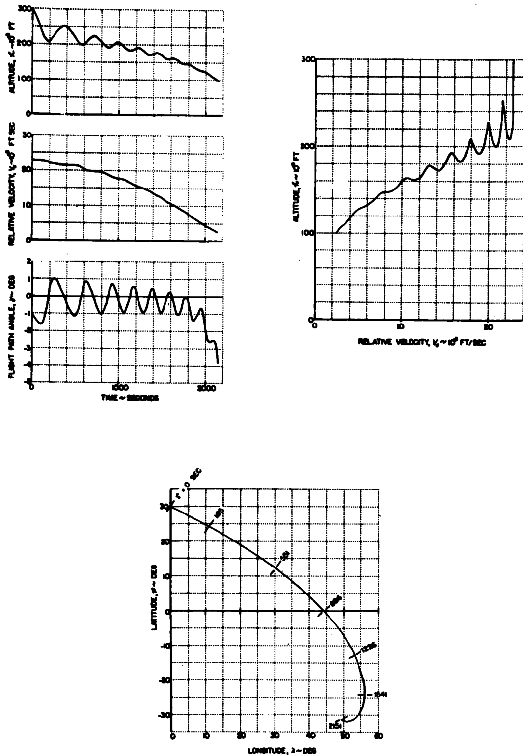
FIGURE 5.5 TURNING RE-ENTRY SOLUTION - CASE III
