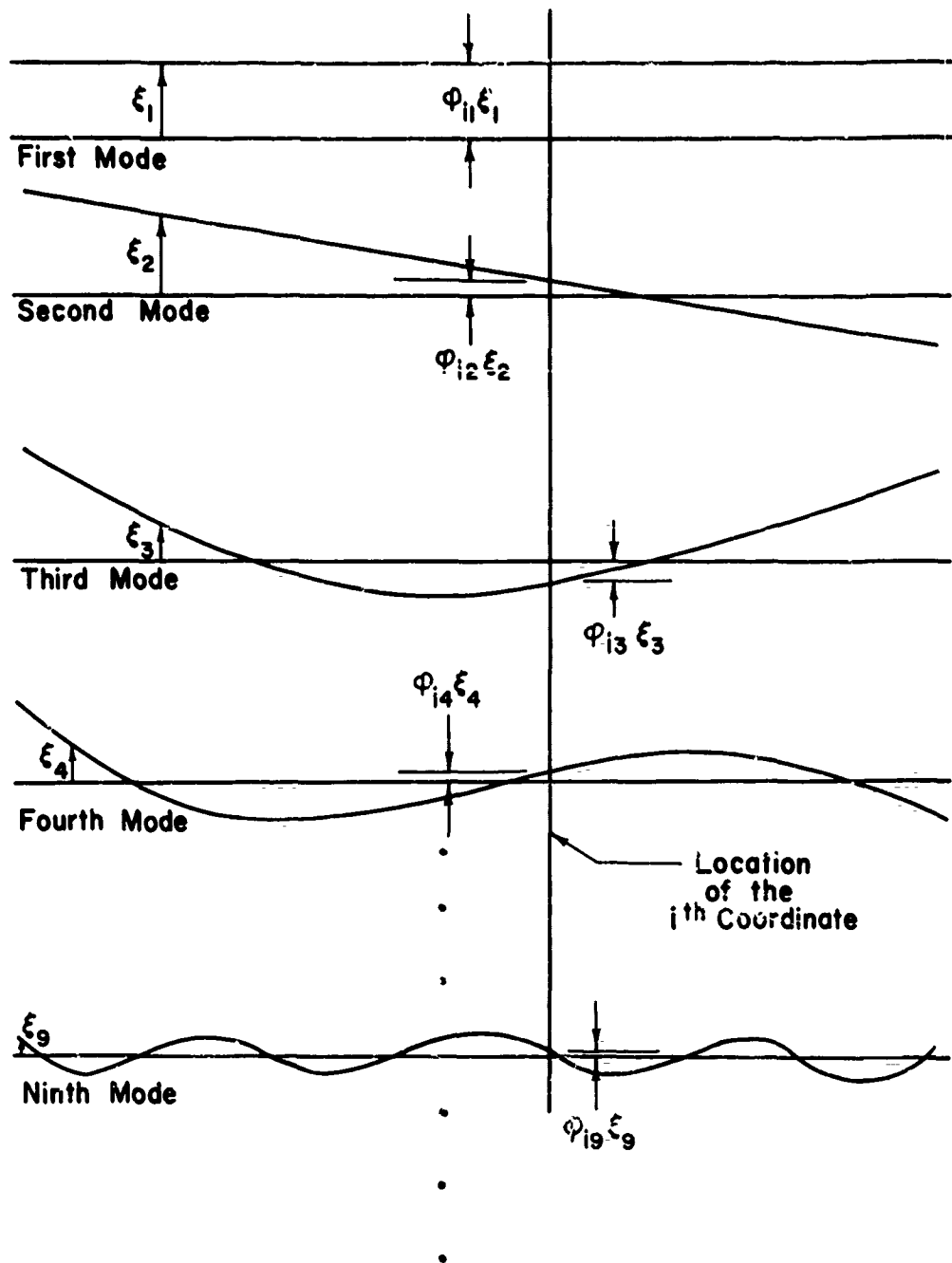
Figure 2. Mode Displacement Curves; q_i = \sum_{j=1}^n \phi_{ij} \xi_j
